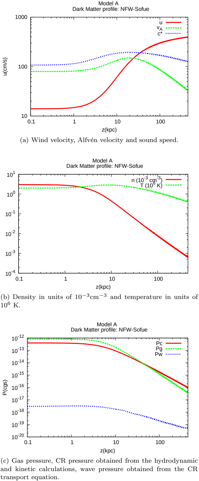
Figure 6. Results for Model-A: at the wind base, z_0 , the gas density is n_0 = 3 \times 10^{-3} \text{cm}^{-3} and the magnetic field is B_0 = 2 \mu\text{G} . The CR injection spectrum has been normalized in order to get the observed CR pressure P_{c0} = 4 \times 10^{-13} \text{erg/cm}^3 at z_0 .
