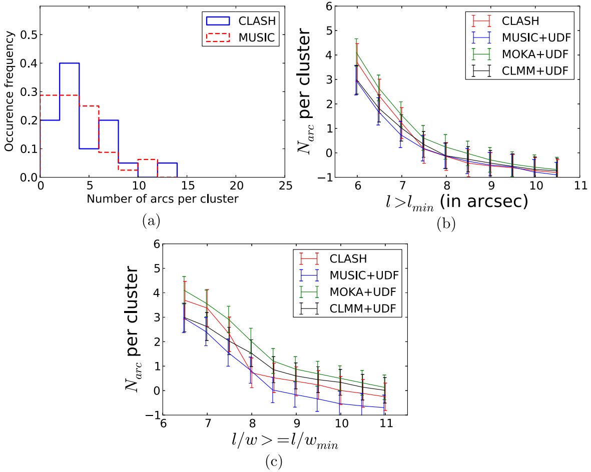
Figure 18. (a) Comparison of the number distribution between the CLASH sample and MUSIC sample. (b) Lensing efficiency as a function of l_{\text{min}} for arcs with l/w \geq 7 for different samples. (c) Lensing efficiency as a function of l/w_{\text{min}} for arcs with l \geq 6'' for different samples.
