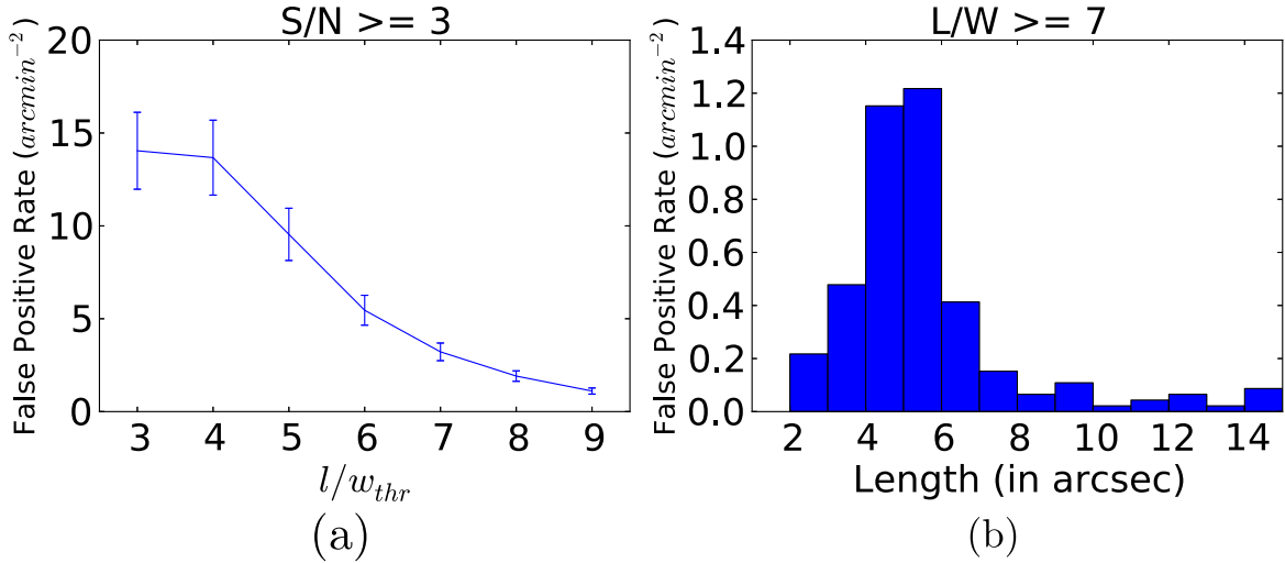
Figure 5. (a) False positive rate per unit area as a function of the detected l/w threshold for arcs with S/N \geq 3 . (b) False positive rate per unit area as a function of the arc length for arcs with l/w \geq 7 . Results are based on running the arc finder on CANDELS data. The error bars denote the 1\sigma rms error.
