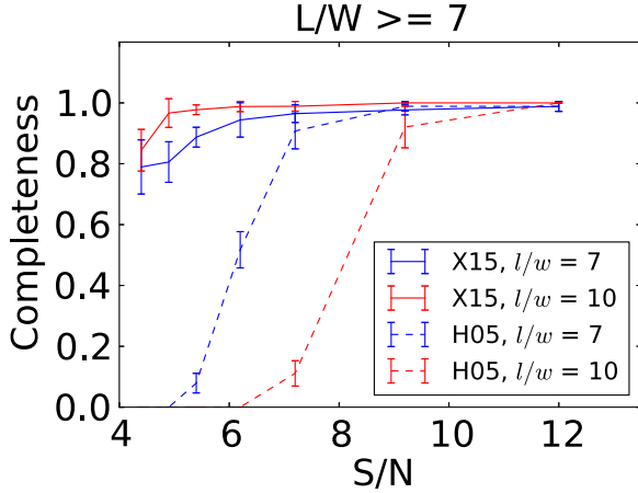
Figure 9. Comparison of the arc detection completeness between our arc finder (solid curves) and the Hoeshe et al. (2005) arc finder (dashed curves) for arcs with l/w = 7, 10 . The error bars denote the scatter. For bright arcs with S/N > 10 both arc finders maintain a high detection rate (>90%), while for faint arcs with lower S/N levels, our arc finder exhibits considerably higher detection efficiency. The error bar denotes the 1\sigma rms error.
