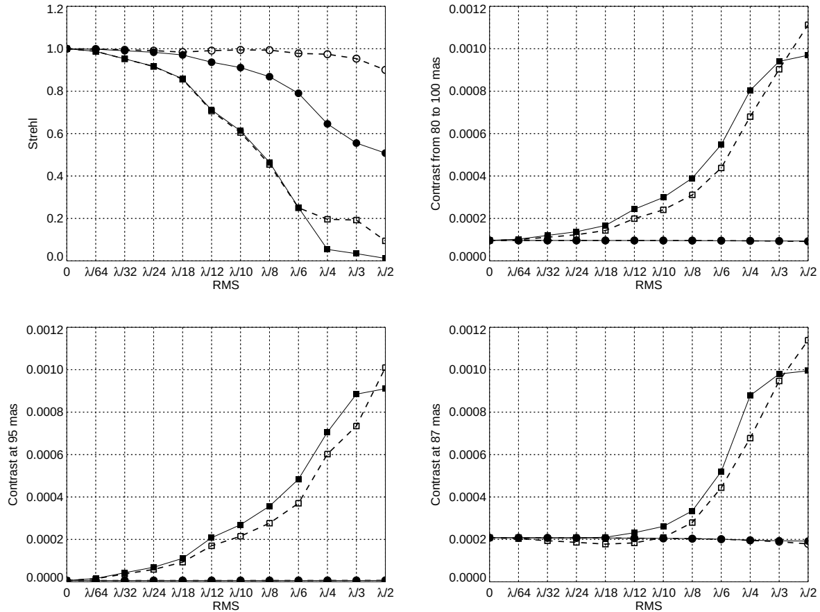
Figure 6. Merit functions for the PSF : Interferometric Strehl (top left), averaged contrast from 80 mas to 100 mas (top right), contrast at 95 mas located in a local minima (bottom left), contrast at 87 mas located in a local maxima (bottom right). AO wavefront errors (square symbol) or piston errors (circular symbol) for various RMS values. Short exposure (empty symbol, dashed line) and long exposure (filled symbol, solid line).
