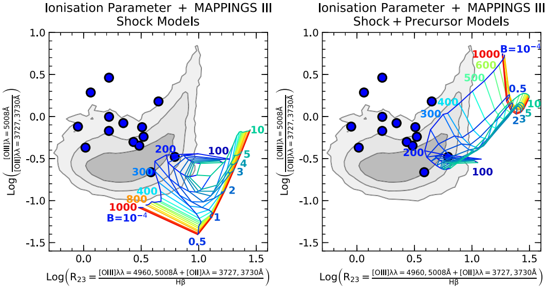
Figure A4. R_{23} versus [O III]/[O II] diagram showing the median location of the outflowing gas in each of the galaxies in our sample, as Fig. 7, but also showing the result of a grid shock models with varying velocities, from 100 \text{ km s}^{-1} (blue) to 1000 \text{ km s}^{-1} (red), and varying magnetic field parameter, from B/n^{1/2} = 10^{-4} \mu\text{G cm}^{3/2} (dark blue) to B/n^{1/2} = 10 \mu\text{G cm}^{3/2} (light blue), both without (left) and with (right) shock precursor. Most outflows classified as star forming cannot be explained in terms of shock.
