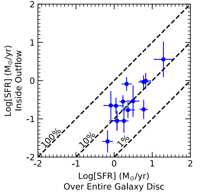
Figure 8. SFR inside the outflow as a function of total SFR in the disc of the host galaxy.
