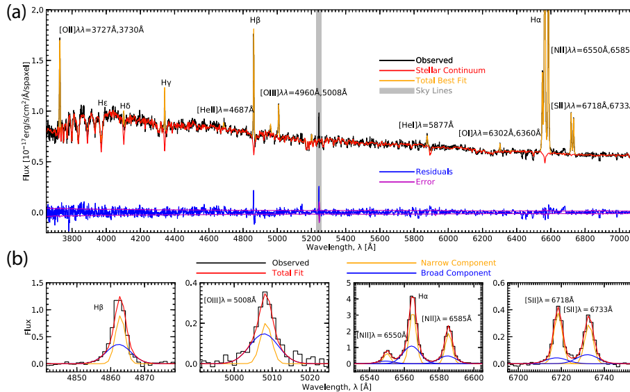
Figure 1. Example of simultaneous stellar continuum and emission-line fit to the spectrum extracted from the central region of a representative galaxy in our sample. (a) Full spectrum decomposition showing the simultaneous stellar continuum (red) and emission-line (orange) fit to spectrum. Shown below the fit are the residuals (blue) and the error spectrum (magenta) for the galaxy. The O II 5577 sky line has been masked, shown here by the grey shaded area. (b) Subsections of continuum-subtracted spectra, showing some of the relevant emission lines used in the analyses. The decomposition of the narrow (orange) and broad (blue) components can be seen, alongside the total fit of the two components (red).
