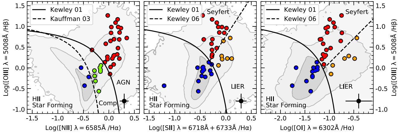
Figure 5. Median BPT classification of the outflows for the galaxies in our sample. According to their median BPT classification in the [S II] and [O I] diagrams (central and right panels), about 30 per cent of the galactic outflows in our sample are ‘star forming’. The same applies to the [N II] classification if one includes galaxies classified as ‘composite’ (however, one should take into account that the [N II] classification is more ambiguous, as discussed in the text).
