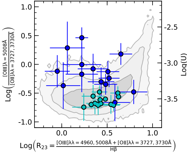
Figure 7. Ionization parameter (right-hand Y-axis) as traced by the [\text{O III}]/[\text{O II}] ratio (left-hand Y-axis) as a function of the R_{23} parameter, which is primarily sensitive to the gas metallicity. Dark blue symbols indicate the median values observed in those galactic outflows dominated by star formation, according to the [\text{S II}] -BPT diagnostic diagram, as in Fig. 5. The light blue symbols are the average location of the narrow component in regions that are classified as star forming. The shaded contours indicate the distribution of star-forming galaxies from the SDSS survey (68 per cent, 95 per cent, and 99.7 per cent of the population). Star-forming outflows (blue symbols) have similar ionization parameter as normal star-forming regions, and possibly even slightly higher. The error bars shown are the median error of the ratios calculated for all spaxels within the outflow.
