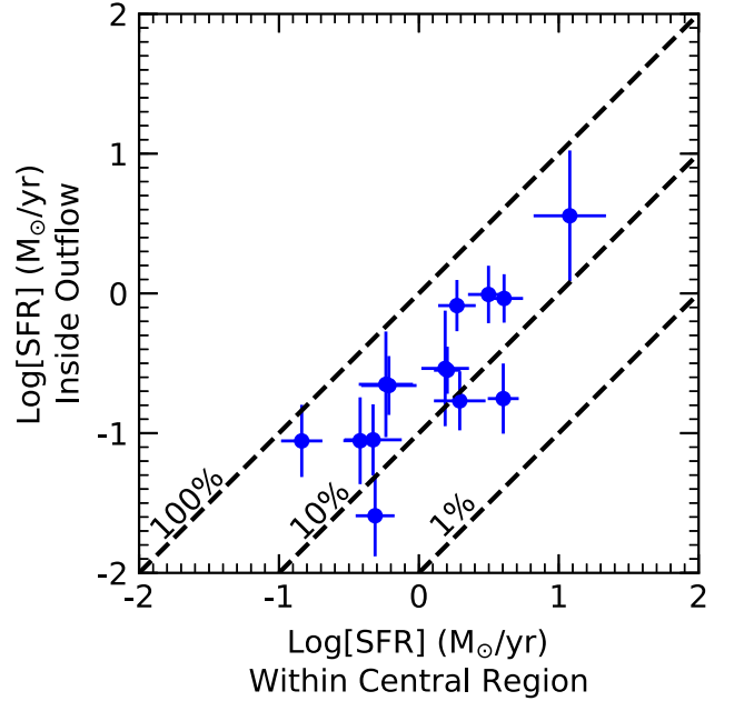
Figure 9. SFR inside the outflow as a function of the SFR in the same central projected area in which the outflow is detected.
