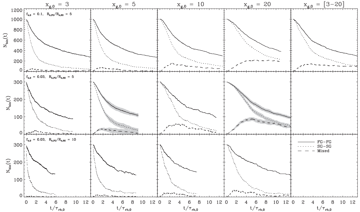
Figure 4. Time evolution of the total number of FG (solid lines), SG (dotted lines) and mixed (dashed lines) binaries for all the MPr5f1 (first row), MPr5f03 (second row) and MPr10f03 (third row) simulations. Each column shows the results of simulations for a different value of x_{g,0} indicated at the top of the figure. For simulations MPr5f03x5 and MPr5f03x20 the lines show the mean of the number of binaries from the results of the 10 simulations with different random realizations of the initial conditions and the shaded area show the \pm 1\sigma . Time is normalized to the initial half-mass relaxation time.
