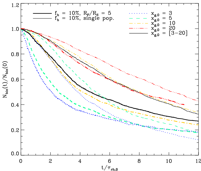
Figure 1. Time evolution of the total number of binaries, N_{\text{bin}}(t) (normalized to the total initial number of binaries, N_{\text{bin}}(0) ), for simulations MPPr5f1 and SPf1 and different values of the hardness factor x_{g,0} . Time is normalized to the initial half-mass relaxation time, \tau_{\text{rh},0} .
