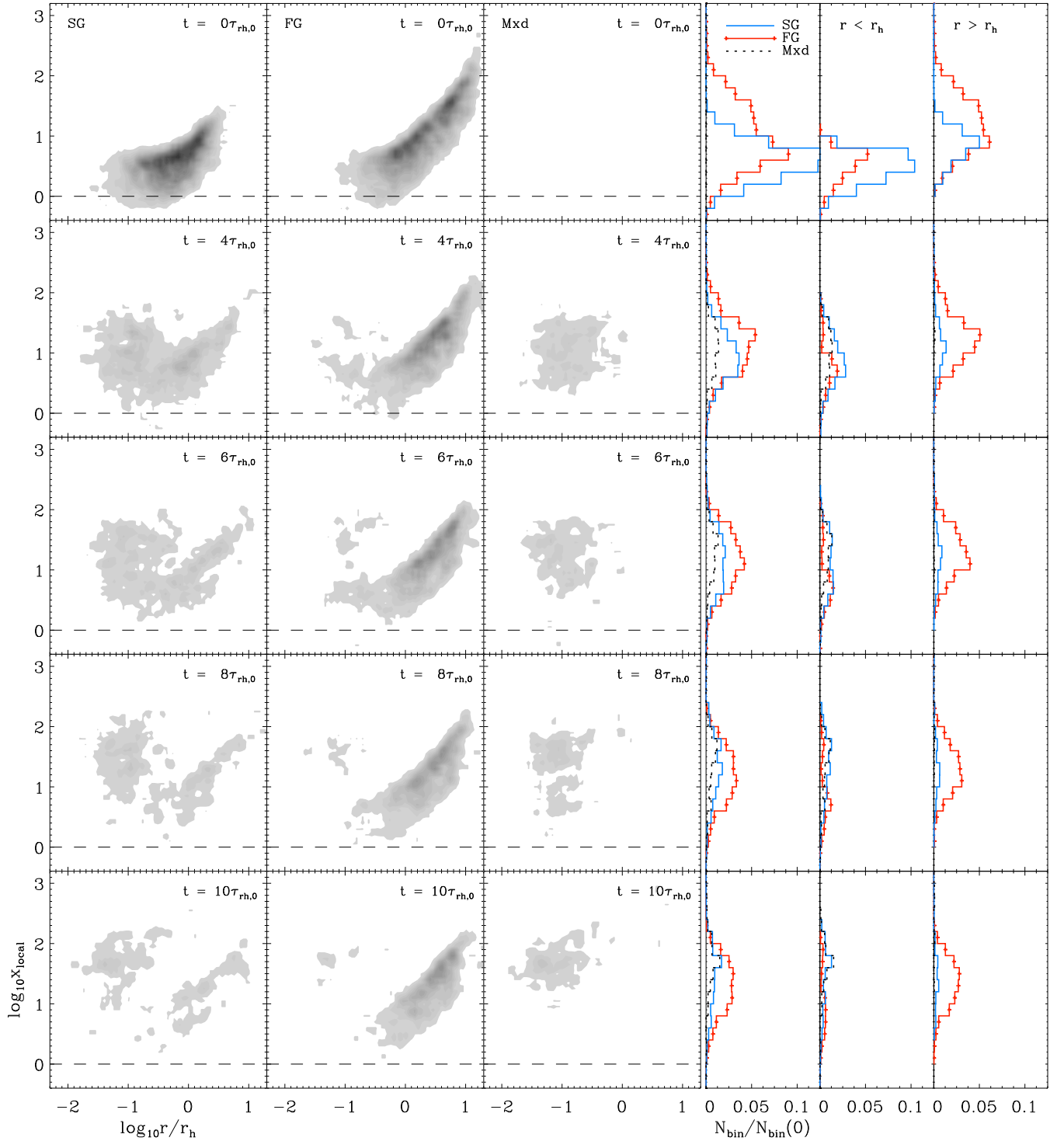
Figure 7. Time evolution of the density of SG (first column), FG (second column) and mixed (third column) binaries in the \log(r/r_h) – \log(x_{\text{local}}(r)) plane (where x_{\text{local}}(r) is the local hardness parameter; see Section 3.1 for definition) for the MPr5f1x3-20 simulation. The last three columns of panels (on the right-hand side of the figure) show the histograms of the distribution of \log(x_{\text{local}}(r)) for SG (solid blue lines), FG (red lines and short vertical segments) and mixed binaries (dashed lines) for the whole system, for binaries within the half-mass radius and outside the half-mass radius. Data from three combined snapshots around the indicated time are used for these plots.
