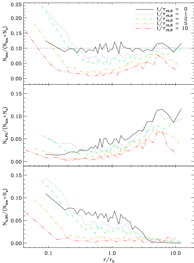
Figure 10. Time evolution of the radial profile of the binary fraction for the model MPPr5f1x3-20 for all binaries (top panel), FG binaries (middle panel) and SG binaries (lower panel). Different lines in each panel correspond to the times indicated in the legend in the top panel. The radial profiles have been calculated with data from three combined snapshots around the indicated time.
