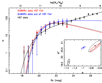
Fig. 2 LFs of galaxies in MACS J1206.2-0847, from HST data (black) and from SUBARU data in the same region covered by HST (red) and in the external region (blue). Continuous lines are the fits with the Schechter function. Dashed line is the fit to HST data down to M=M^*+3 . The best-fit Schechter parameters for \alpha and M^* with their 1\sigma contours for the corresponding LFs are also reported in the small panel.
