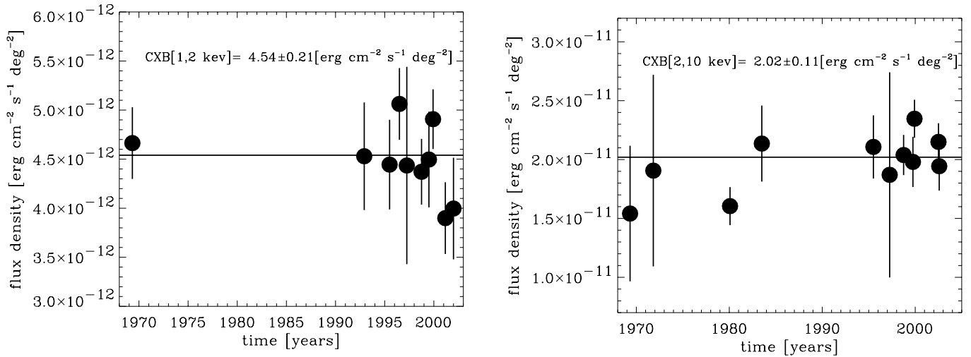
FIG. 3.— Left panel: Soft CXB (1–2 keV) measurements spaced in time along with their 68% error bars. Solid line: Best fit to all these measurements ( \chi^2_{\text{red}} = 0.9 ). CXB values ( left to right ) are from Gorenstein, Kellogg, & Gursky (1969); Garmire et al. (1992); Gendreau et al. (1995); Georgantopoulos et al. (1996); Chen, Fabian, & Gendreau (1997); Miyaji et al. (1998); Parmar et al. (1999); Vecchi et al. (1999); Kuntz, Snowden, Mushotzky (2001); Lumb et al. (2002). Right panel: Hard CXB (2–10 keV) measurements spaced in time along with their 68% error bars. Solid line: Best fit to all these measurements ( \chi^2_{\text{red}} = 1.3 ). CXB values ( left to right ) are from Gorenstein, Kellogg, & Gursky (1969); Palmieri et al. (1971); Marshall et al. (1980); McCammon et al. (1983); Gendreau et al. (1995); Chen et al. (1997); Miyaji et al. (1998); Ueda et al. (1999); Vecchi et al. (1999); Lumb et al. (2002); Kushino et al. (2002).
