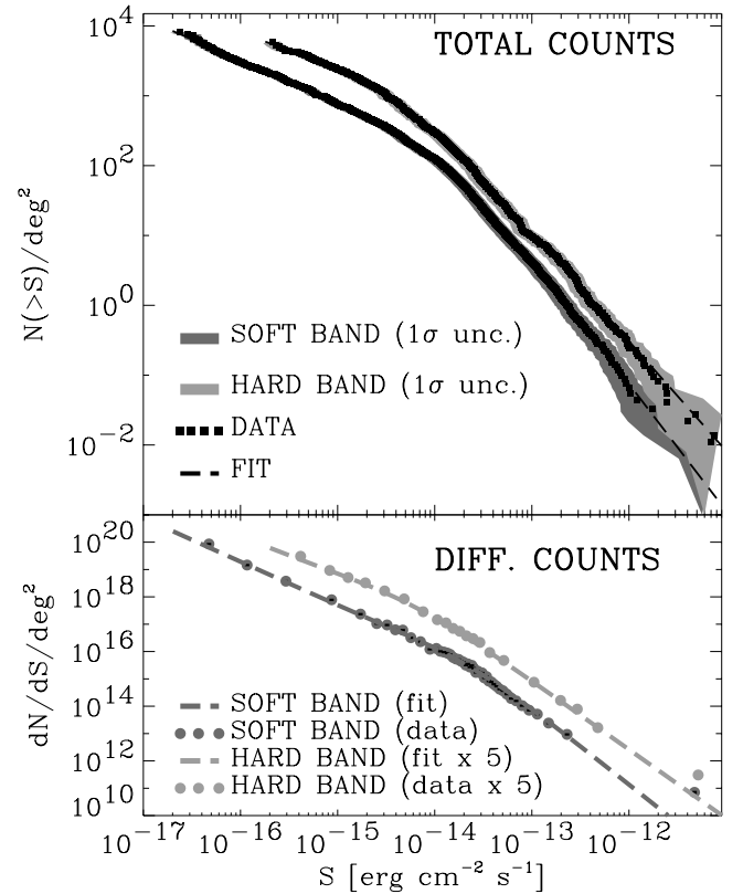
FIG. 4.— Upper panel : log N -log S (integral) curves of our composite catalog in both soft and hard band; in both cases we obtained an excellent fit with two smoothly joined power laws (see text). Lower panel : Plot of the differential distributions: the data are grouped to have a minimum of 100 (50) measures in each bin in the soft (hard) band. The hard band counts are multiplied by 5 for clarity of the plot. Because of the very large y -axis range the error bars are not visible in the graph: they are approximately 10% and 15%, respectively.
