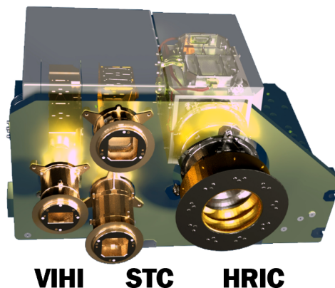
Figure 1: SIMBIOSYS three channels
