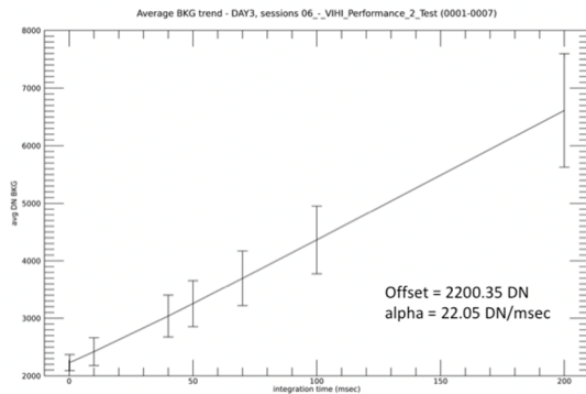
Figure 13: Trend of the background signal (left side) and of the dark signal (right side) with respect to the integration times (i.e., 0.2, 10, 40, 50, 70, 100, 200 ms) and FPA temperature 215K, Spectrometer temperature 225K, PE Temperature 284-286K.
