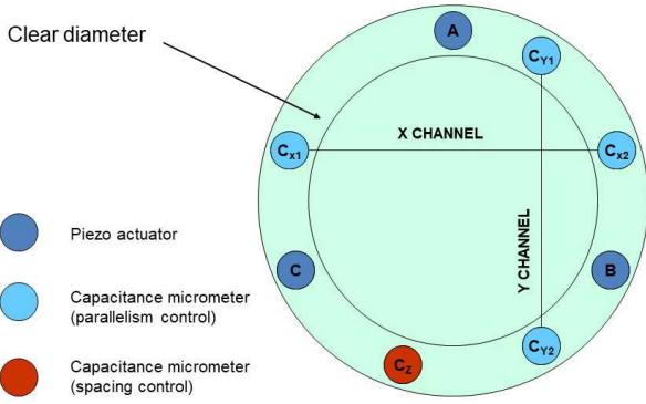
Fig. 11. Scheme of the piezo-electric actuators and the capacitance controls for separation and parallelism of the ET50' plates.
