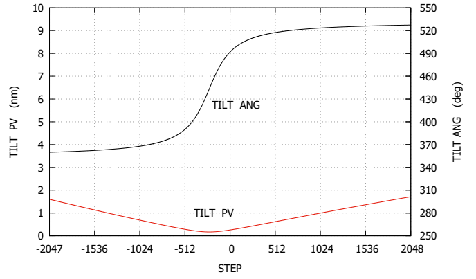
Fig. A.4. As Fig. A.3 for the 2.8 mm gap ET50 of NSO (Fig. A.2).
