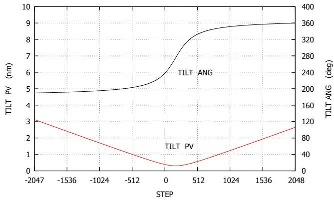
Fig. A.3. PV and angle of the tilt component of the cavity error maps of the 609 \mu\text{m} gap NSO ET50 (Fig. A.1).
