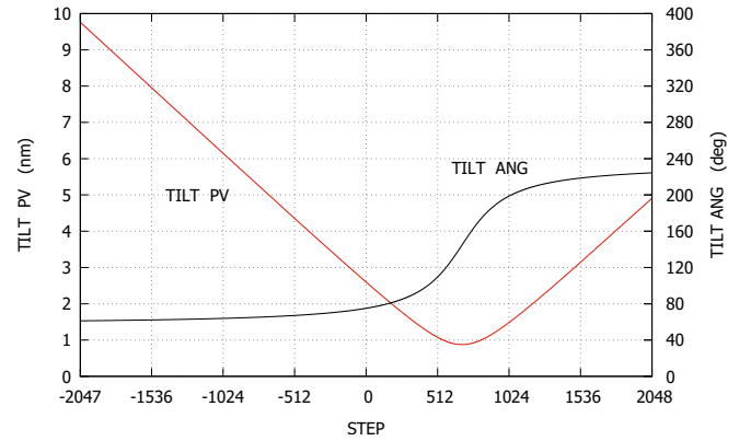
Fig. 7. PV and angle of the tilt component of the cavities of Fig. 6 (TILT PV and TILT ANG, respectively), along the full spectral scan. The curves represent the actual values of the parameters derived from the planar fit; both vary very smoothly with n . Any local variation of the parameters is contained within the thickness of the font.
