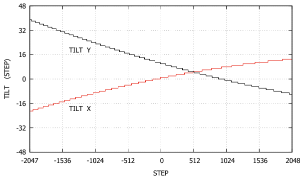
Fig. 12. Lookup table of the (TILTX, TILTY) corrections adopted to minimize the cavity tilt introduced by the scan. Each tilt step corresponds to 1.4 \times 10^{-3} arcsec.
