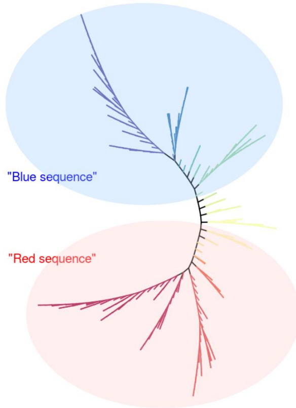
Figure 6. The phylogenetic tree for the galaxies of the WINGS survey. Colors mark the different groups defined by the cladistic analysis on a set of parameters which includes color index, absolute magnitude, effective radius, sersic index, among others. From Fraix-Burnet et al. (2017).
