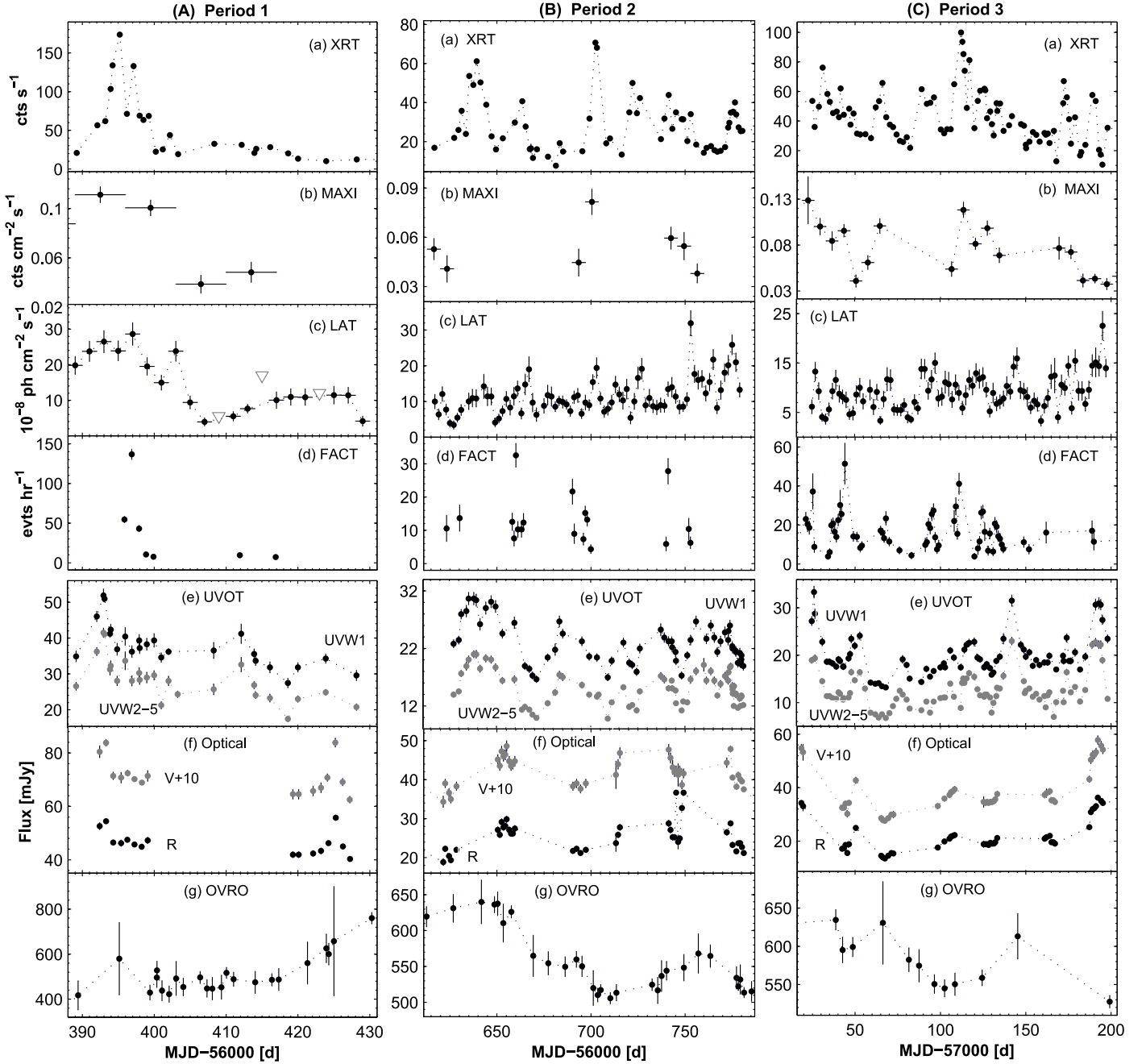
Figure 2. MWL light curves of Mrk 421 in different periods (with the same time bins, except for the LAT data binned within 2-day intervals).
