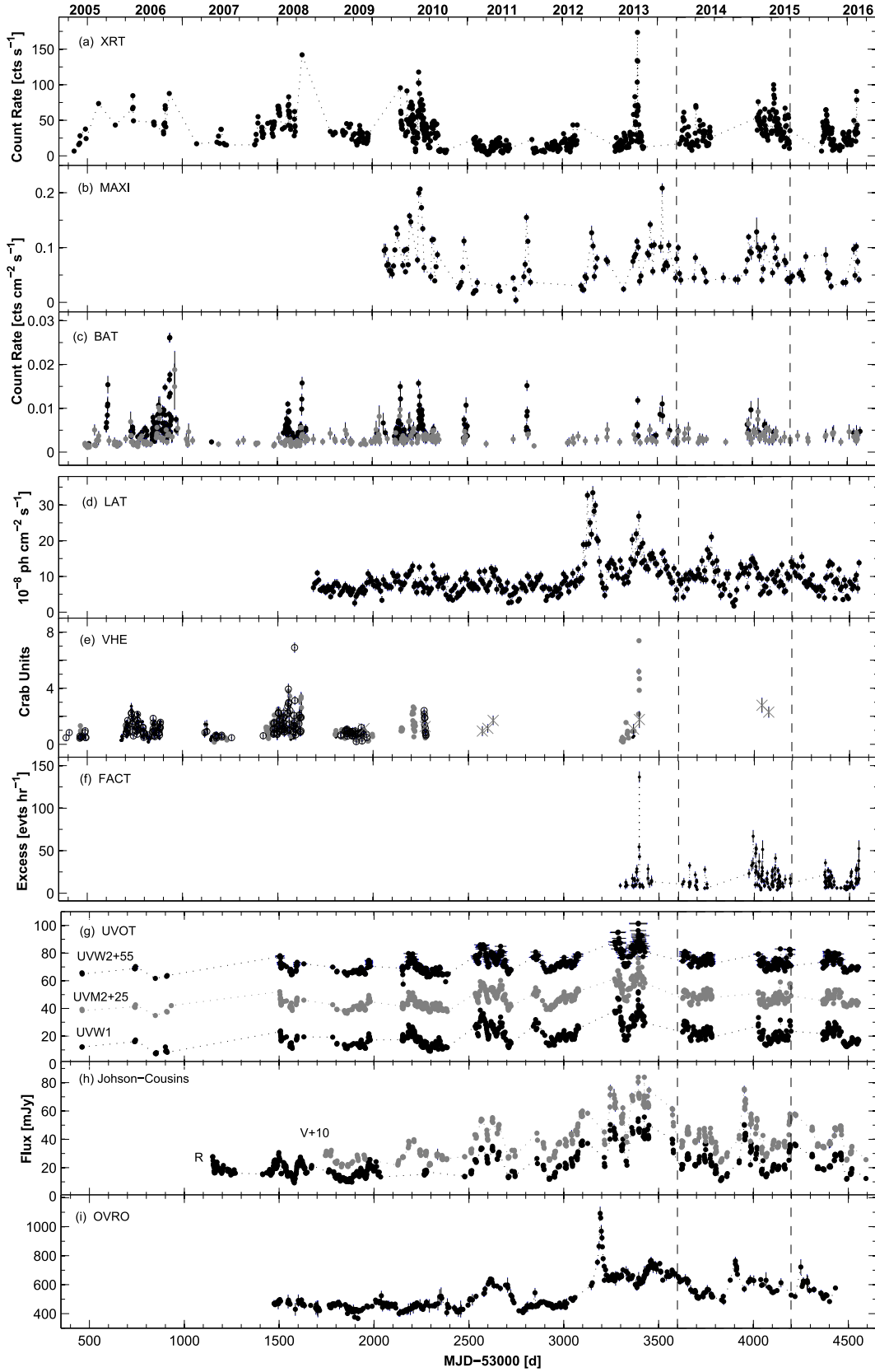
Figure 1. Historical light curves of Mrk 421 from the MWL observations in 2005–2016 performed with (a) XRT, (b) MAXI, (c) BAT (black and gray points stand for the detections with 5\sigma and 3\sigma significance, respectively), (d) LAT, (e) VHE (black points correspond to the VERITAS data; gray points, open circles, and asterisks correspond to those from the MAGIC, Whipple, and HAGAR observations, respectively), (f) FACT, (g) UVOT, (h) ground-based optical telescopes, and (i) the OVRO 40 m telescope. We used daily bins for XRT, BAT, FACT, UVOT, Steward, and OVRO data and 1-week bins for those of MAXI or LAT observations. The period 2013 November–2015 June (MJD 56,600–57,200) is confined within vertical dashed lines.
