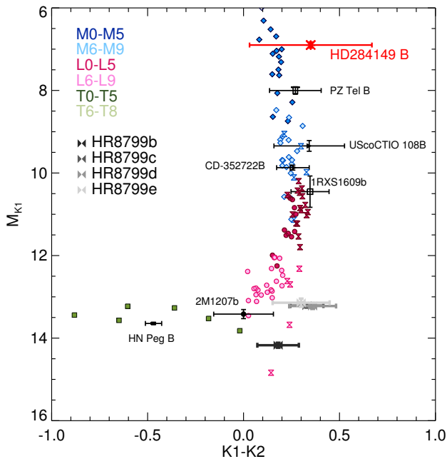
Fig. 8. Colour magnitude diagram showing the position of HD 284149 B (red bow tie) relative to that of M, L and T field dwarfs and of young known companions, based on the K1-K2 photometry from the non-coronagraphic IRDIS data (see text for details).
