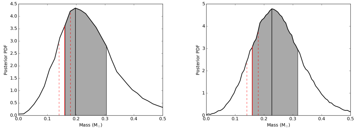
Fig. 11. Mass distribution of the companions compatible with the observed \Delta\mu , assuming a semi-major axis compatible with the observed projected separation of HD 2841419 B, and an eccentricity randomly drawn from a flat ( left panel ) or Gaussian ( right panel ) distribution. The black solid line shows the position of the most likely value and the shaded area highlights the region within a 1 sigma confidence level. The red solid line marks the value of the mass of HD 2841419 B (see Table 2).
