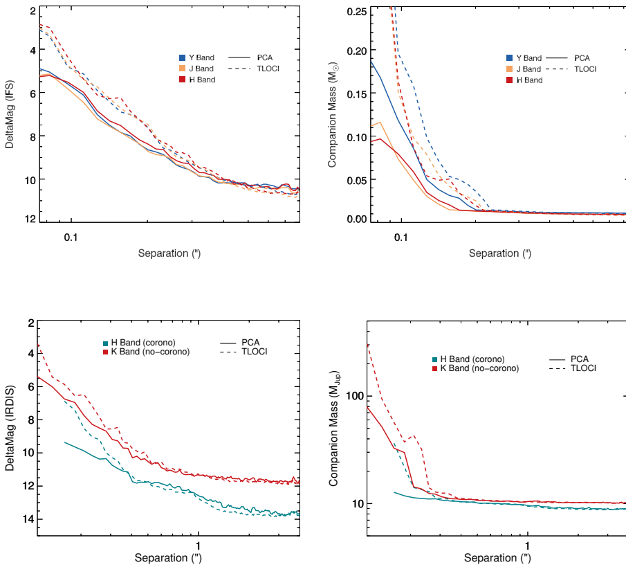
Fig. 2. IFS detection limits achieved during the non-coronagraphic observations of HD 284149 in terms of \Delta\text{mag} (left panel) and minimum companion mass (right panel) vs. separation. The mass limits are evaluated using the COND models by Baraffe et al. (2003) and assuming an age of 35 Myr. The different colours show the limits for the Y, J and H IFS filters respectively. The dashed line shows the limits evaluated using the images processed using the TLOCI method for speckle suppression (Marois et al. 2014), while the solid lines show the ones obtained using the images reduced using the PCA algorithm (Soummer et al. 2012; Amara & Quanz 2012).
