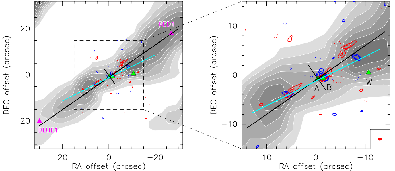
Fig. 1. ALMA CO(2–1) emission integrated over the blue- (–8, +1 km s –1 ) and red-shifted (+5, +18 km s –1 ) velocity ranges are compared with the PACS [OI] emission line at 63 μm by Nisini et al. (2015). The ALMA synthesised beam of the CO map is shown in the right panel. Green triangles indicate the positions of the three sources, as reported by Murillo et al. (2013b); magenta triangles label the closest CO knots identified by André et al. (1990). Black lines indicate the directions of the VLA1623A disk (PA = 35°, Murillo & Lai 2013a; Murillo et al. 2013b) and the relative outflow (PA = 125°). The latter is consistent with the large-scale CO outflow direction and with the secondary [OI] 63 μm peaks, whereas the closest [OI] 63 μm emission peaks are misaligned. The cyan line indicates the direction of the collimated jet (Br1 and Bb1 CO knots from Fig. 2), which is not associated with the large-scale CO outflow direction and with the direction perpendicular to the A disk, but it is rather associated with the closest [OI] 63 μm emission peaks.
