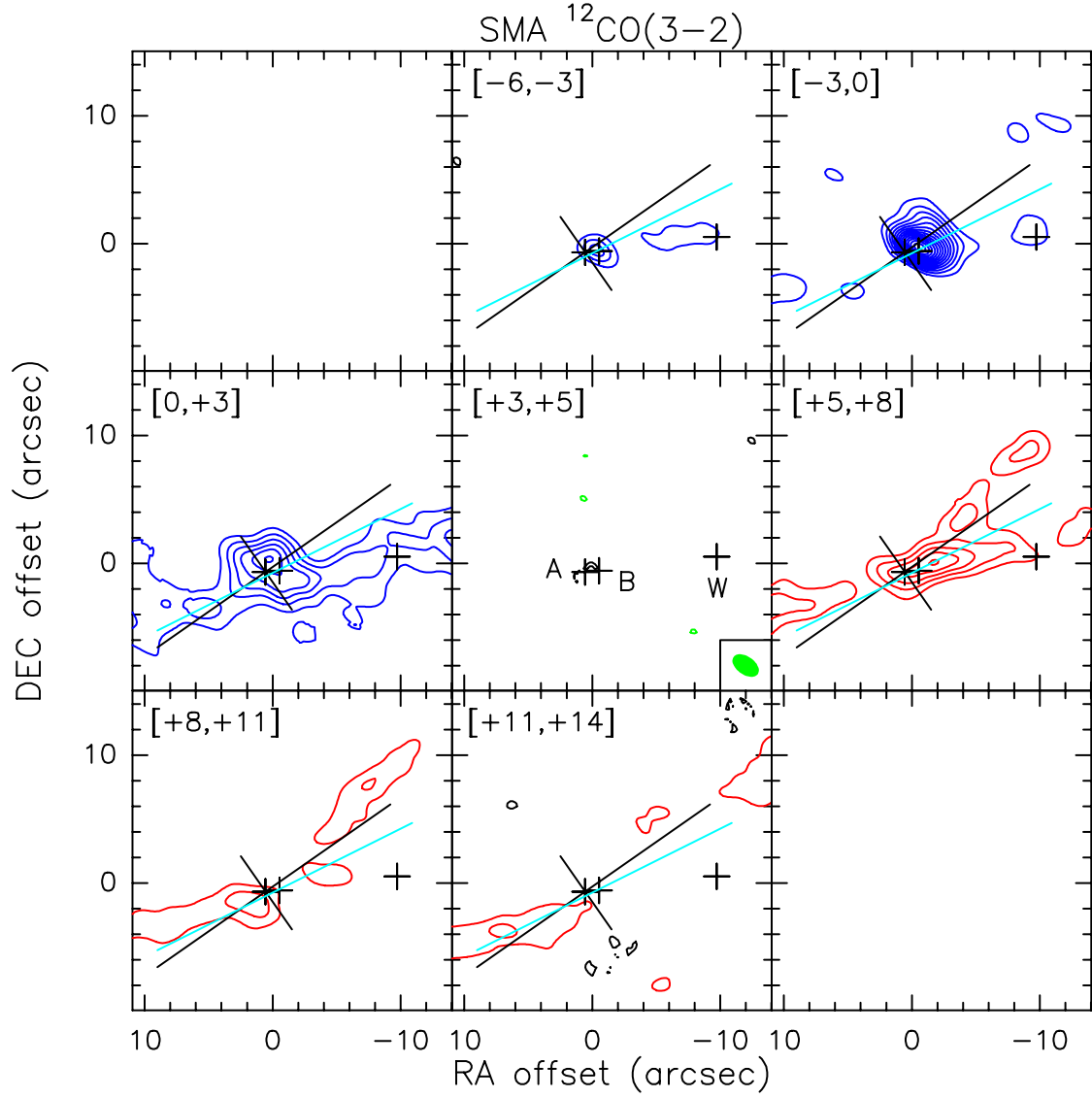
Fig. A.2. Channel maps of the SMA CO(3–2) emission. The velocity range of each map is indicated in the top left corner. The SMA synthesised beam of 2''.32 \times 1''.41 ( \text{PA} = 55^\circ ) is shown in the central panel. Contour levels of emission are traced starting at 3\sigma levels and increasing in steps of 3\sigma . Negative contours are displayed in black starting at 3\sigma level and decreasing in steps of 3\sigma . Black crosses represent the three protostars, which are labelled in the central panel. Black and cyan solid lines are the same as in Fig. 1.
