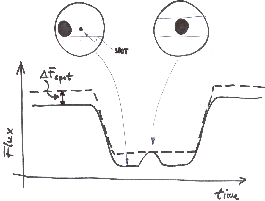
Fig. 7. The case of a transiting planets occulting a dark spot (at the disc centre) along the transit chord. The flux variation due to the transit in the case of a star with the spot is given by the solid line in the lower plot that shows a relative flux increase (a bump) when the spot is occulted. This happens because the corresponding configuration is the same as in the case without spot. In that case the reference flux level outside the transit is higher as shown by the dashed line that is the flux variation vs. the time in the case of a star without spots. The quantity \Delta F_{\text{spot}} measures the flux decrease due to the spot when it is in view on the stellar disc.
