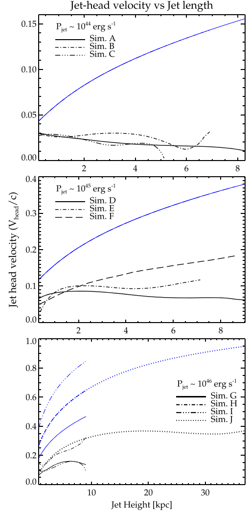
Figure 15. Speed of advance of the jet head as a function of jet height (see Section 3.4). In blue is plotted the maximum velocity expected from a non-decelerating jet following equation (19) (as derived in Martí et al. 1997).
