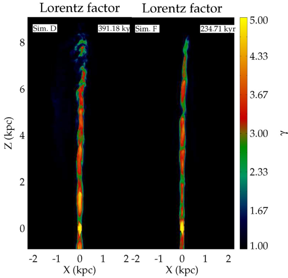
Figure 7. Plots of the Lorentz factor in the X–Z plane for simulations D and F. Simulation D shows deceleration at the top with irregular distribution of flow implying onset of decollimation. Simulation F shows a steady cylindrical spine along the Z.
