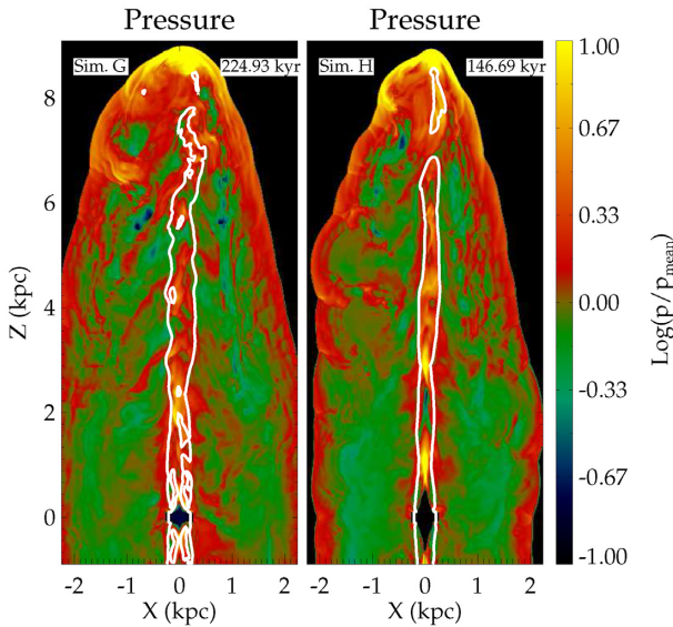
Figure 11. Plots of the pressure normalized to its mean value in the X – Z plane for simulations G and H. The white contours denote constant Lorentz factor with a value \gamma = 2 . Simulation G with a higher initial pressure but lower Lorentz factor has irregular jet axis (traced by the \gamma = 2 contour), bending of the jet, and more pronounced internal structures, implying faster growth of unstable modes (Kelvin–Helmholtz). Simulation H has a more regular jet axis and cocoon than that in G.
