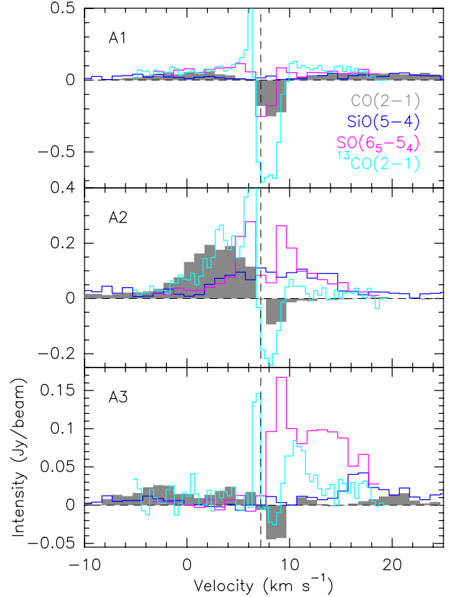
Fig. 3. 12 CO(2–1) (grey), SiO(5–4) (blue), SO(6 5 –5 4 ) (magenta), and 13 CO(2–1) (cyan) at the positions of the continuum sources A1, A2, and A3 (see Fig. 5). The selected positions are displayed from top to bottom. The 12 CO(2–1) data have been convolved to match the angular resolution at 1.4 mm (1''.1 × 0''.8). The vertical dashed line marks the systemic velocity of +7.2 km s -1 for the three continuum sources. We note that the systemic velocity of A3 has been derived from PdBI N 2 H + (1–0) observations at 93.17 GHz from our CALYPSO dataset.
