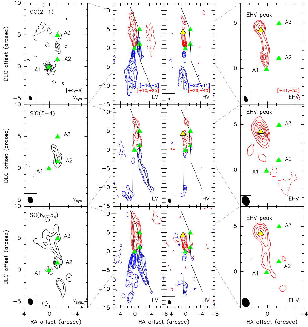
Fig. 5. Upper: channel maps of the ^{12}\text{CO}(2-1) emission integrated in the ambient systemic- ( v_{\text{sys}} ; +6, +9 km s ^{-1} ), low- (LV; -10, +5 km s ^{-1} ) and +10, +25 km s ^{-1} ), high- (HV; -20, -11 km s ^{-1} and +26, +40 km s ^{-1} ), and extremely high- (EHV; +41, +55 km s ^{-1} ) velocity ranges. The contour levels of emission are traced at 5 and 8 \sigma levels and increase in steps of 5 \sigma . Negative emission is shown with dashed contours starting at the 3 \sigma level and decreasing in steps of 3 \sigma . The positions of the continuum sources at 1.3 mm are marked in green and the position of the SiO(5-4) emission peak in the EHV range is marked in yellow. The PdBI synthesised beams (HPBW) are shown in the bottom-left corner. Solid black curves indicate the proposed propagation directions of the A1 and A2 jets. Middle: same as the upper panel for the SiO(5-4) emission. Lower: same as the upper panel for the SO(6 _5 -5 _4 ) emission.
