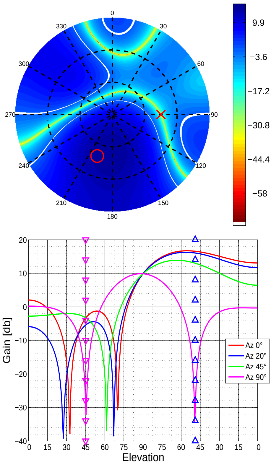
Figure 5.19: Antenna Pattern for Channel 10
