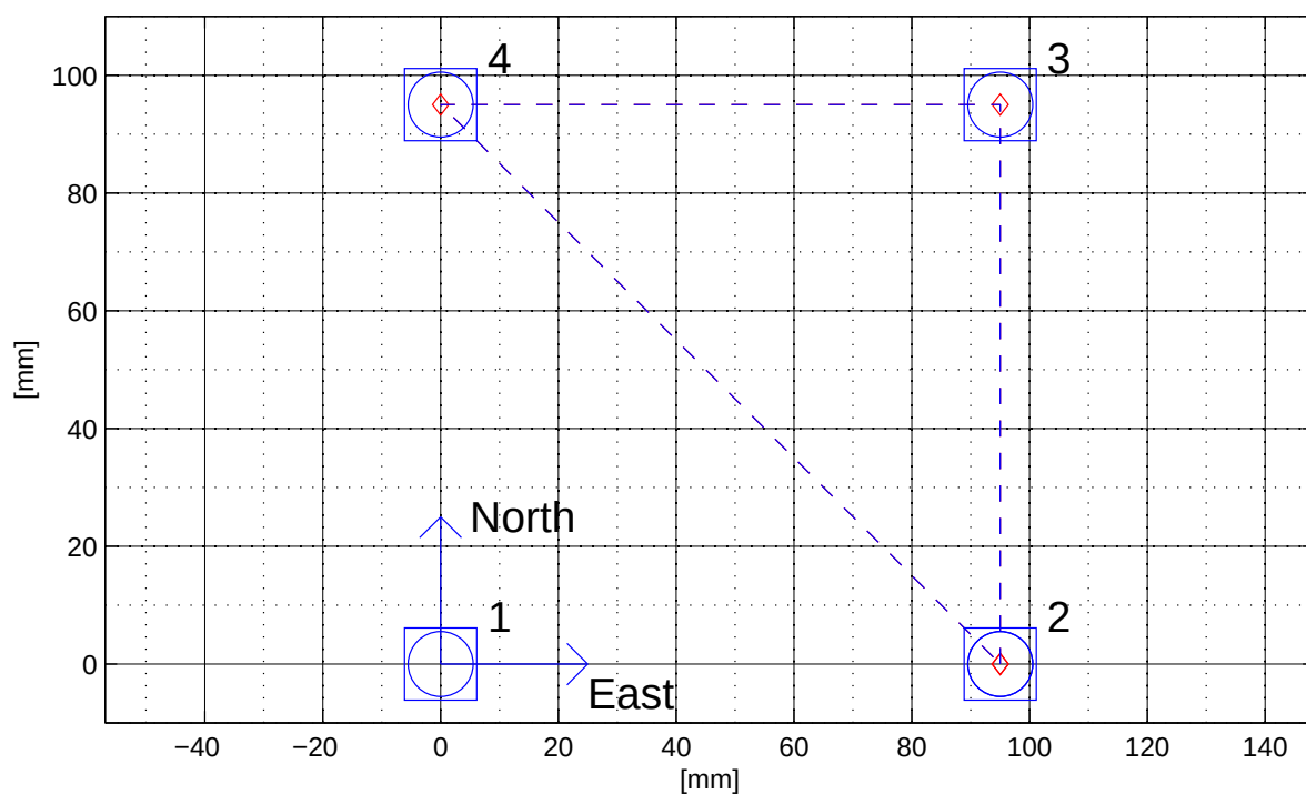
Figure 5.34: Antenna Array Map
