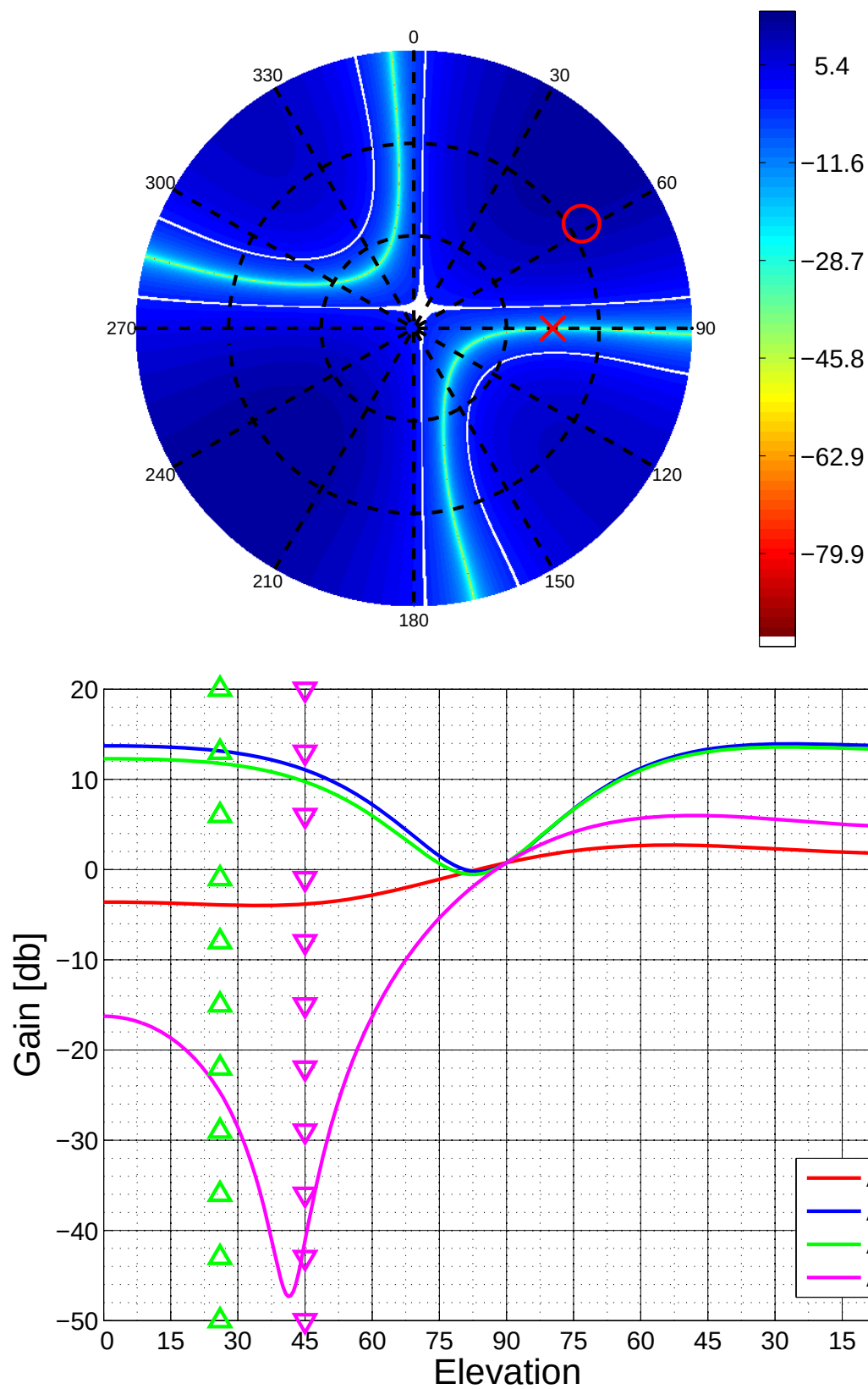
Figure 5.46: Antenna Pattern for Channel 2
