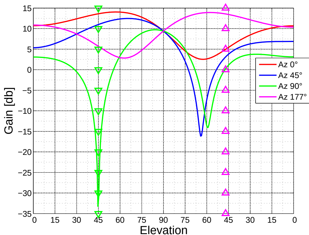
Figure 5.66: Antenna Pattern for Channel 16 : modelled antenna gains mismatch
