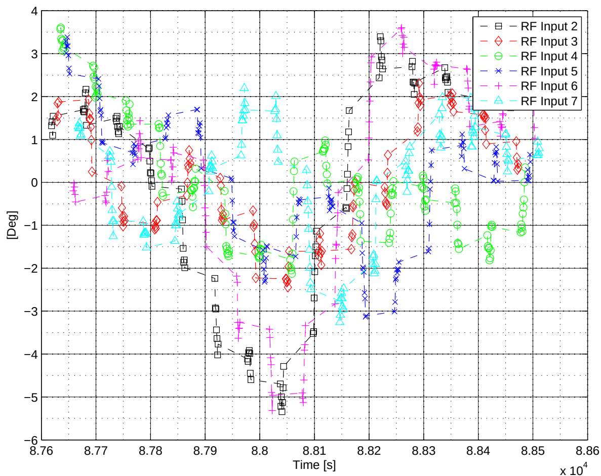
Figure 5.79: "De-biased" Phase Offsets for RF Inputs 2 - 7
