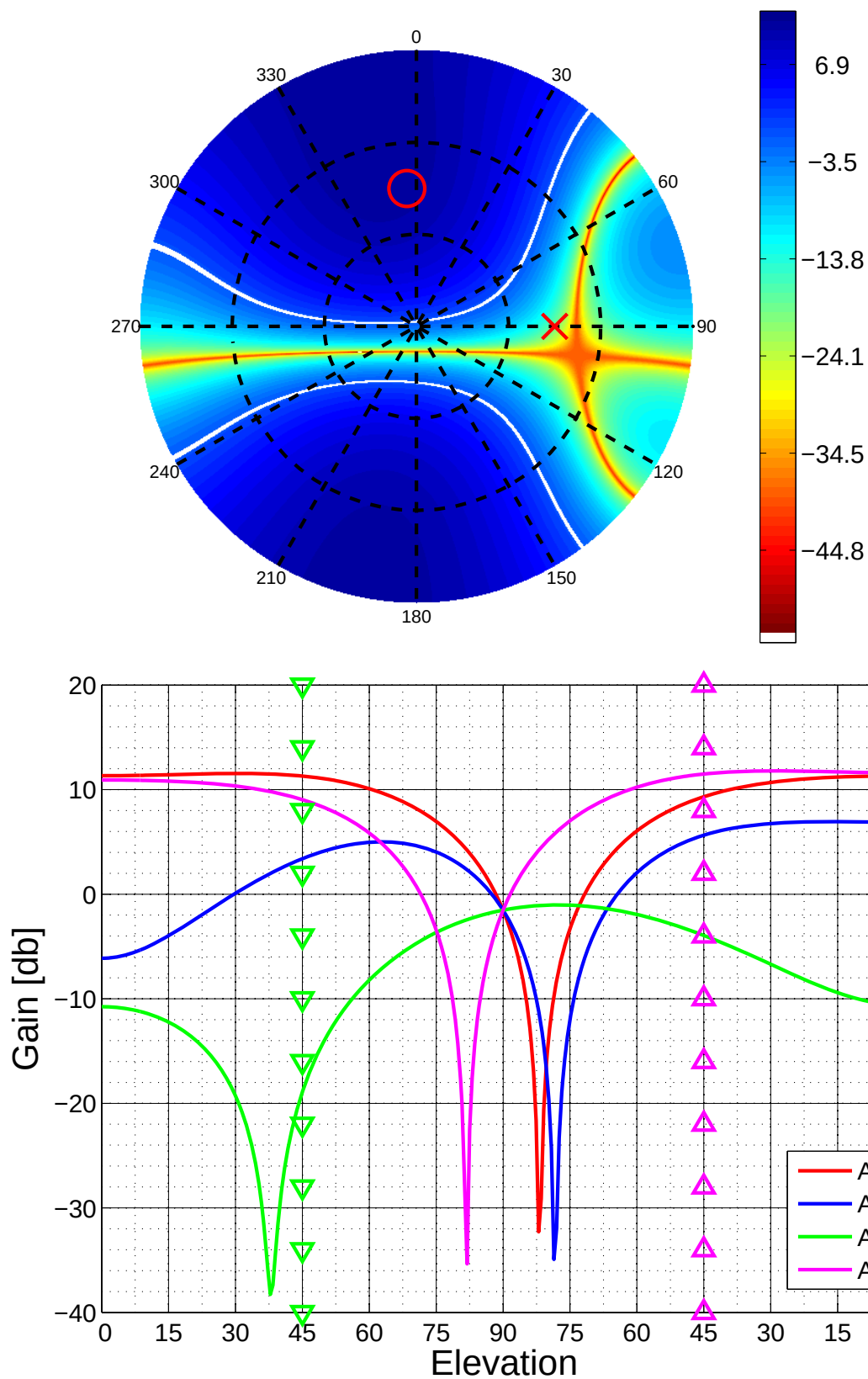
Figure 5.44: Antenna Pattern for Channel 16
