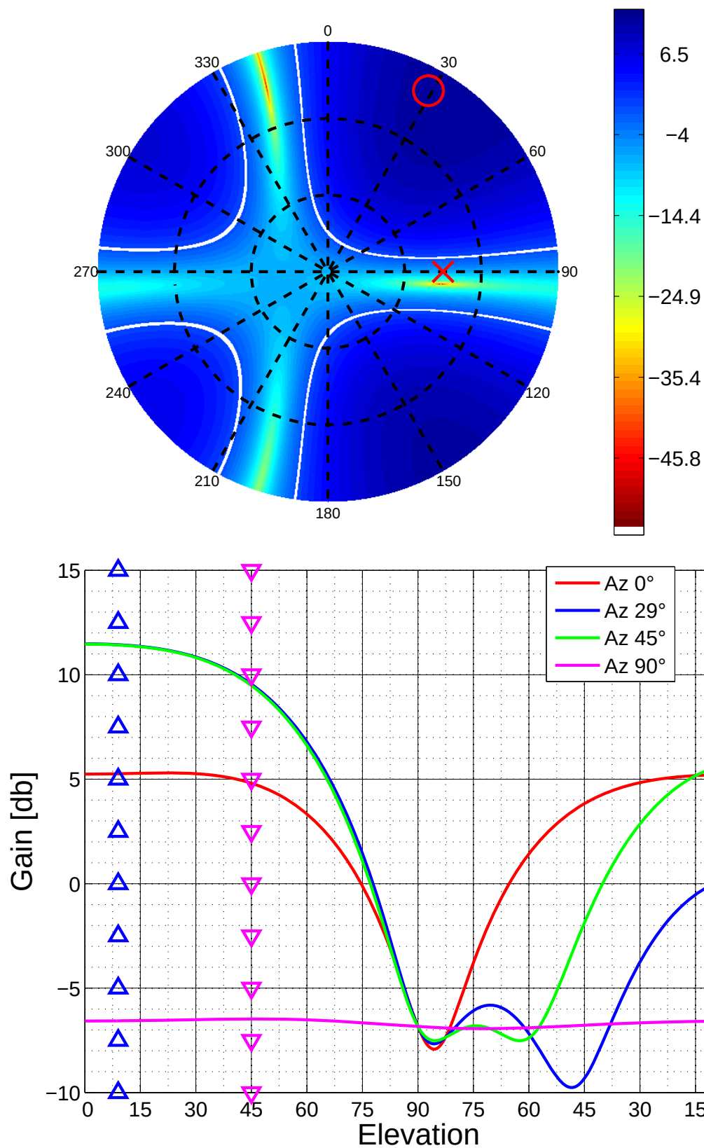
Figure 5.39: Antenna Pattern for Channel 7
