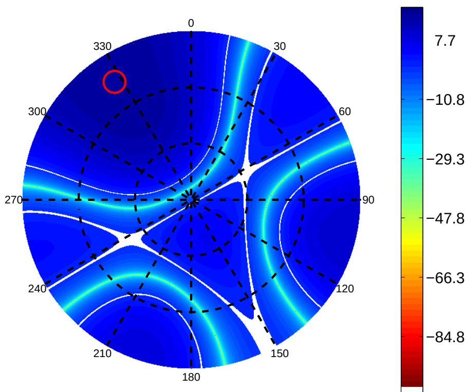
Figure 5.3: Nominal Mode Test Antenna Pattern For Channel 3
