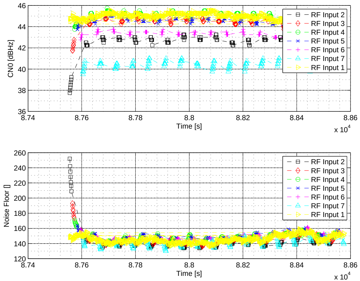
Figure 5.81: SNR and Noise Floor vs Time
