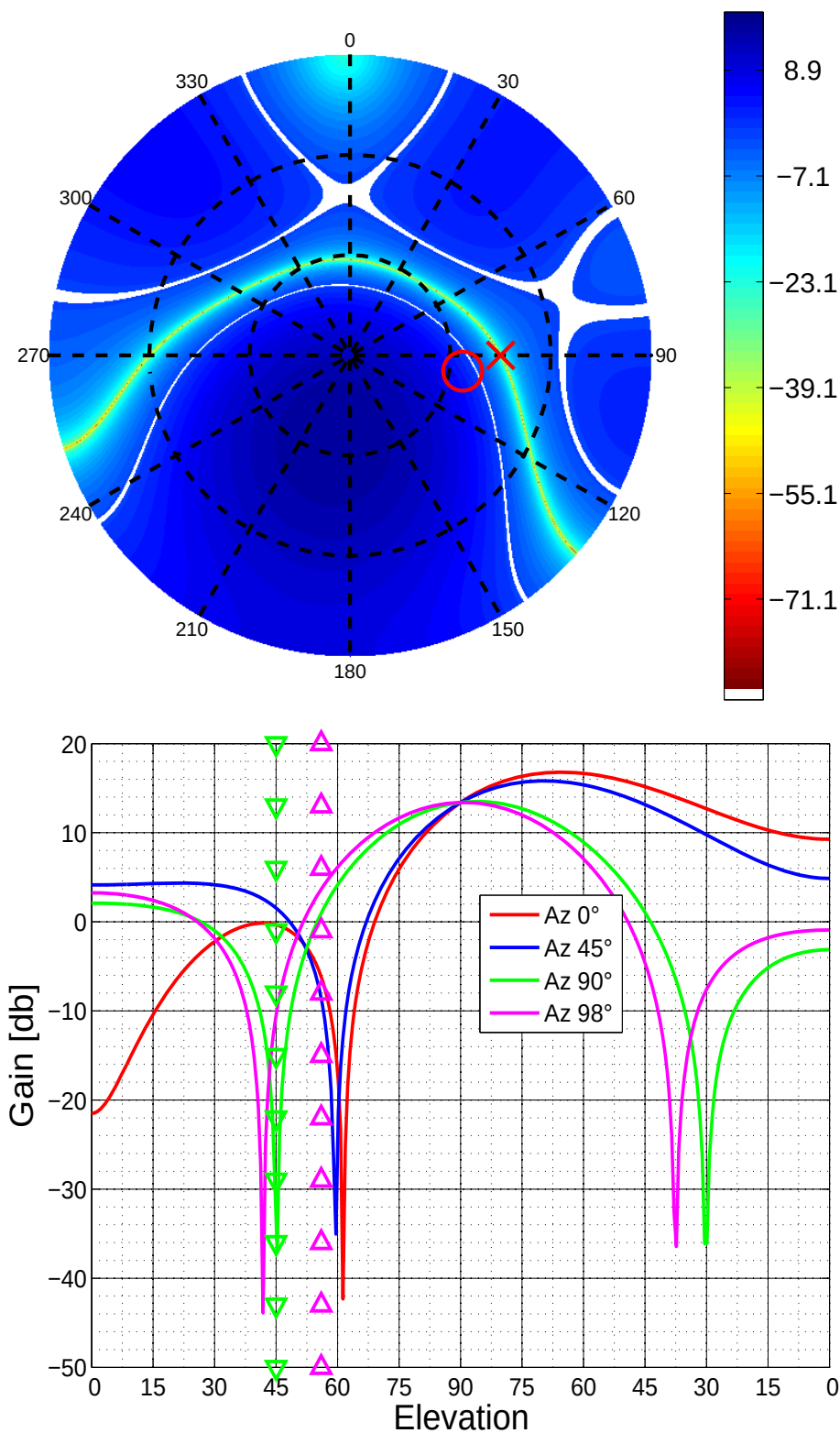
Figure 5.18: Antenna Pattern for Channel 9
