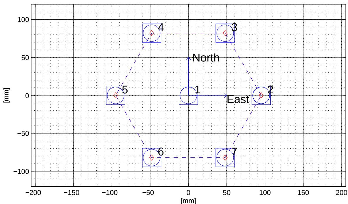
Figure 5.12: Antenna Array Map
