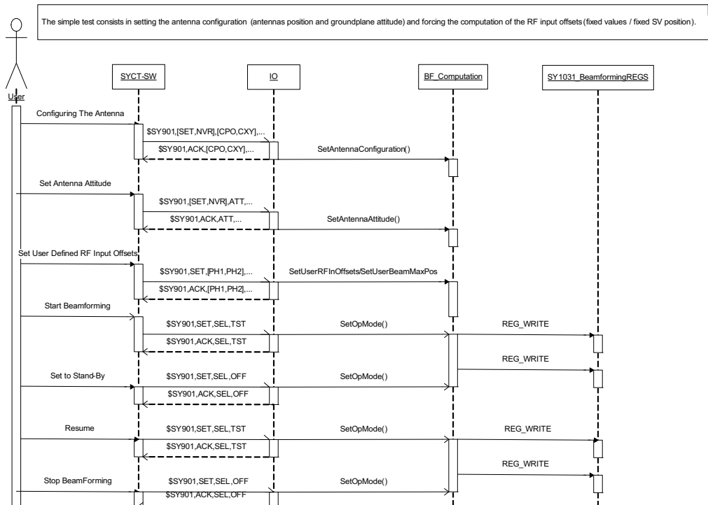
Figure 3.5: Sequence 1 – simple test sequence diagram
