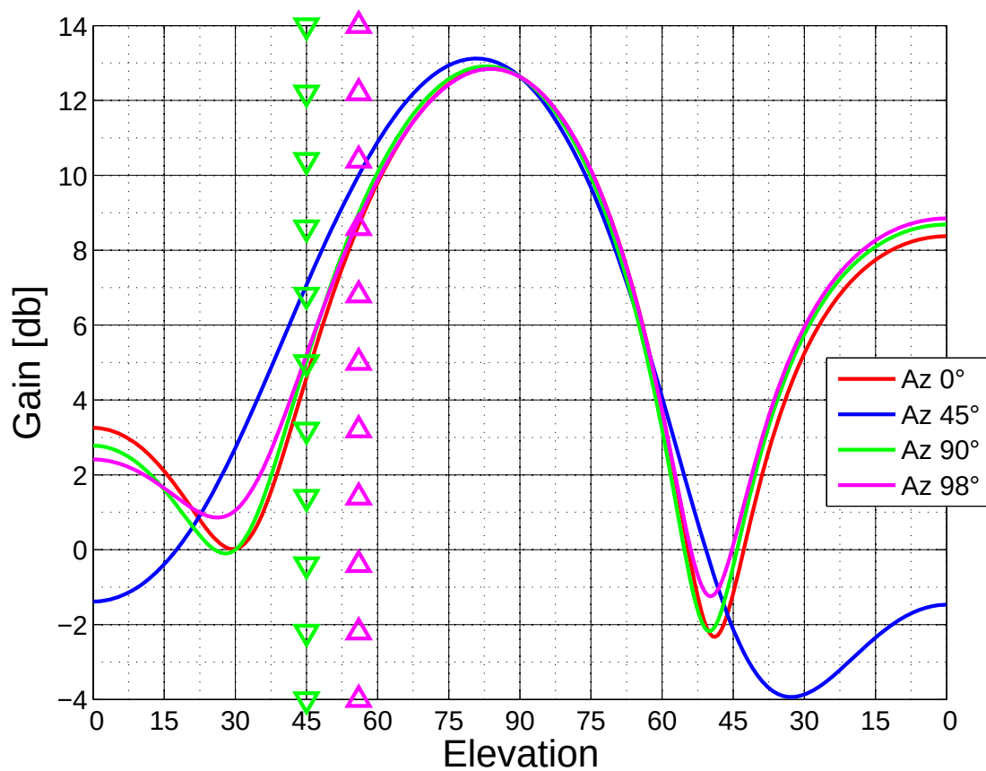
Figure 5.51: Antenna Pattern for Channel 9
