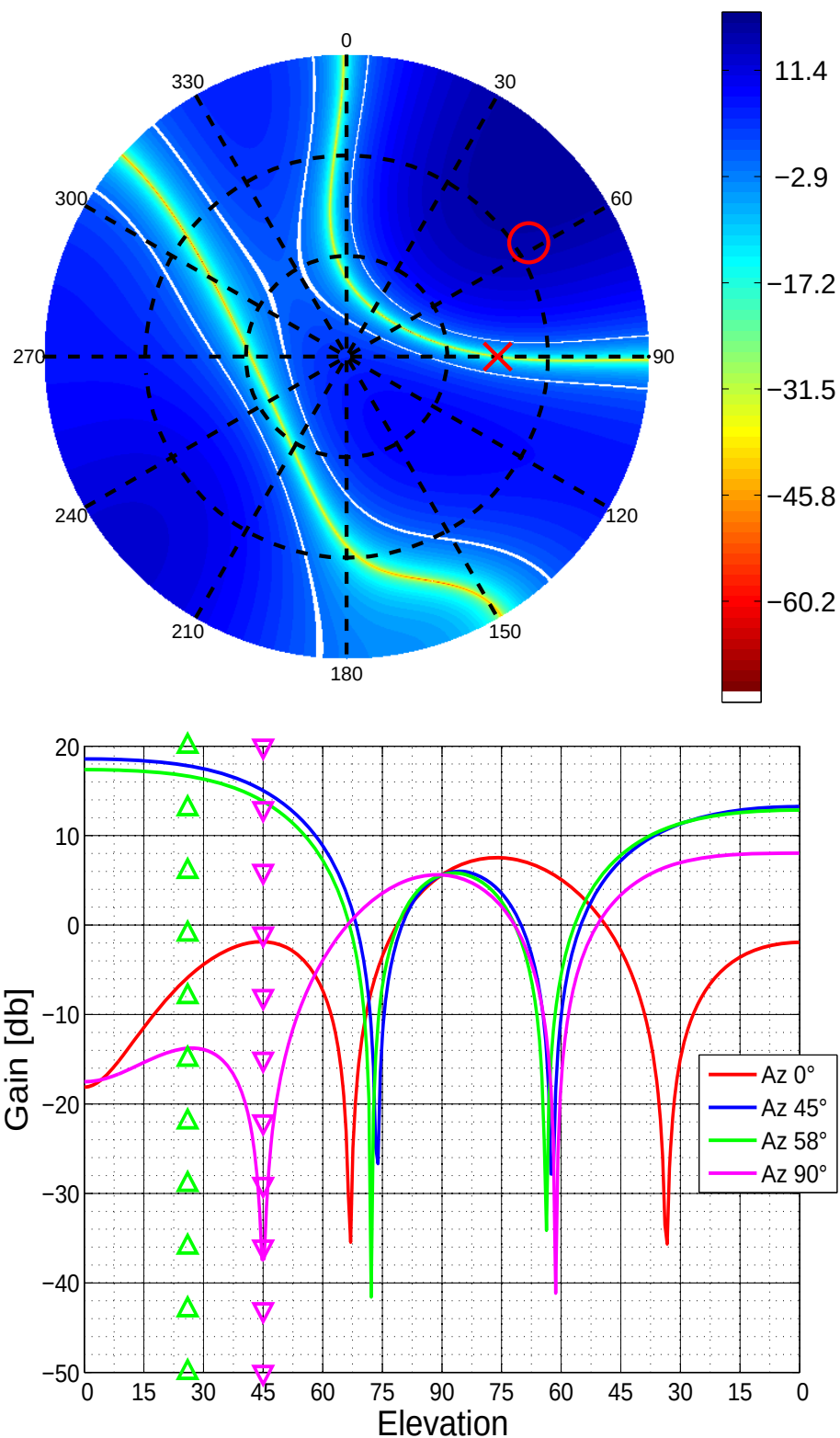
Figure 5.24: Antenna Pattern for Channel 2
