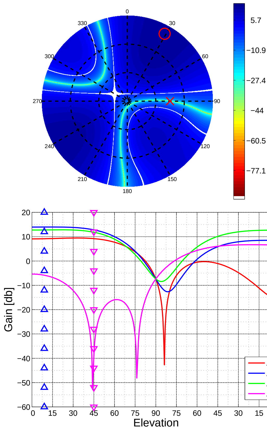
Figure 5.50: Antenna Pattern for Channel 7
