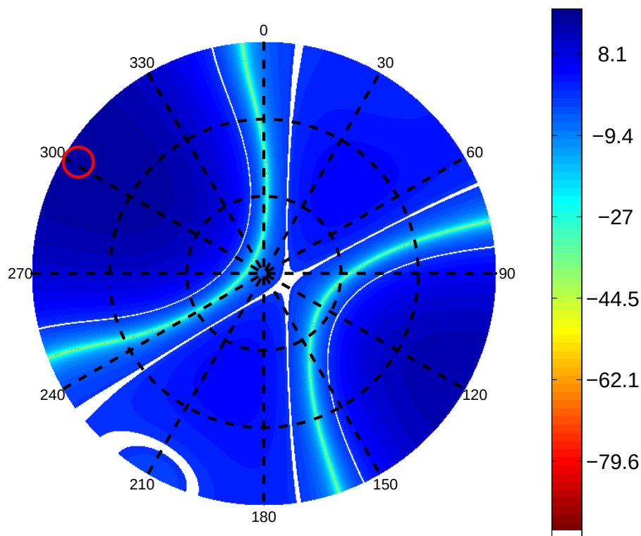
Figure 5.4: Nominal Mode Test Antenna Pattern For Channel 4
