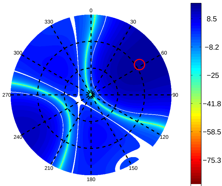
Figure 5.2: Nominal Mode Test Antenna Pattern For Channel 2
