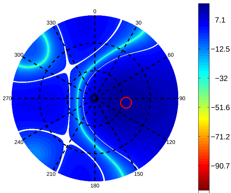
Figure 5.7: Nominal Mode Test Antenna Pattern For Channel 9
