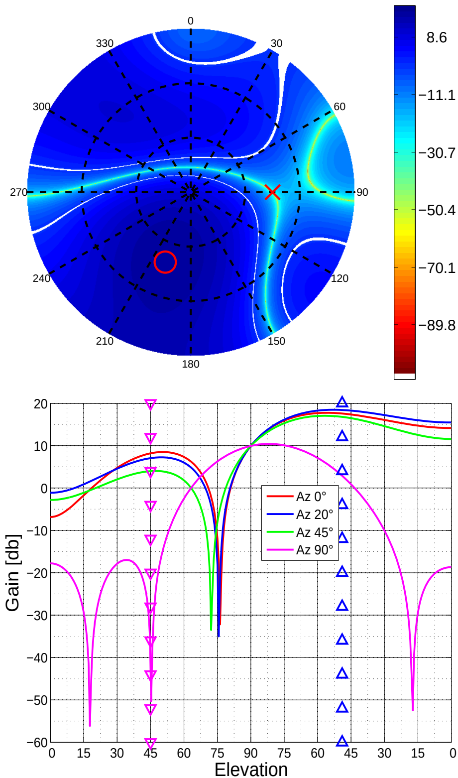
Figure 5.30: Antenna Pattern for Channel 10
