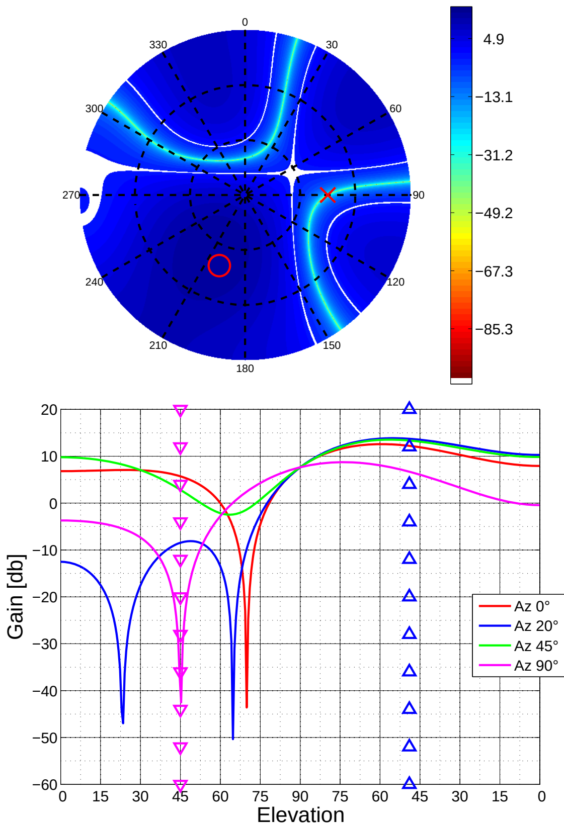
Figure 5.52: Antenna Pattern for Channel 10
