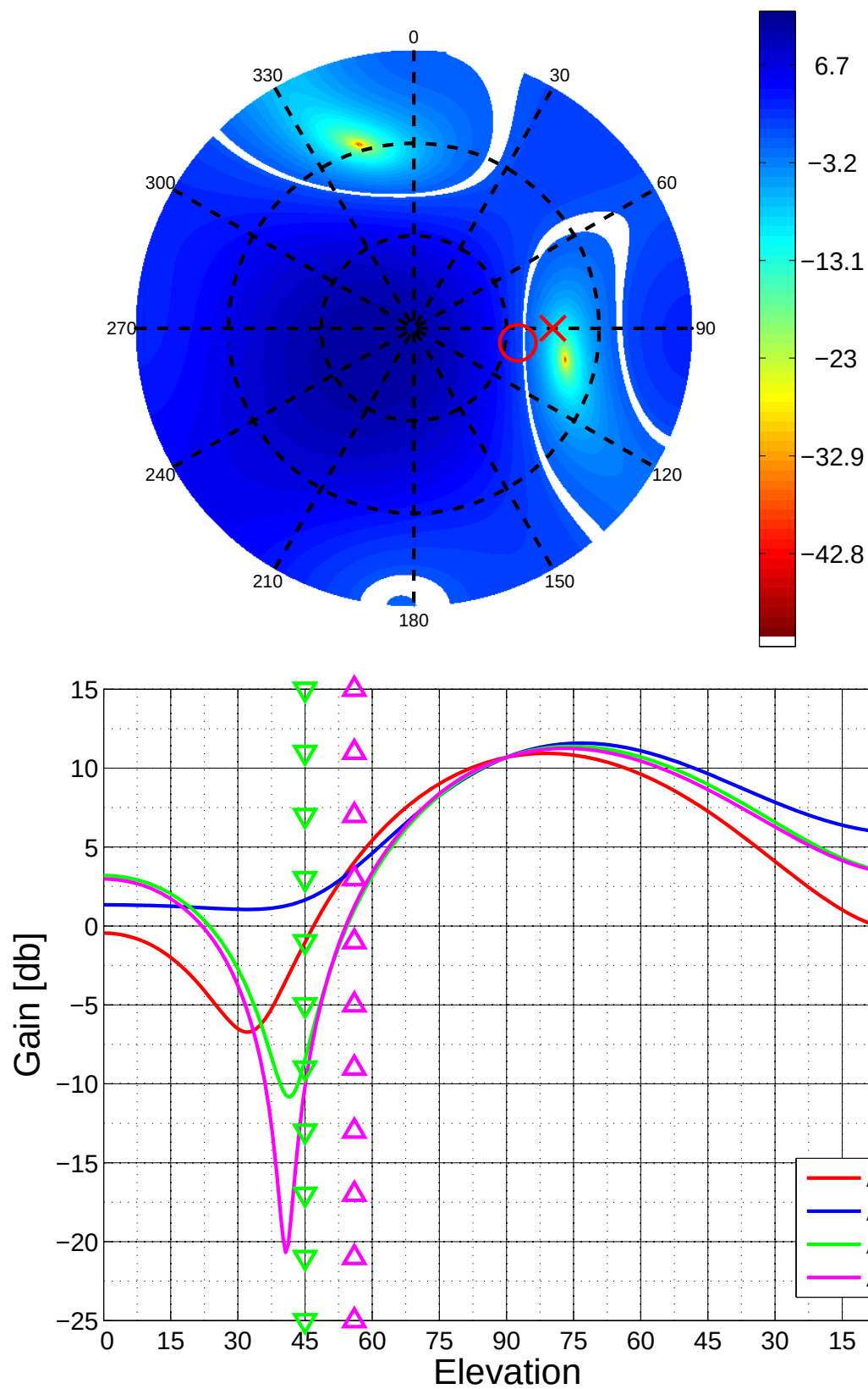
Figure 5.40: Antenna Pattern for Channel 9
