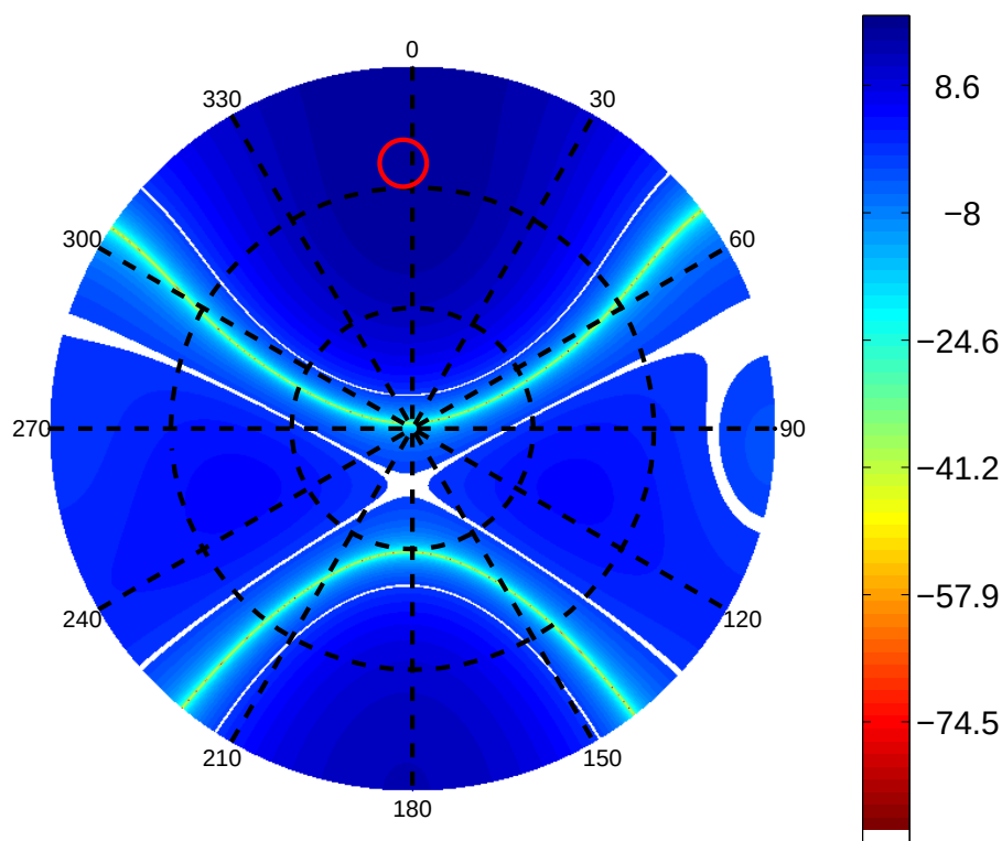
Figure 5.5: Nominal Mode Test Antenna Pattern For Channel 6
