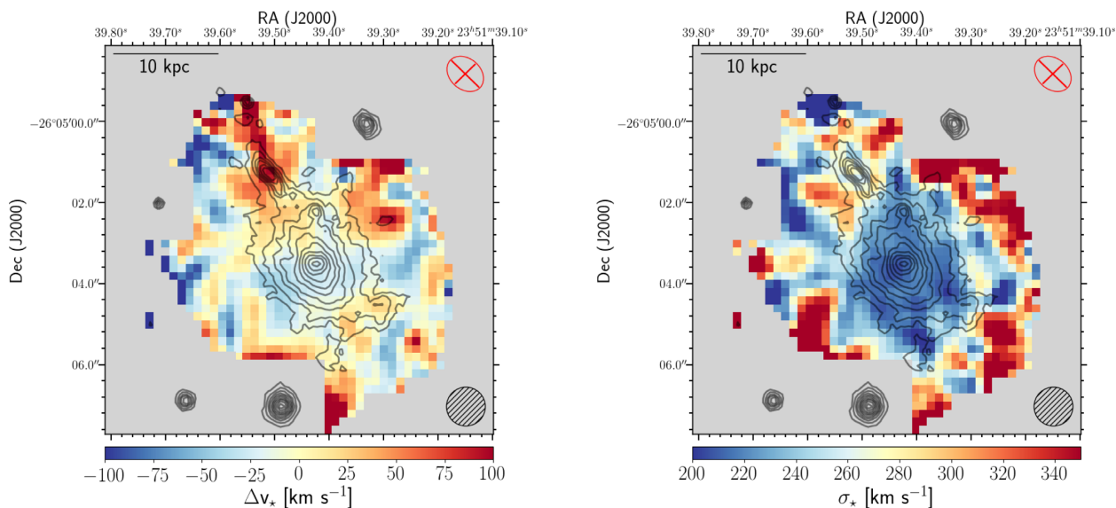
Figure 2. pPXF maps for the stellar velocity (left-hand panel) and velocity dispersion (right-hand panel) along the observer's line of sight, with the Hubble Space Telescope F450W WFPC2 contours superimposed (grey solid lines). In both maps, the spaxels with an SNR < 3 are coloured in grey. The hatched black circle on the bottom right-hand side shows the beam size of the average V-band observed seeing of \sim 0.96 arcsec (FWHM) while the red ellipse at the top indicates the galaxy orientation in the sky-plane. The ratio between the ellipse's axes corresponds to the b/a value retrieved by the two-dimensional surface brightness model of the galaxy by GALFITM.
