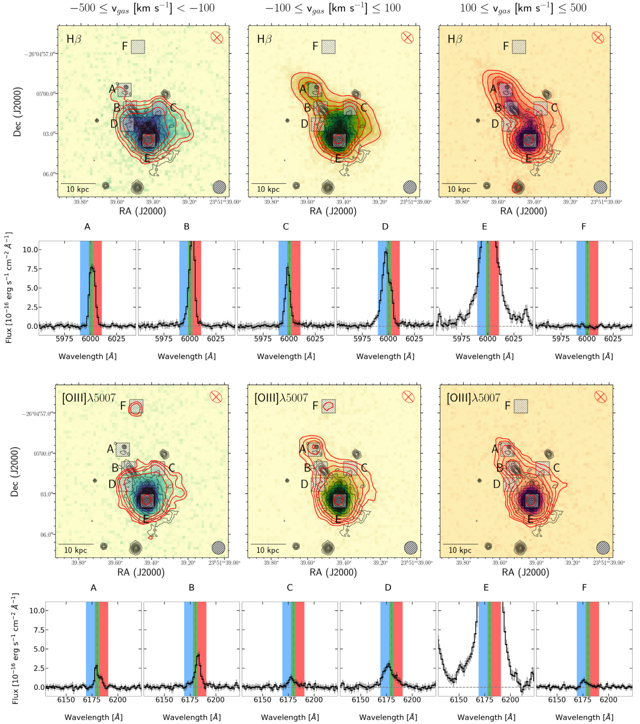
Figure 7. H\beta (top panels) and [OIII] \lambda 5007 (bottom panels) emission in Abell 2667 BCG with contours and symbols as defined in Fig. 2. The images show the emission line integrated flux within three different velocity channels: from -500 to -100 \text{ km s}^{-1} (blue), from -100 to 100 \text{ km s}^{-1} (green), and from 100 to 500 \text{ km s}^{-1} (red). In each panel, the red solid lines are indicative of the 85.0, 90.0, 93.0, 95.5, and 99.7 percentiles of the emission line flux, respectively. For both H\beta and [OIII] \lambda 5007 , we report cut-outs of the integrated spectra of six peculiar small ( 1 \text{ arcsec} \times 1 \text{ arcsec} ) sky regions, labelled with capital letters, and chosen to be representative of very different areas of the galaxy. In each cut-out, the shaded areas indicate the different velocity ranges we adopted.
