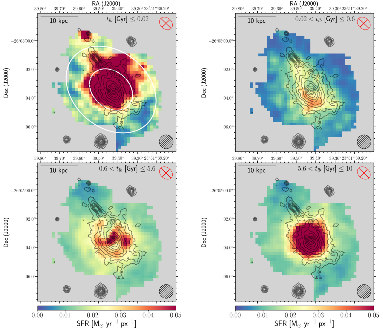
Figure 3. SINOPSIS SFR density maps of the Abell 2667 BCG in the look-back time ( t_{lb} ) intervals t_{lb} [\text{Gyr}] \leq 0.02 (top left), 0.02 < t_{lb} [\text{Gyr}] \leq 0.6 (top right), 0.6 < t_{lb} [\text{Gyr}] \leq 5.6 (bottom left), and 5.6 < t_{lb} [\text{Gyr}] \leq 10 (bottom right), respectively. In the top left-hand panel, the two white ellipses show the spatial extent of the regions we define as nuclear and outskirt in Fig. 4. Contours and symbols are defined as in Fig. 2.
