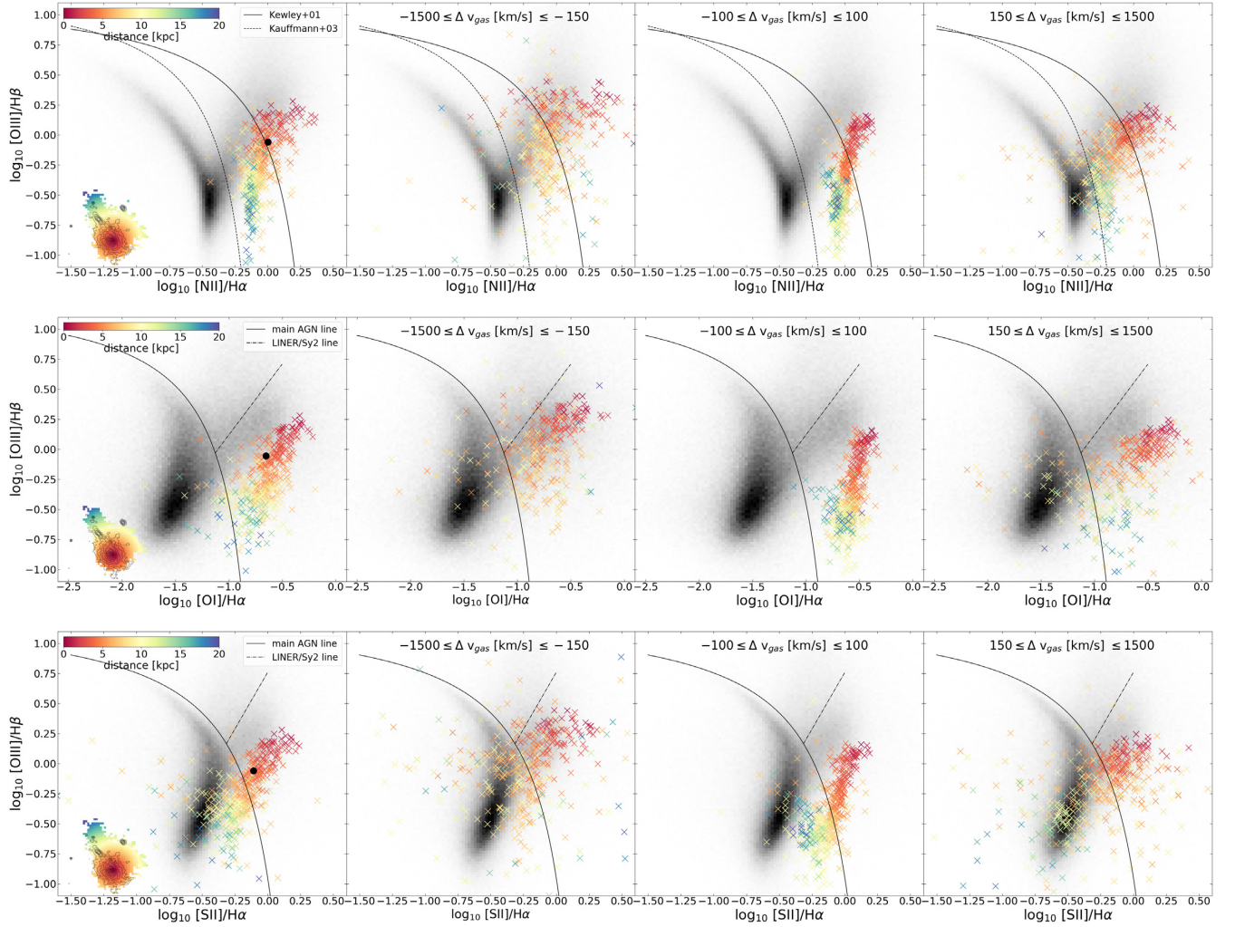
Figure 8. From top to bottom, the BPT-[N II], BPT-[O I], and the BPT-[S II] diagrams for the spaxels with \text{SNR}([\text{O III}] \lambda 5007) > 3 . For each diagnostic, from left to right we report the diagram obtained integrating all the fluxes within -1500 \text{ km s}^{-1} to 1500 \text{ km s}^{-1} , and in the velocity ranges -1500 \text{ km s}^{-1} to -150 \text{ km s}^{-1} (blueshifted outflow), -100 \text{ km s}^{-1} to 100 \text{ km s}^{-1} (disc), and 150 \text{ km s}^{-1} to 1500 \text{ km s}^{-1} (redshifted outflow), respectively. Each mark is representative of a spaxel and is colour-coded according to its distance from the BCG centre (see the colourbar at the top left and the colour map at the bottom left of the left-hand panels). To separate the loci corresponding to star-forming galaxies, transition objects, and AGNs, we report the empirical relations by Kewley et al. (2001) and Kauffmann et al. (2003). Finally, we report in black the distribution of the emission line galaxies in the Sloan Digital Sky Survey DR7 (Abazajian et al. 2009).
