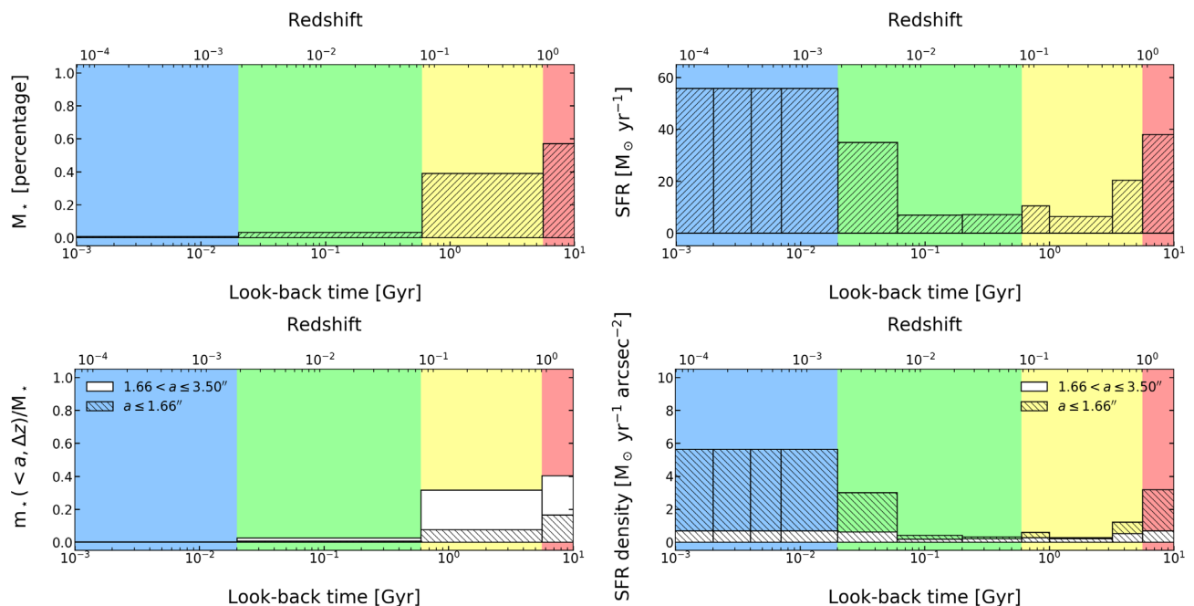
Figure 4. Top panels: SINOPSIS spatially integrated mass building (left-hand panel) and star formation history (right-hand panel) of the Abell 2667 BCG. The colour-shaded areas of the diagrams represent the four main age bins within which SINOPSIS calculates the galaxy percentage of mass built and the SFR (see Fig. 3). In the right-hand panel, the histogram show the SFH computed in the highest temporal resolution mode (11 SSP age intervals). Both the percentage of mass built and the SFR of each time-bin have been obtained integrating all the maps' values within an elliptical region centred at the galaxy coordinates, with axis ratio b/a = 0.76 , position angle PA = 48.89^\circ (for the parameters see Section 3.1), and semimajor axis a = 3.5 arcsec. Bottom panels: percentage of stellar mass built (left-hand panel) and SFR density (right-hand panel) at different epochs for the nuclear (hatched histogram) and external regions (white histogram) of the BCG. For the nuclear region we have integrated SINOPSIS spatially resolved values within an elliptical aperture centred at the galaxy coordinates, with b/a and PA as before but a = 1.66 arcsec. For the outskirts, we have resorted to an elliptical annulus with central coordinates, b/a and PA as before, but with 1.66 \text{ arcsec} < a \leq 3.55 \text{ arcsec} . The two different areas are marked with the two white ellipses in the top left-hand panel of Fig. 3.
