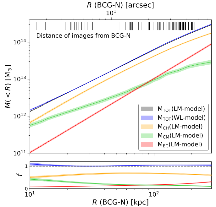
Fig. 7. Cumulative total mass profiles of the different mass components considered in the lens models. Top : cumulative total mass distribution of A2744 as a function of the projected distance R from BCG-N obtained from the reference lens model. The different components of the total mass are shown: cluster halo (CH), cluster members (CM, including the BCGs), and external clump (EC). The distances of the observed multiple images from BCG-N are plotted using small vertical bars. Bottom : ratio between the projected mass profiles obtained for the different color-coded mass components and the total cluster mass.
