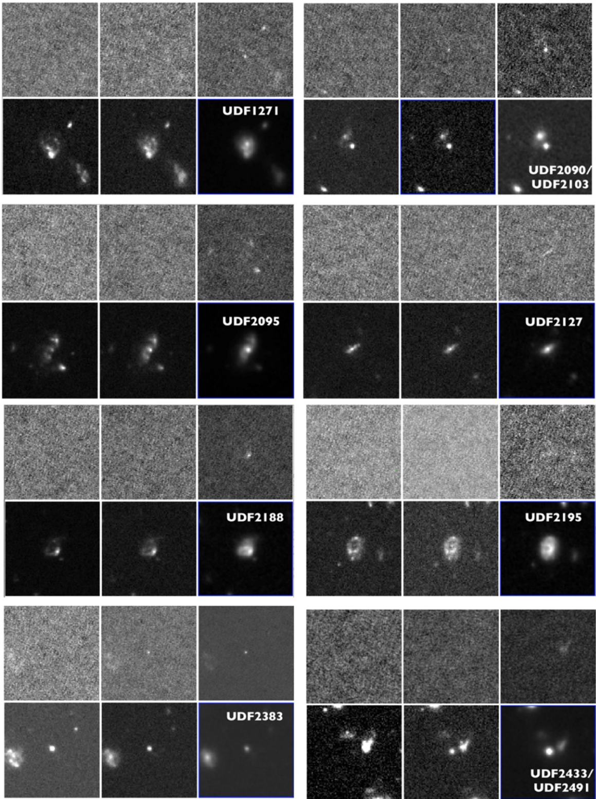
Figure 11. HUDFJ0332.4-2746.6 candidates. For each candidate, starting from the top left, we show clockwise WFC3 F_{225W} , F_{275W} , and F_{336W} from UVUDF, ACS F_{435W} , I_{814} , and WFC3 J_{125} images. Galaxies are identified by their 3D- HST ID. The size of each image is 5'' . All candidates are F_{275W} dropouts.
