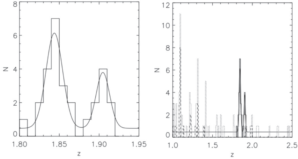
Figure 1. On the left, the redshift distribution of HUDFJ0332.4-2746.6 and HUDFJ0332.5-2747.3 spectroscopic members. The continuous line is the double Gaussian fit described in the text. On the right, we also show the spectroscopic redshift distribution in the HUDF from the 3D- HST (dashed line) and the GOODS and GMASS catalogs (dotted line).
