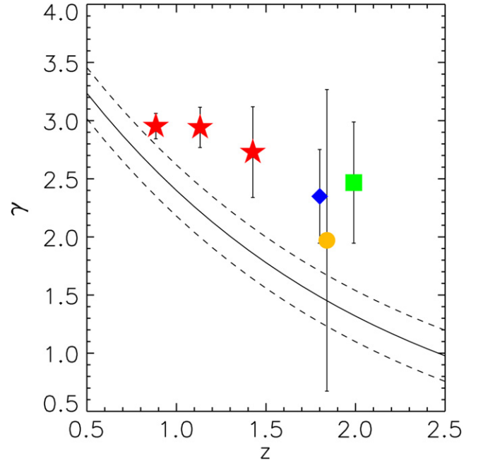
Figure 10. Median mass-normalized B-band rest-frame size \gamma , as a function of redshift. The yellow circle is the median \gamma for HUDFJ0332.4-2746.6 ETGs. The red stars are the median \gamma s for quiescent ETGs in clusters at 0.7 < z < 1.6 from Delaye et al. (2014). The green square and the blue diamond are the median \gamma s for quiescent ETGs from CL J1449+085 at z = 1.99 (Strazzullo et al. 2013) and JKCS 041 at z = 1.8 (Newman et al. 2014), respectively. Our structures' star-forming blue ETGs are consistent with those of quiescent ETGs in dense environments at similar redshifts. Both star-forming and quiescent ETGs in dense environments do not show much evolution in the redshift range of z = 0.7-2 . The continuous line shows the evolution of field galaxies and is from Newman et al. (2012).
