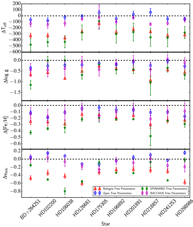
Fig. 8. The \Delta T_{\text{eff}} , \Delta \log g , \Delta [\text{Fe}/\text{H}] , and \Delta v_{\text{mic}} computed from the free run (described in Sect. 5) for each star from top to bottom, respectively. We note here that the \Delta represents the difference of the node and adopted values for each parameter. For example, \Delta \log g = \log g_{\text{node}} - \log g_{\text{adopted}} . The BACCHUS (ULB) method is denoted as the open magenta diamond, the iSpec method is denoted as the open blue hexagon, the EPINARBO method is denoted as an open green star and the Bologna method is denoted as an open red triangle.
