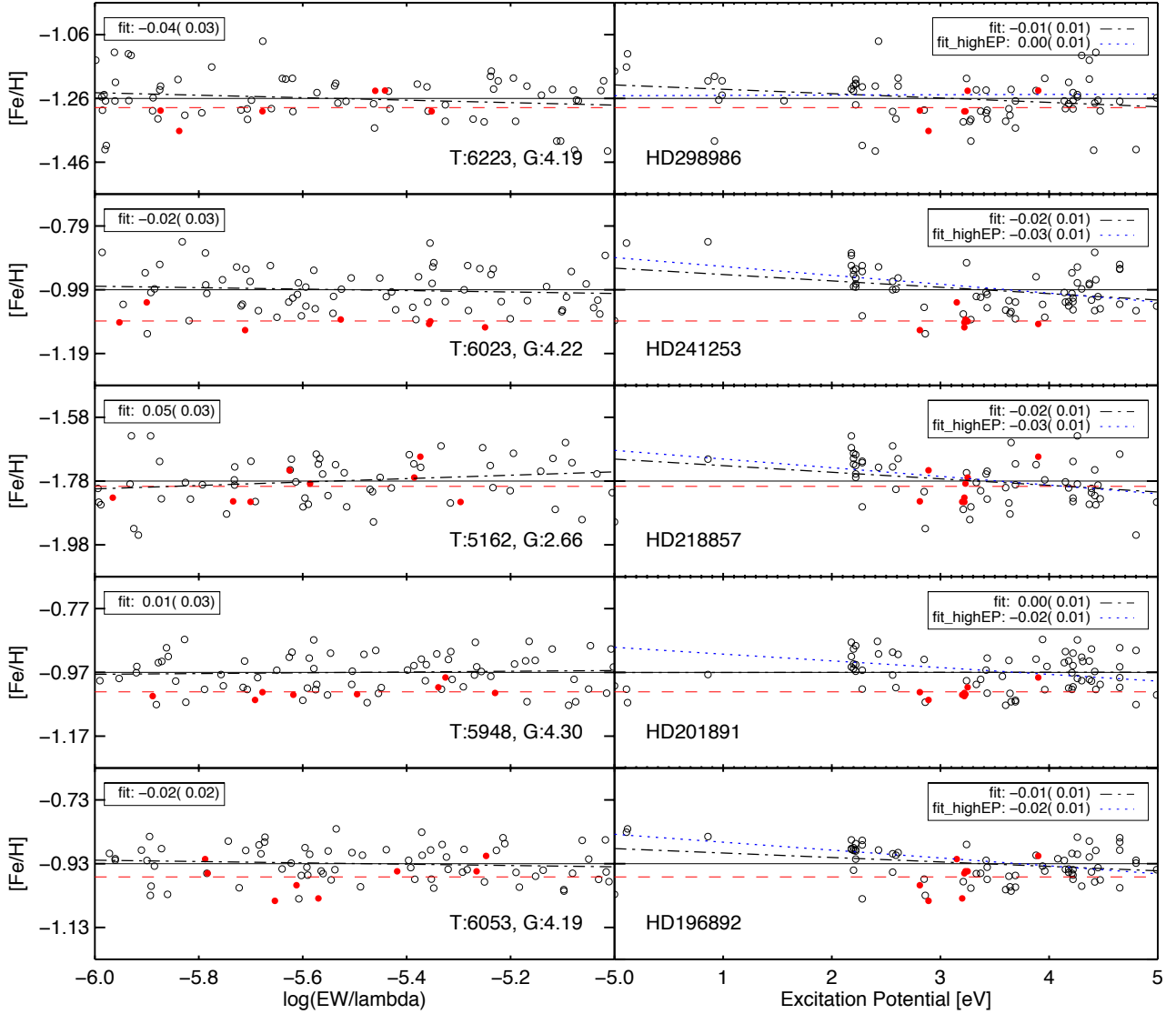
Fig. 7. Final iron abundances as a function of REW (left panels) and EP (right panels) for the remaining five stars (HD 196892, HD 201891, HD 218857, HD 241253, HD 298986) analysed in this work. Symbols used are the same as in Fig. 6.
