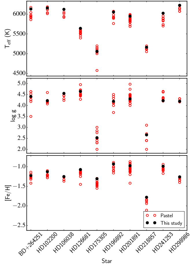
Fig. 3. The adopted T_{\text{eff}} (top panel), \log g (middle panel), and [\text{Fe}/\text{H}] (bottom panel) of the metal-poor GBS candidate stars (black closed circles) compared with the values from the literature (open red circles) sourced from the PASTEL catalogue.
