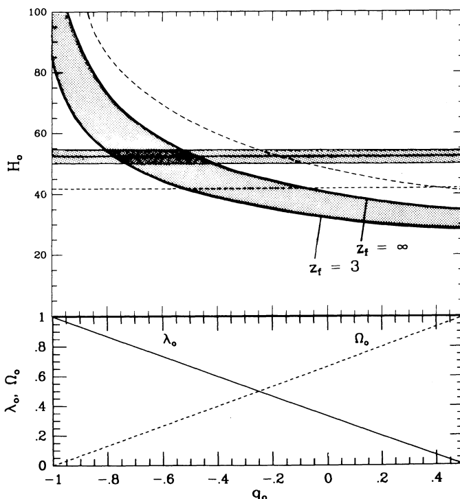
FIG. 5.—Same as Fig. 4 but for the case of a zero-curvature space with \Lambda_0 \neq 0 . See text for discussion about the combined relationship of the different relevant cosmological parameters.
