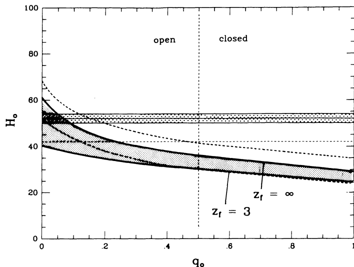
FIG. 4.—Allowed combinations between H_0 and q_0 in a classical Friedmann cosmology as it derives from the fit to the data. The shaded strip is the solution with the redshift for galaxy formation z_f ranging from 3 (lower edge) to \infty (upper edge). An upper 1\sigma envelope is also traced (dashed line). The horizontal strip at H_0 = 52 \pm 2 is the value suggested by Sandage & Tammann (1990) with a lower limit at 42 \text{ km s}^{-1} \text{ Mpc}^{-1} , also reported in the figure. Vertical line separates open and closed models of universe.
