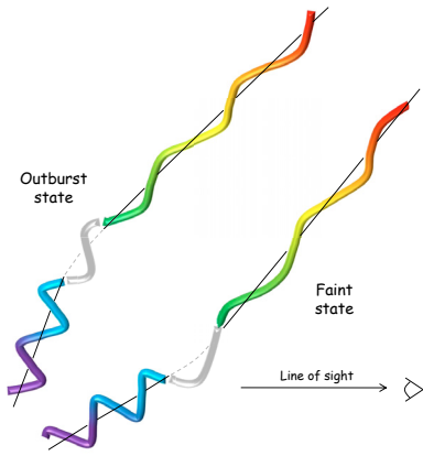
Fig. 10. Sketch of our helical jet model during both the 2008 faint state and the 1997 outburst state. The angle between the jet axis and the line of sight, \psi , has been multiplied by a factor 10 with respect to the values given in Table 4 for clarity. We distinguish the inner region, emitting the high-energy synchrotron plus self inverse-Compton component (purple-blue) from the outer zone, where the low-energy emission component is produced (green-yellow-red).
