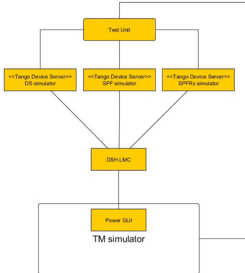
Figure 9: DISH Power Management testing setup
