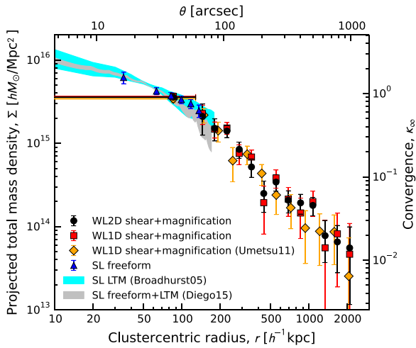
Figure 9. Comparison of projected mass density profiles \Sigma(r) derived from our Subaru 1D weak-lensing analysis (squares; Section 4.1), Subaru 2D weak-lensing analysis (circles; Section 4.2), and free-form strong-lensing analysis of HST data (triangles; Section 5). The cyan shaded area represents the mass profile with 1\sigma uncertainty from a strong-lensing analysis of Broadhurst et al. (2005b) based on the light-traces-mass (LTM) assumption. The gray shaded area shows the strong-lensing results (68% CL) from Diego et al. (2015) using a hybrid scheme combining both free-form grid and LTM substructure components. The diamonds with error bars show the results from our earlier 1D weak-lensing analysis (Umetsu et al. 2011b) based on Subaru Vi' data. Good agreement between the strong and weak lensing results is seen in the region of overlap. There is also good agreement between the different lensing methods and data sets.
