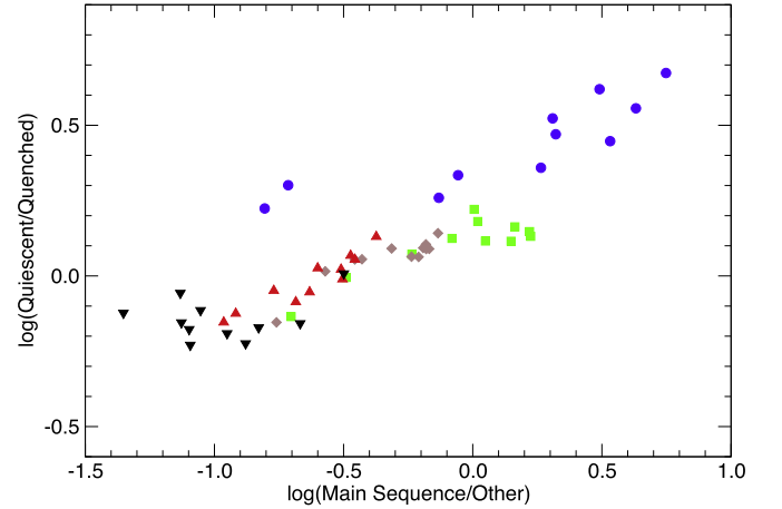
Figure 9. Fraction of main-sequence galaxies vs. the ratio of quiescent to passive galaxies for each data point in Figure 8. Points are labeled by mass range as in Figure 8: blue circles: 9.5–10.0, green squares: 10.0–10.5, brown diamonds: 10.5–11.0, red up triangles: 11.0–11.5, black down triangles: 11.5–12.0.
