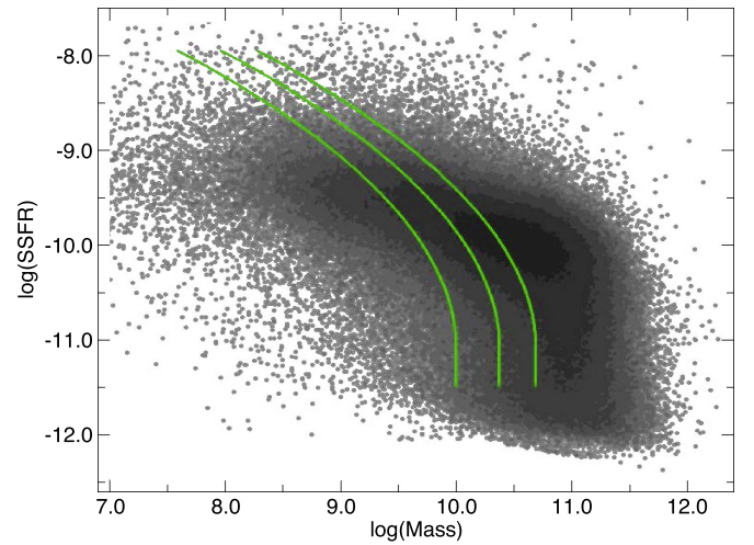
Figure 2. \text{sSFR} vs. mass relation for the entire B04-DR7 sample, using the \text{sSFR} values derived in the Appendix. Superimposed are the median completeness limits at, from left to right, the first through third quartiles of the redshift distribution of the galaxies.
