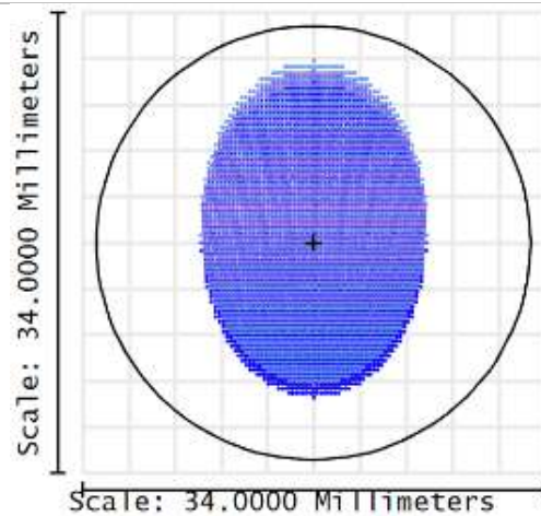
Figure 8: Footprint on CP_TT_VIS.
