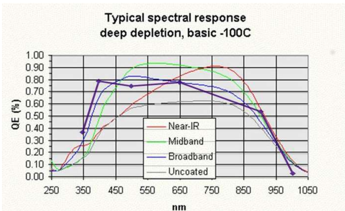
Figure 49: e2v CCD QE
