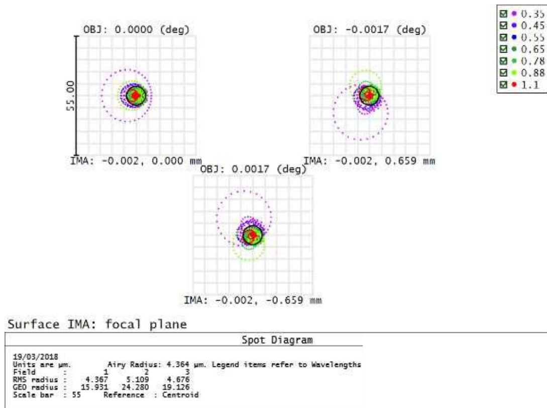
Figure 12: CP-VIS spot diagrams 30° zenith angle.
