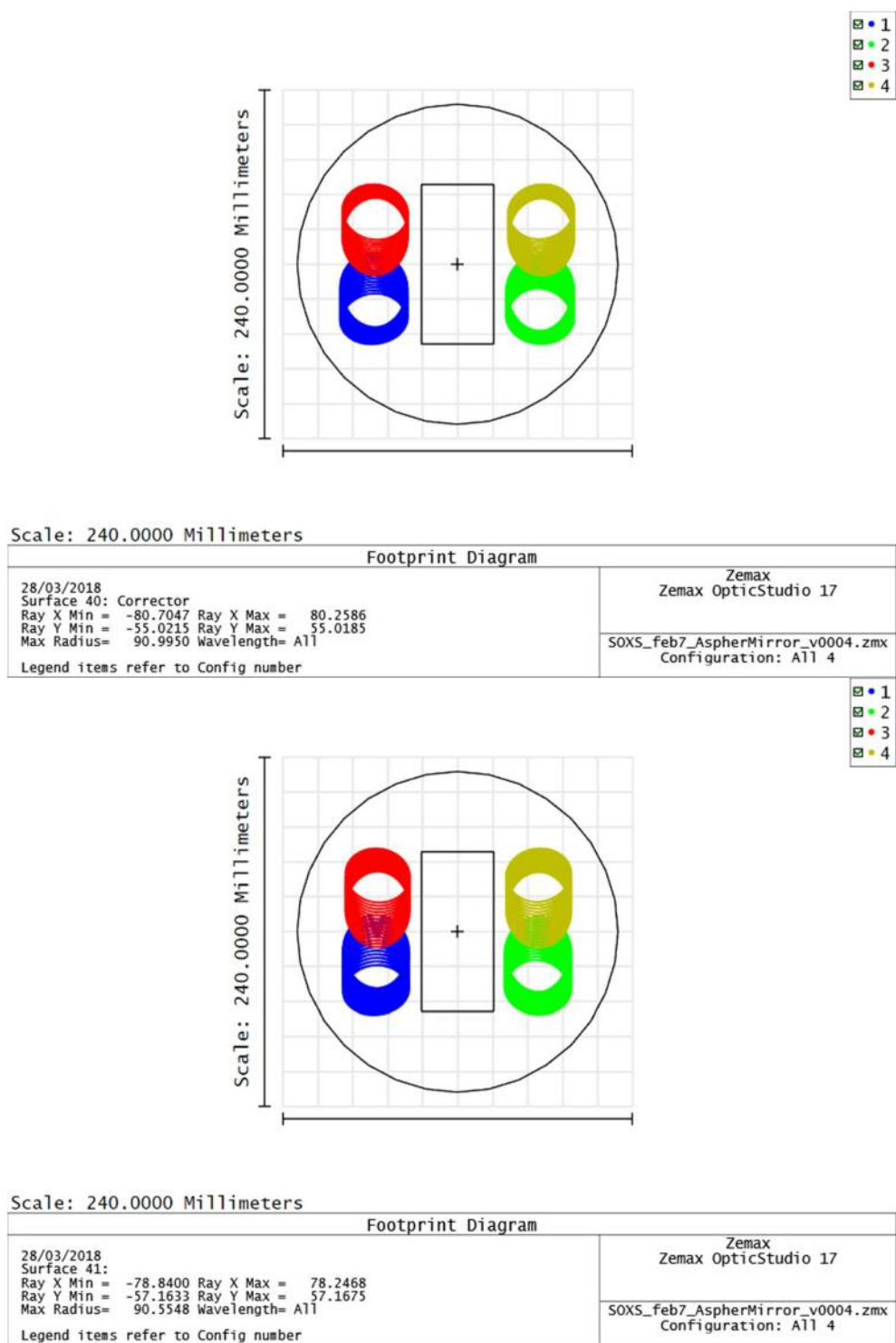
Figure 46: Footprint on the CaF2 corrector entrance (top) and exit (bottom). 1/2/3/4 represent u/g/r/i.
