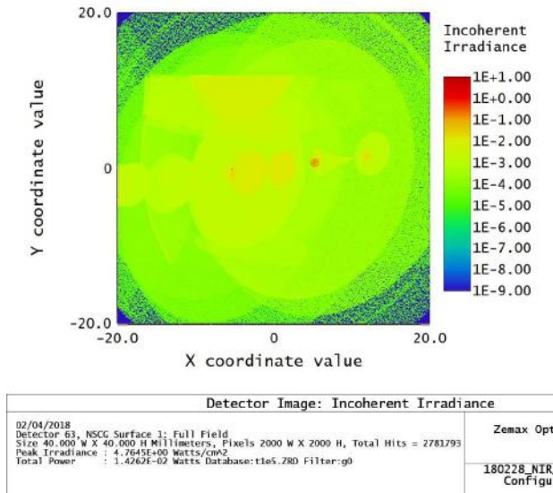
Figure 101: Irradiance due to ghosts only.
