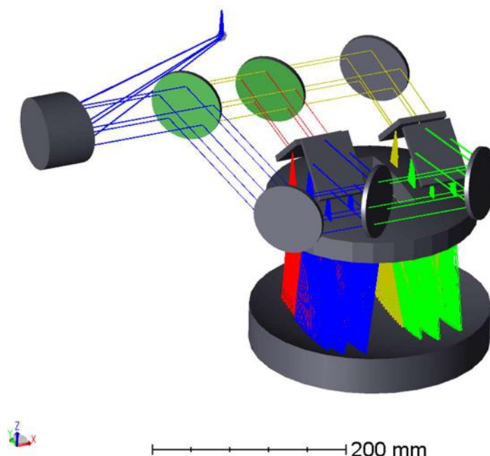
Figure 36: SOXS UV-VIS Spectrograph.
