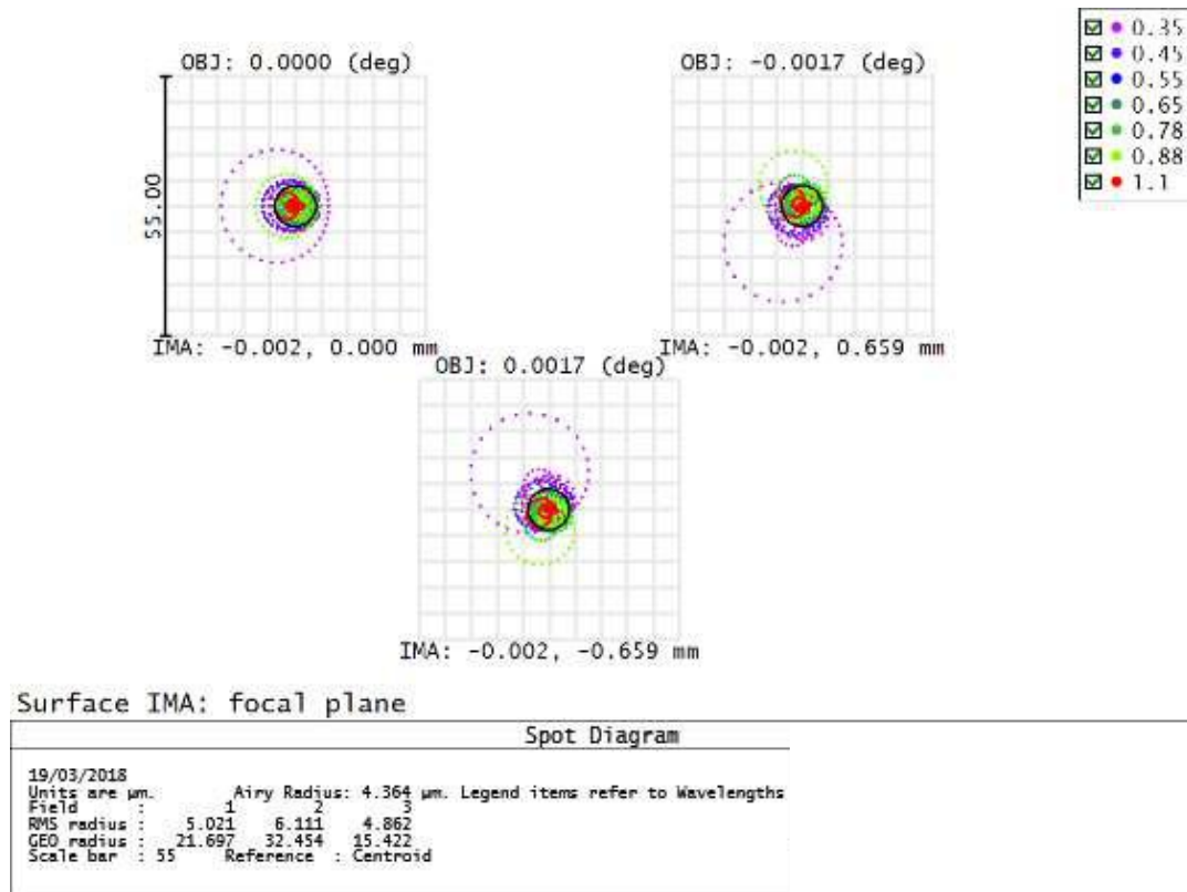
Figure 13: CP UV-VIS spot diagrams 60° zenith angle.
