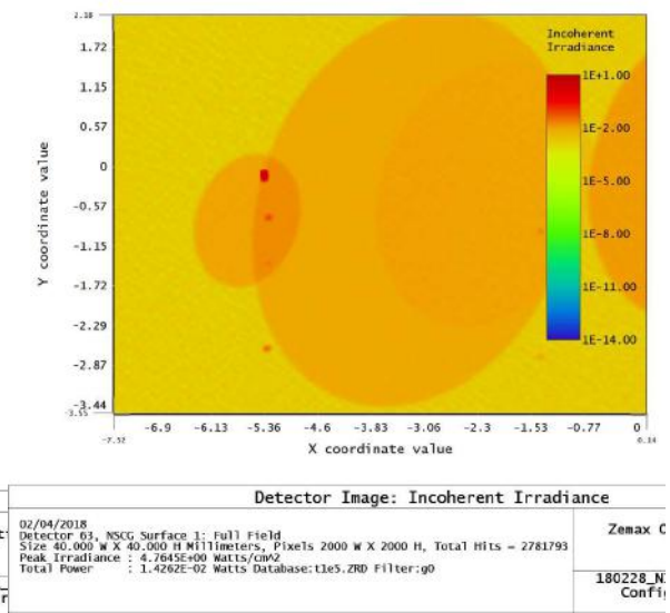
Figure 102: Zoom on pointlike ghosts.
