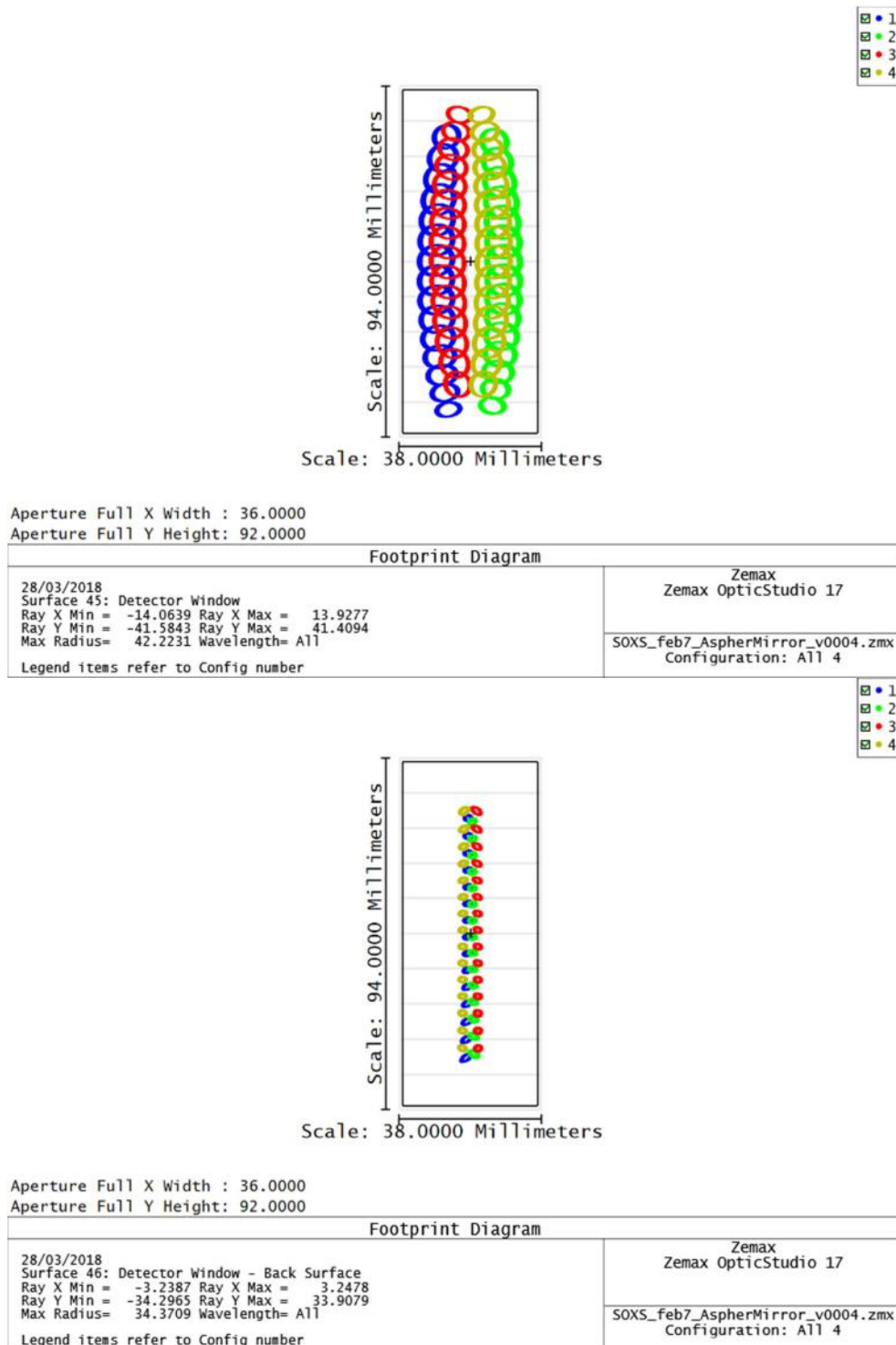
Figure 48: Footprint on the fused silica field flattener entrance (top) and exit (bottom). 1/2/3/4 represent u/g/r/i.
