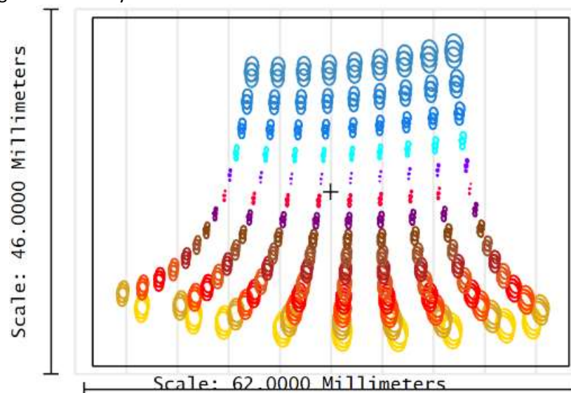
Figure 69: NIR-SM Footprint.
