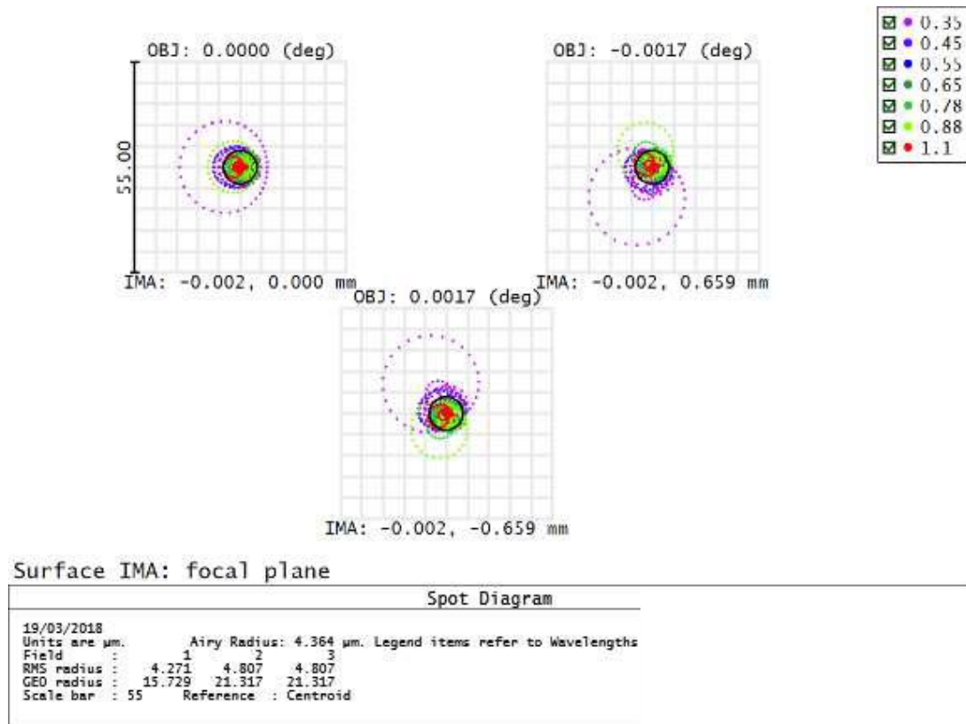
Figure 11: CP UV-VIS spot diagrams 0° zenith angle.
