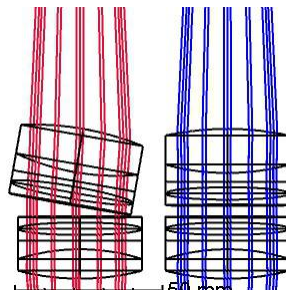
Figure 20: CP UV-VIS ADC1 element, tilted around the X axis passing through the first surface vertex (RED). The BLUE layout is the nominal design.
