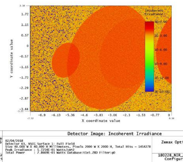
Figure 104: Zoom showing the absence of pointlike ghosts when prisms borders are blackened
