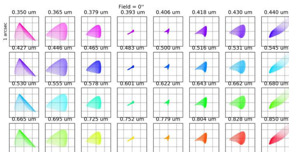
Figure 50: Spot diagram for a field set at the center of the slit. 1 \times 1 arcsec boxes are shown, with the grid representing the pixels ( 15 \times 15 \mu\text{m} ). The wavelength for each spot is written above each box.
