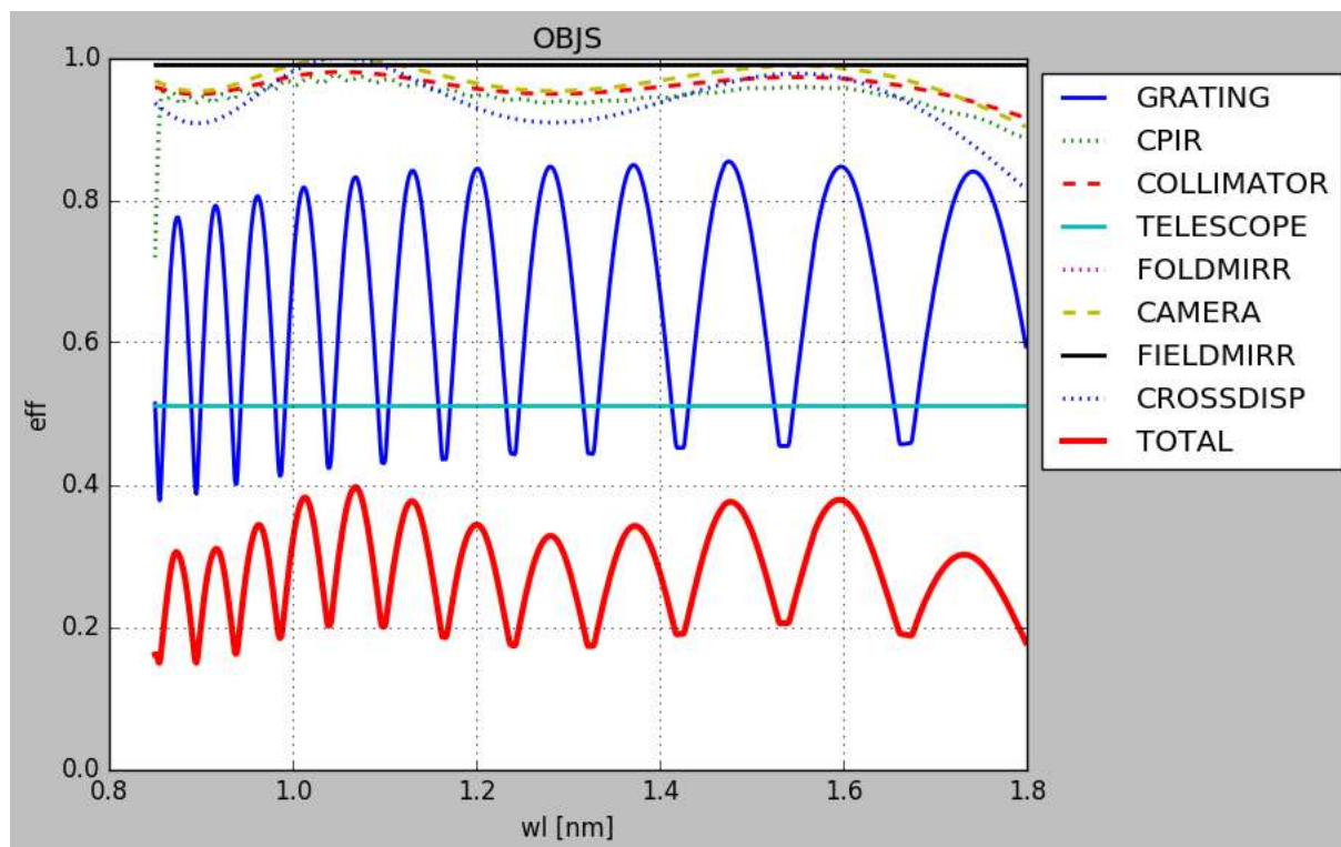
Figure 90: NIR elements efficiencies and total throughput.
