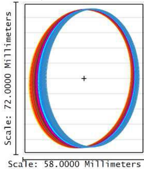
Figure 68: Grating Footprint.
