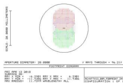
Footprint on Singlet1
