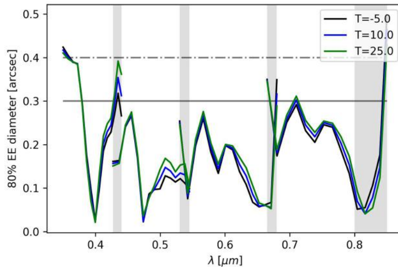
Figure 59: Effect of a 30C temperature change ( -5 to 25^{\circ}\text{C} ) without any compensation.
