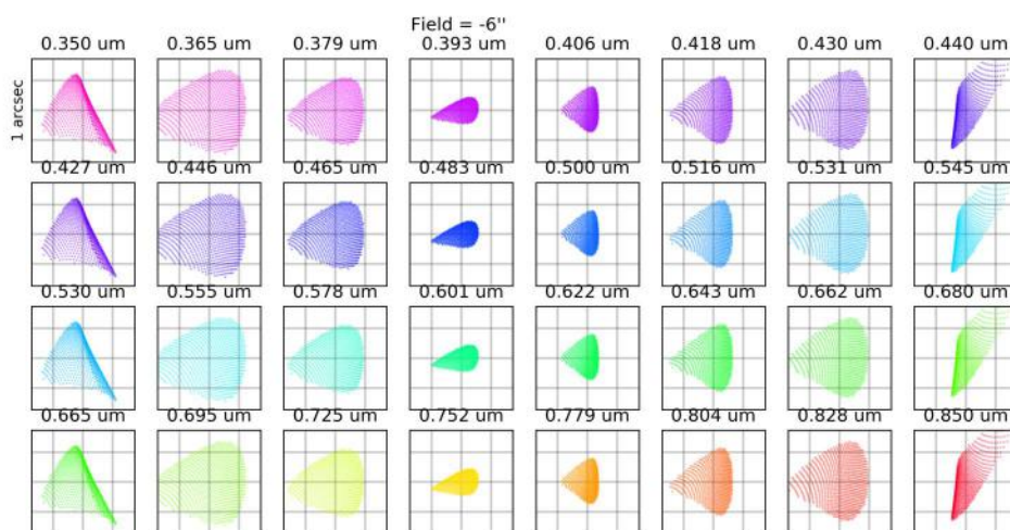
Figure 51: Spot diagram for a field set at the -6 arcsec edge of the slit. 1 \times 1 arcsec boxes are shown, with the grid representing the pixels ( 15 \times 15 \mu\text{m} ). The wavelength for each spot is written above each box.
