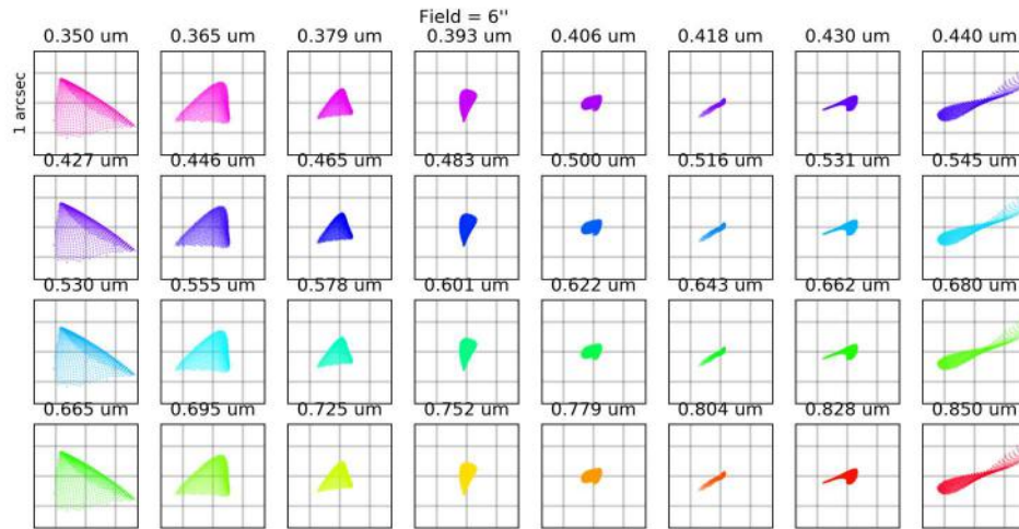
Figure 52: Spot diagram for a field set at the +6 arcsec edge of the slit. 1x1 arcsec boxes are shown, with the grid representing the pixels (15x15μm). The wavelength for each spot is written above each box.
