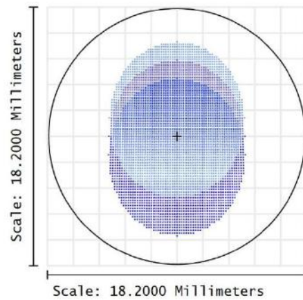
Figure 6: Footprint on CP_FM_VIS.
