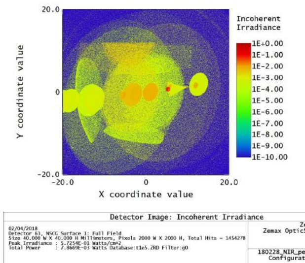
Figure 103: Irradiance due to ghosts using absorbing borders of prisms.
