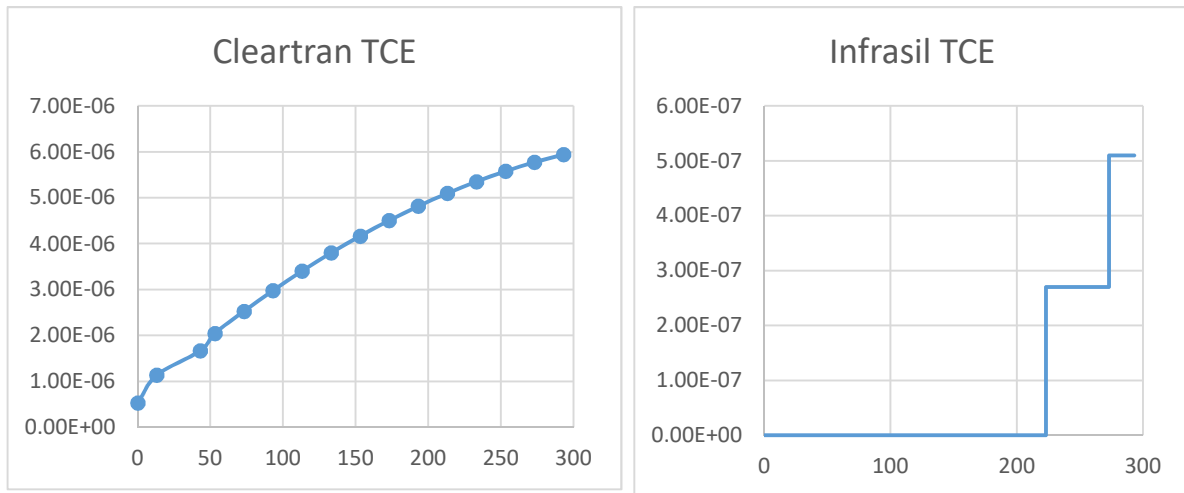
Figure 93: Variation of TCEs of used materials in the considered temperature range.
