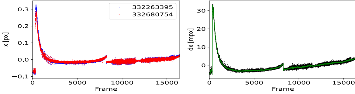
Figure 2. COG estimates on X-axis (left) and difference (right) for target pair {TIC 332263395, TIC 332680754}. Mean values are subtracted, and the filtered data (green line) are superposed to the COG difference.
