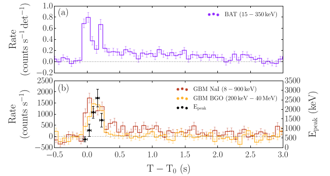
Figure 1. GRB 180618A light curves at 64 ms resolution as detected by the BAT and the GBM instruments. (a) Count rate per enabled detector of the 15–350 keV energy band of the BAT. (b) Count rates of the 8–900 keV energy band of the GBM sodium iodide (NaI) detector, and the 200 keV–40 MeV of the GBM bismuth germanate (BGO) detector. In a different y-axis, we present the evolution of the peak energy ( E_{\text{peak}} ); the values were derived from a cutoff power-law model fit to the 8 keV–40 MeV \nu F_\nu spectrum. In the x-axis, T_0 corresponds to the BAT trigger time.
