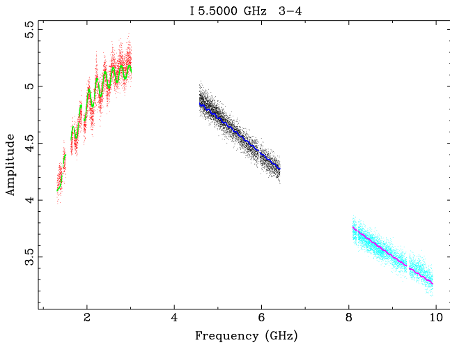
Figure 1. Measured spectrum for PKS 1718-649 from the December 2013 data on a single 415 m baseline, shown with a model fit derived via MIRIAD task uvsfits , as described in the text. Red is the 16 cm (2.1 GHz) band data, with green as model. Black is the 4 cm (5.5 GHz) band data, with dark blue as model. Light blue is the 4 cm (9.0 GHz) band data, with red as model. The data, particularly in the 16 cm band show the beating of the visibility amplitude, indicating a confusing source.
