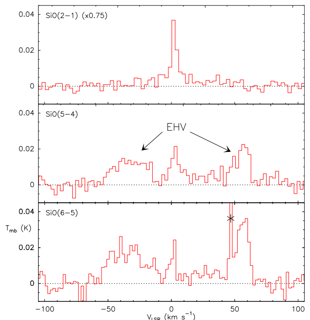
Fig. 2. SiO spectra toward L1157mm (RA(J2000) = 20 h 39 m 06 s .3, Dec(J2000) = 68°02′15″.8). The component near 2.7 \text{km s}^{-1} , most prominent in SiO(2-1), arises from accelerated ambient gas, while the two components labeled “EHV” probably represent a molecular jet. An asterisk in the SiO(6-5) spectrum marks the contribution of ambient c\text{-C}_3\text{H}_2(5_{32}\text{--}4_{41}) .
