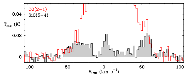
Fig. 6. Spectra of CO(2-1) (red) and SiO(5-4) (gray) toward L1157-mm. Note that the CO (2-1) line, which does not reveal distinct EHV emission, has similar velocity extents as the SiO (5-4) line with the same intensity level.
