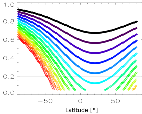
Figure 15 - Percentage of along track (vertical) overlapping wrt latitude of the FOV of a panchromatic filter along an orbit arc during the phase HR1. Values are shown for different repetition times, starting from 3 sec (black curve) and ending with 15 seconds (red curve).
