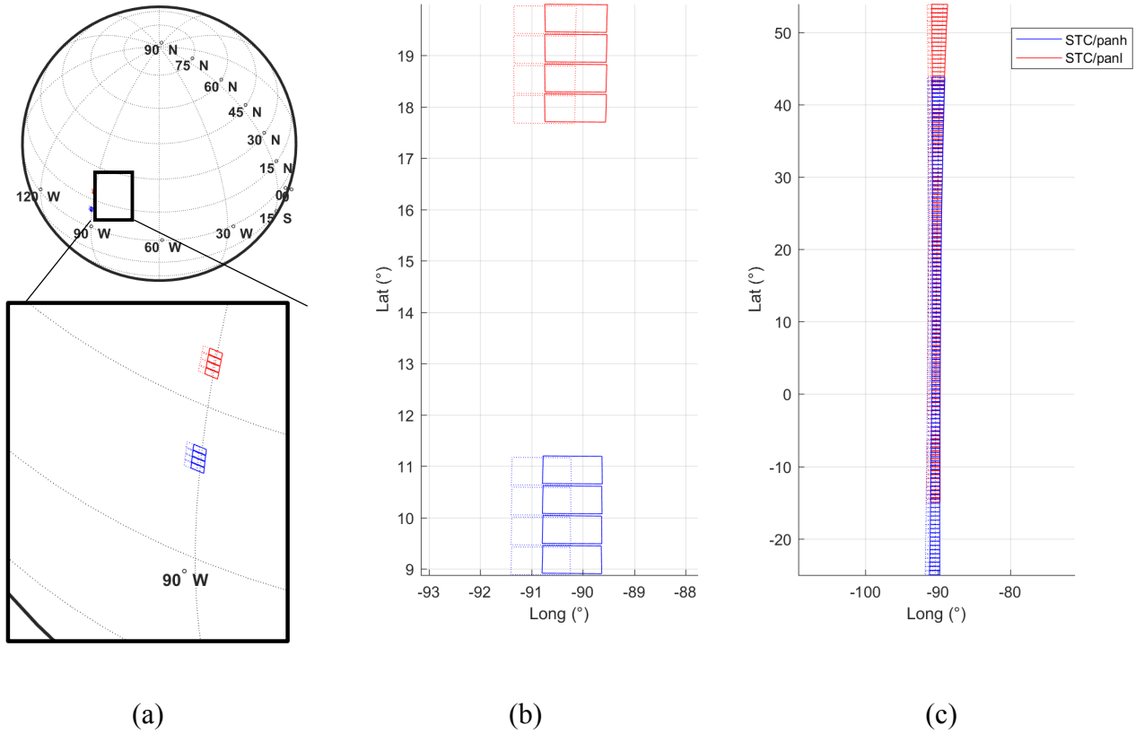
Figure 11 – STC-PANH and PANL FoV projection on the Mercury surface at first aphelion orbit around perihelion (lat. +16°). On-ground projection for 2 consecutive orbits of the footprints of the panchromatic filter of SIMBIOSYS STC -H and -L (respectively in blue and red). Projection on the Mercury sphere in a) and equirectangular projection in b) of 4 consecutive acquisitions with a repetition time of 10 sec (which does not guarantee the along track overlapping). In (c) same simulation as in b), but extended to 10 minutes.
