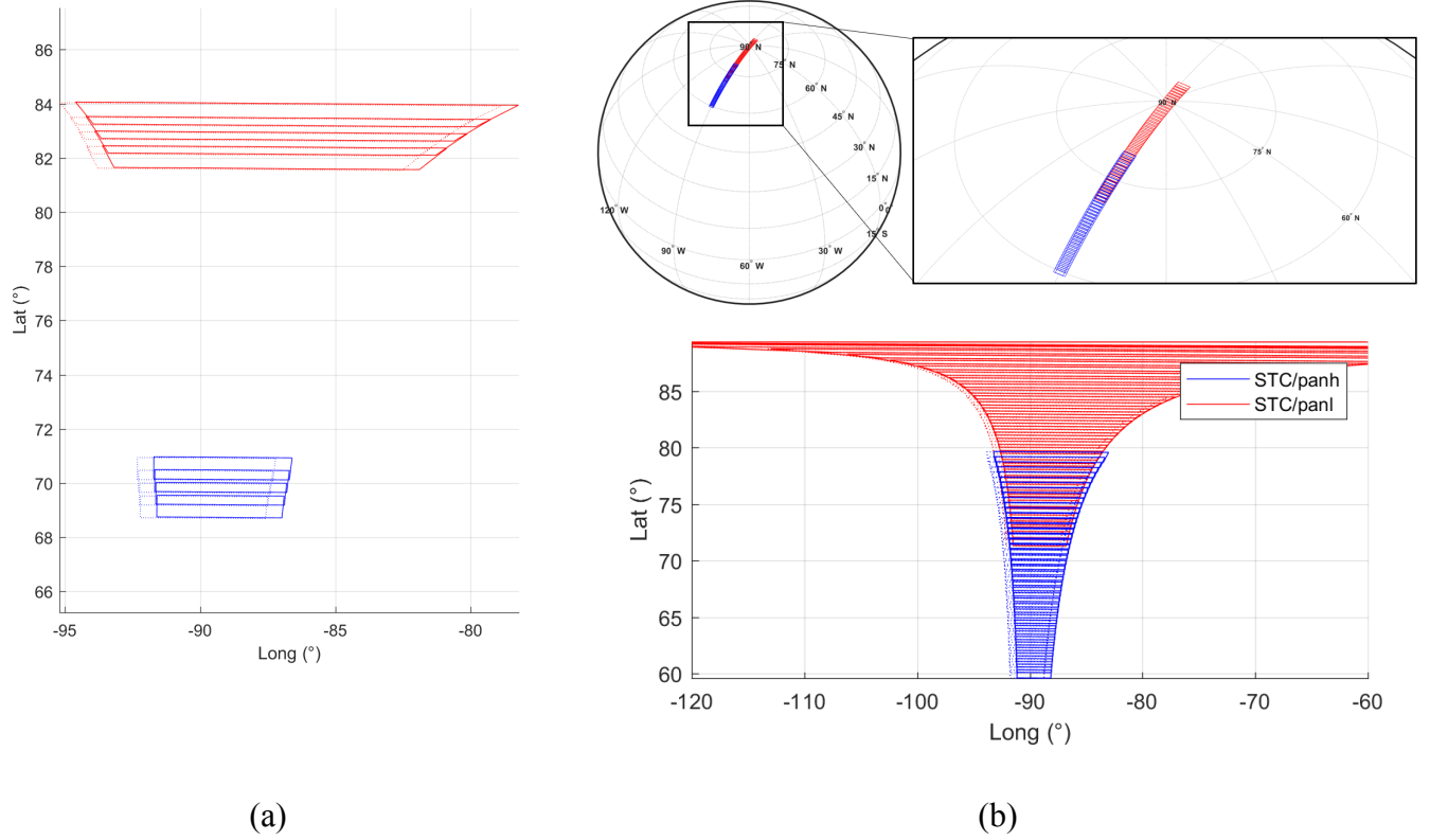
Figure 12 STC-PANH and PANL FoV projection on the Mercury surface at aphelion 0 orbit around sub-nadir latitude +83^\circ (polar region). On-ground FoV projection for 2 consecutive orbits on the surface of Mercury of the panchromatic filters of SIMBIOSYS STC -H and -L (respectively in blue and red). In (a) simulation of 4 consecutive acquisitions with a repetition time of 10 s (which around the poles guarantees the along track overlapping). Cross track overlapping is almost complete. In (b) same simulation but extended to 7 minutes projected on the Mercury sphere (upper images) and with the equirectangular projection (bottom image).
