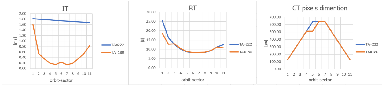
Figure 18 The three plots show the comparison between the 3 main formal parameters (IT, RT, CTdim) for the HR1 aphelion orbit (TA=180°) and the HR1 last bounds orbit (TA=222°) of the same mercury year.
