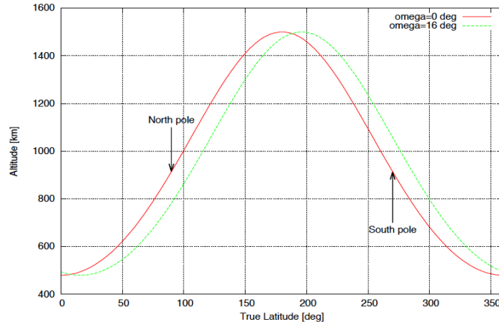
Figure 4 - Variation of MPO altitude with respect to true latitude for a perihelion argument of 16^\circ (green curve, beginning of science phase) and of 0^\circ (red curve, after six months).
