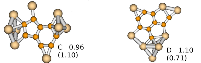
Figure 13. The most stable \text{Si}_9\text{C}_9 clusters and relative energies (in eV).
