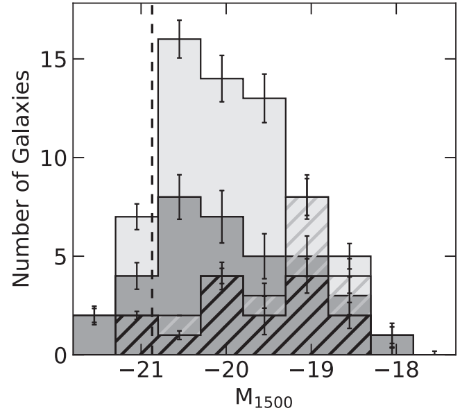
Figure 16. The same as Figure 6 but for M_{1500} . The dashed line indicates the characteristic M_{1600}^* = -20.87 at z = 7 (Bouwens et al. 2015).
