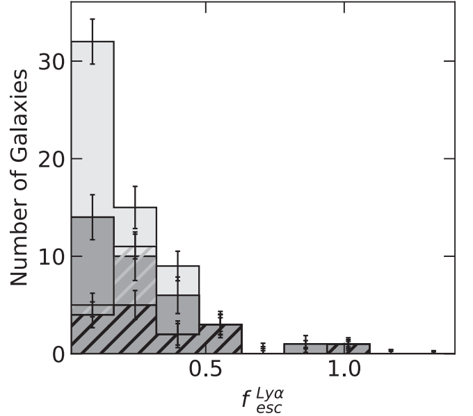
Figure 14. The same as Figure 6 but for f_{\text{esc}}^{\text{Ly}\alpha} .
