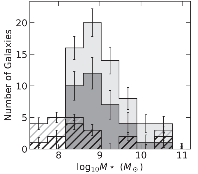
Figure 13. The same as Figure 6 but for M_* .
