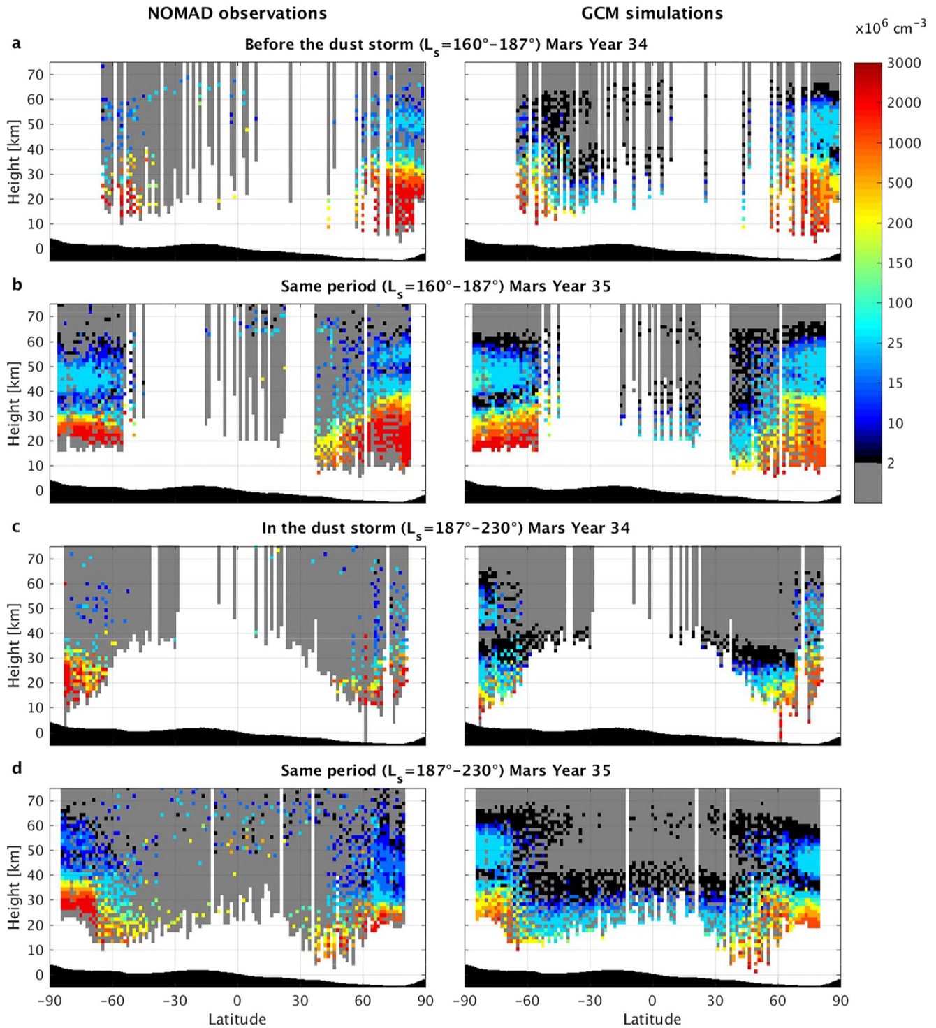
Figure 2. Latitude-height distribution of the ozone ( O_3 ) number density profiles. Panels (a and b) show the average over L_s = 160^\circ – 187^\circ and (c and d) over L_s = 187^\circ – 230^\circ , in MY34 (a and c) and MY35 (b and d). The first period is before the global dust storm (GDS) in MY34, the second period covers the GDS in MY34. Left plots for the O_3 observed by NOMAD/UVIS and right ones from simulations. Gray shading: for the observations, this represents values that were filtered out (see Section 2); for the simulations, values are below 2 \times 10^6 \text{ cm}^{-3} . Height is with respect to the MOLA reference level (black shading shows zonally averaged MOLA topography). A grid of 1.5^\circ in latitude and 1.5 km in height was used to compute the averages. Model results were interpolated to the time and location of the observations.
