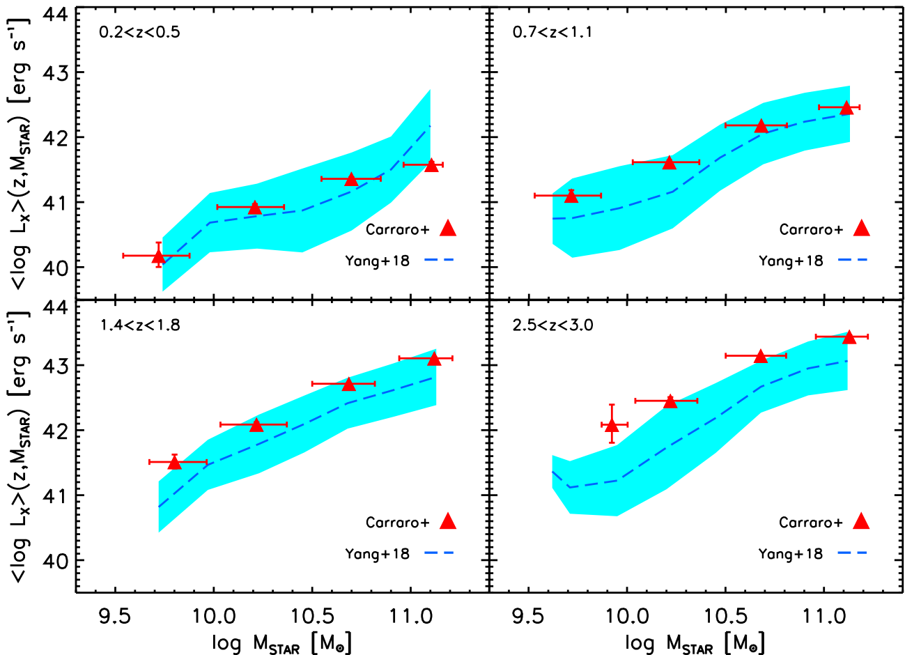
Figure 1. X-ray luminosities, averaged over active and inactive galaxies, as a function of stellar mass and redshift. Data are from Yang et al. (2018) and Carraro et al. (in preparation), as labelled. The cyan region brackets the 1\sigma scatter around the mean.
