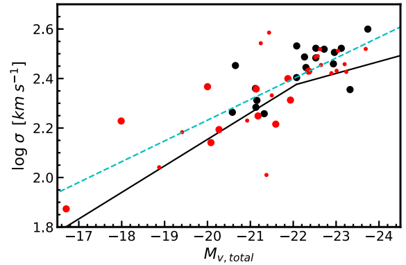
Figure A1. Same layout as fig. 2 in Kormendy (2019). Comparison between the double power-law local \sigma – M_V relation (solid black line) by Lauer et al. (2007) and Kormendy & Bender (2013), with the Kormendy (2019) data set of galaxies with dynamical measurements of their central supermassive black hole mass subdivided into core (black circles) and coreless (red circles) galaxies. The long-dashed, cyan line is a linear fit to the Kormendy (2019) black hole data, proving that at fixed (total) galaxy magnitude M_V , local black holes’ hosts tend to have larger mean velocity dispersions than the underlying population of local galaxies.
