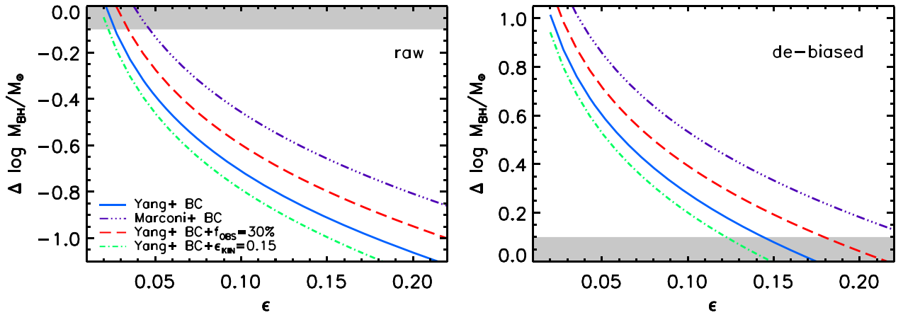
Figure 6. Left: Displacement \Delta \log M_{\text{bh}} between the \log M_{\text{bh}} - \log M_{\text{star}} relations of Kormendy & Ho (2013) and the one inferred from direct integration of the black hole accretion rate. Right: Displacement in \log M_{\text{bh}} between the \log M_{\text{bh}} - \log M_{\text{star}} relations of Shankar et al. (2016a) and the one inferred from direct integration of the black hole accretion rate. The solid blue, long-dashed red, triple dot-dashed purple, and green dot-dashed lines refer, respectively, to models based on the bolometric correction by Yang et al. (2018), on the bolometric correction by Marconi et al. (2004), the bolometric correction by Yang et al. (2018) plus some correction for obscured sources, and on the bolometric correction by Yang et al. (2018) plus a kinetic efficiency of \varepsilon_{\text{kin}} = 0.15 . Higher bolometric corrections or significant obscured fractions require larger radiative efficiencies to reproduce the de-biased M_{\text{bh}} - M_{\text{star}} relation.
