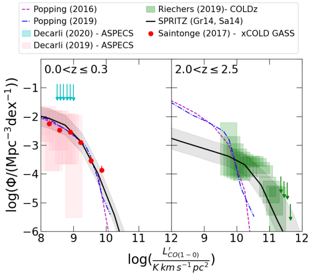
Fig. 5. CO(1–0) LF (solid black lines) derived with SPRITZ, compared with observations by Saintonge et al. (2017, red circles), Riechers et al. (2019, green squares), Decarli et al. (2019, pink squares), and Decarli et al. (2020, cyan arrows as upper limits). The grey shaded area contains the propagated errors of the IR LF and errors in the relations used to derive the CO(1–0) luminosity. We also report the models by Popping et al. (2016, dashed magenta lines) and Popping et al. (2019b, dash-dotted blue line). Gr14 and Sa14 refer to the relations by Greve et al. (2014) and Sargent et al. (2014), respectively.
