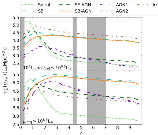
Fig. 4. Contribution to the [CII] luminosity density of the different galaxy populations (see legend) included in SPRTZ. We report two different luminosity ranges: 10^7 L_\odot < L_{[\text{CII}]} \leq 10^{8.5} L_\odot (top) and L_{[\text{CII}]} > 10^{8.5} L_\odot (bottom). The grey shaded areas show the redshift range where observations are available. We highlight that SBs and SB-AGN have sSFRs ranging from \log(\text{sSFR}/\text{yr}^{-1}) = -8.8 to -8.1 , which is above the main sequence at low- z , but on it at z = 5-7 .
