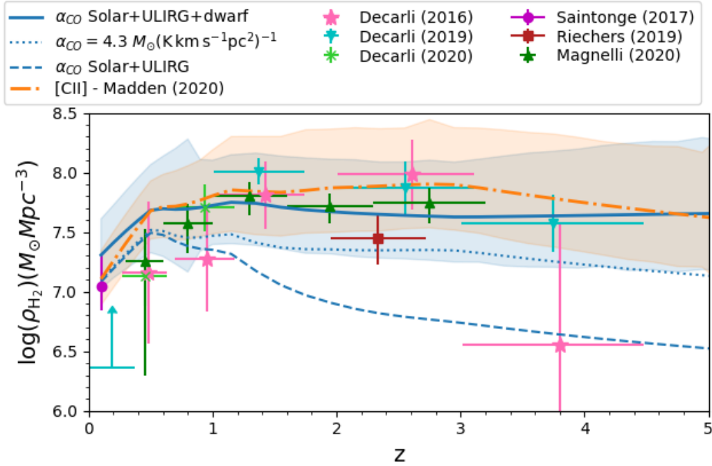
Fig. 8. Molecular gas mass density derived by SPRITZ from [C II], using the [C II] luminosity derived from V15 and the relation by Madden et al. (2020, dash-dotted orange line). We also report the H 2 mass density derived from the CO, using the CO(1–0) luminosity derived from Greve et al. (2014) and Sargent et al. (2014), and considering different \alpha_{\text{CO}} values for star-forming galaxies, ULIRG-like galaxies, and dwarfs (solid blue line). We show the molecular gas mass density obtained by considering a single \alpha_{\text{CO}} value for all the galaxies (dotted blue line), or two different \alpha_{\text{CO}} values for star-forming and ULIRG-like galaxies (dashed blue line). We report observational results by Decarli et al. (2016, 2019, 2020), Saintonge et al. (2017), Riechers et al. (2019), and Magnelli et al. (2020, from the evolution of the dust mass density). The shaded areas include the 1\sigma uncertainties on the input LF, the high- z extrapolations, and the H 2 conversions. For the sake of clarity, we report uncertainties only for the results obtained from [C II] and from CO, assuming three different \alpha_{\text{CO}} values for star-forming galaxies, ULIRG-like galaxies, and dwarfs. The uncertainties associated with other results derived from CO, under different \alpha_{\text{CO}} assumptions, are comparable.
