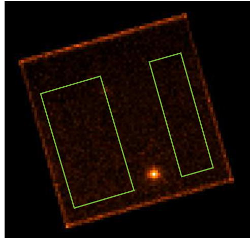
Fig. 1.— Small-window EPIC-pn image corresponding to the 2006 data of the Double Pulsar (first XMM-Newton orbit). The bright spot indicates the target, while the green rectangles show the areas selected to extract the background spectrum.
