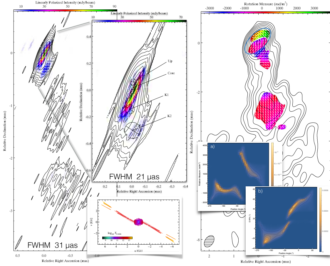
Figure 4: Left: RadioAstron images of BL Lac at 1.3 cm from November 11, 2013. Total intensity is shown in contours, linearly polarised intensity in color scale, and white bars indicate the EVPAs. The inset panel shows the uv-coverage. Right shows the rotation measure map and a) two-dimensional histograms of the rotation measure and b) Faraday-corrected EVPA in the core area. For details see figures in Gómez et al. [49].
