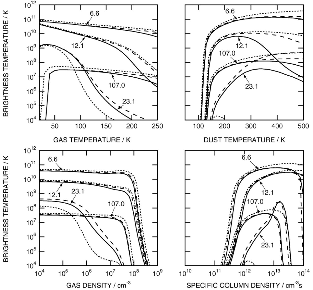
Figure 9: Effect of parameter (gas and dust temperature, gas and specific column density) variations on the brightness temperature of four different methanol masers. The four curves are labelled with the frequency of the maser transition to which they refer: 6.6, 12.1, 23.1 and 107 GHz (reproduced from Fig. 2 in Cragg et al. [19]).
