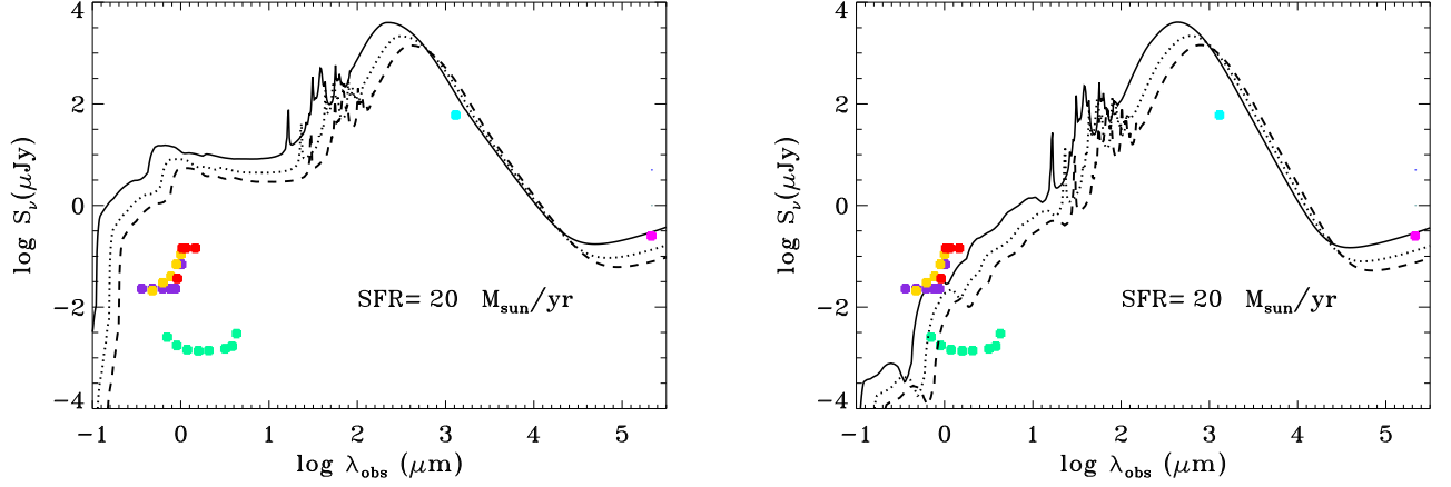
Figure 15. Left panel: Detection limits of deep optical/near-IR surveys (left) and of the deepest SKA1-MID survey (magenta symbol on the right) compared with the spectral energy distribution of an UV-bright young galaxy with a \text{SFR} = 20 M_{\odot} \text{ yr}^{-1} at z = 2 (solid), 4 (dotted) and 6 (dashed). We have considered the following surveys (from top to bottom): Euclid deep (red), Subaru HSC ultra-deep (yellow), LSST deep drilling fields (violet) and JWST (green). The cyan point corresponds to the flux density limit of the deepest ALMA maps at 1.1 and 1.3 mm available so far (dot-dashed brown line; Carniani et al. 2015). The SED was computed using the GRASIL package (Silva et al. 1998) for a Chabrier (2003) Initial Mass Function (IMF), a galaxy age of 10 Myr and a metallicity of 0.1 Z_{\odot} . Right panel: same as the left panel but for an obscured SED with the same IMF and SFR, a galactic age of 1 Gyr and a metallicity of 3 Z_{\odot} .
