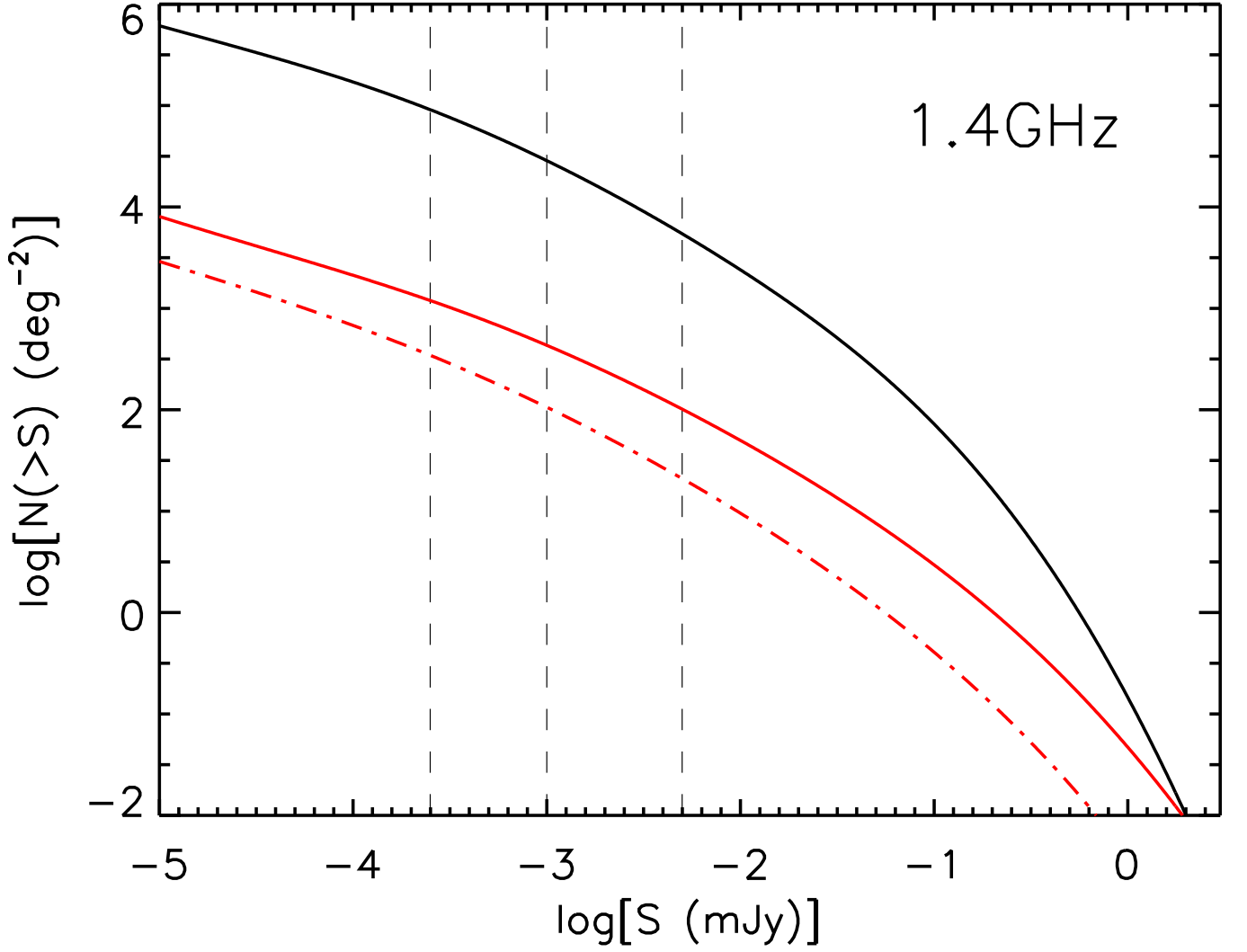
Figure 13. Predicted integral number counts of proto-spheroids at 1.4 GHz. The solid black curve represents the un-lensed counts. The red curves represent the counts of strongly lensed galaxies as a function of the total (sum of all images) flux density (solid) and of the flux density of the fainter of the two images (dot-dashed). The vertical lines represent the three SKA1-MID 5\sigma detection limits for unresolved sources (i.e 0.25\ \mu\text{Jy} , 1\ \mu\text{Jy} , 5\ \mu\text{Jy} ).
