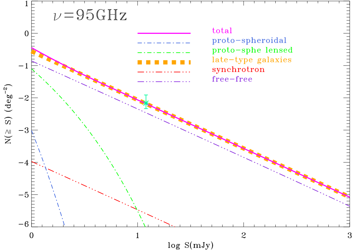
Figure 6. Our re-assessment of the integral counts of dusty galaxies at \nu=95 GHz (asterisks with error bars) compared with the expectations from the Cai et al. (2013) model, using for each source populations the complete SEDs that include dust, synchrotron and free-free emissions. The various lines correspond to the contributions from the different source populations and from the different emission processes, identified in the legend inside the figure.
