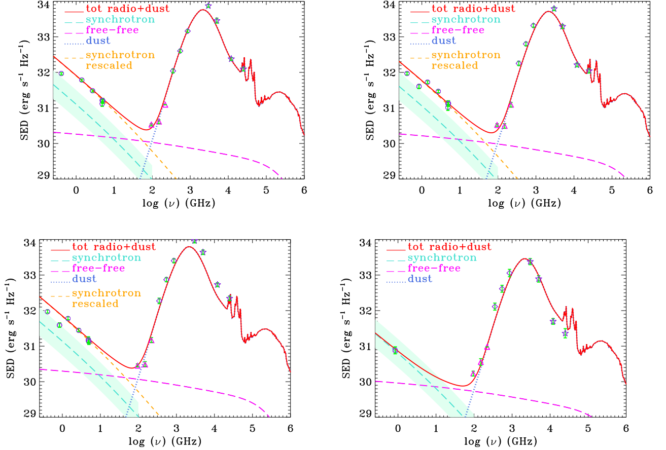
Figure 5. SEDs of 95 GHz selected dusty galaxies in the SPT sample by Mocanu et al. (2013): SPT-SJ041736-6246-8 (top left), SPT-SJ041959-5456-2 (top right), SPT-SJ044540-5914-7 (bottom left), SPT-SJ213629-5433-4 (bottom right). The red curve is a fit made by eye summing the Cai et al. (2013) SED of a cold late-type galaxy (dotted blue line), chosen because the 4 galaxies are all normal disc galaxies, with the free-free emission given by eq. (5) for the same SFR (long-dashed magenta line) and with the synchrotron emission matching the low frequency data. For three of the galaxies, such synchrotron emission (short-dashed orange line) is higher than that given by eq. (3), represented by the long-dashed green line. The difference is about twice the dispersion of the relation between the synchrotron luminosity and the SFR (shaded green band; see sub-sect. 3.1), yet within the range of values for star-forming galaxies according to Yun, Reddy & Condon (2001). It may thus be not statistically significant, especially taking into account a possible selection effect: the higher synchrotron luminosity helps bring the sources above the detection limit at 95 GHz. However, we cannot rule out alternative explanations such as an additional contribution from a weak active nucleus or excess radio emission arising from radio continuum bridges and tidal tails not associated with star formation, similar to what is observed for so-called “taffy” galaxies (Condon et al. 2002; Murphy 2013). Data points: low frequency radio flux densities from the NED (open circles); SPT flux densities (triangles); Planck flux densities (open diamonds); IRAS flux densities (open stars).
