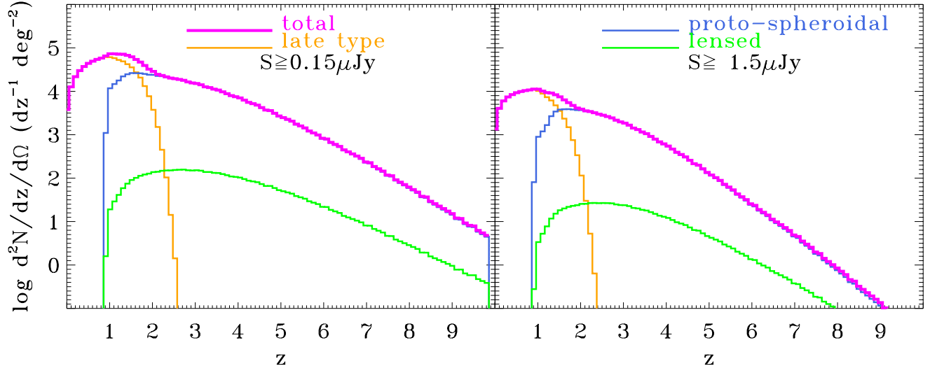
Figure 11. Predicted redshift distributions at the 5\sigma detection limits of SKA1-MID 10 GHz surveys (see text). The lines show the contributions of the various galaxy populations: late-type galaxies (yellow); unlensed proto-spheroidal galaxies (blue); strongly lensed proto-spheroidal galaxies (green); the magenta line shows the total.
