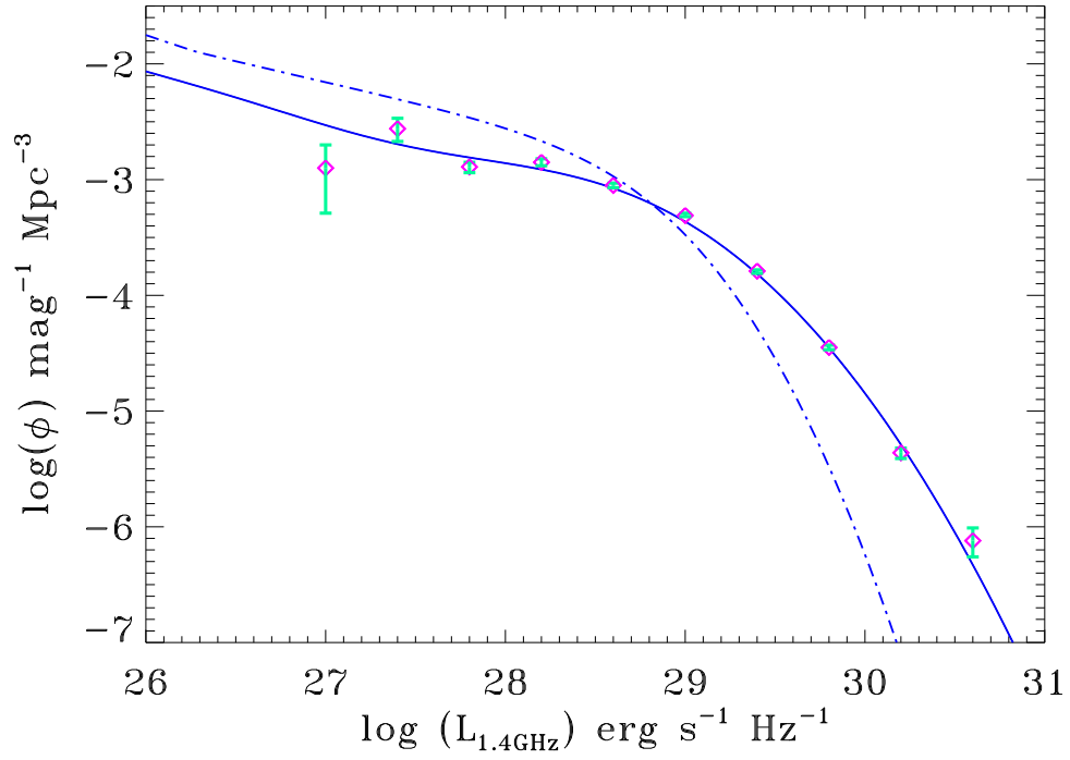
Figure 4. Synchrotron luminosity function of local star-forming galaxies derived from the local SFR function using the non-linear L_{\text{radio}} –SFR relation (cf. eq. 4) and a dispersion of \sigma_{\text{radio}} = 0.4 dex around the mean relation, compared with the observational determination by Mauch & Sadler (2007). The luminosity function obtained assuming a simple proportionality between L_{\text{radio}} and the SFR [eq. (3)] is also shown for comparison (dot-dashed line). The dispersion \sigma_{\text{radio}} raises the bright portion of the luminosity function while eq. (4) flattens the faint part.
