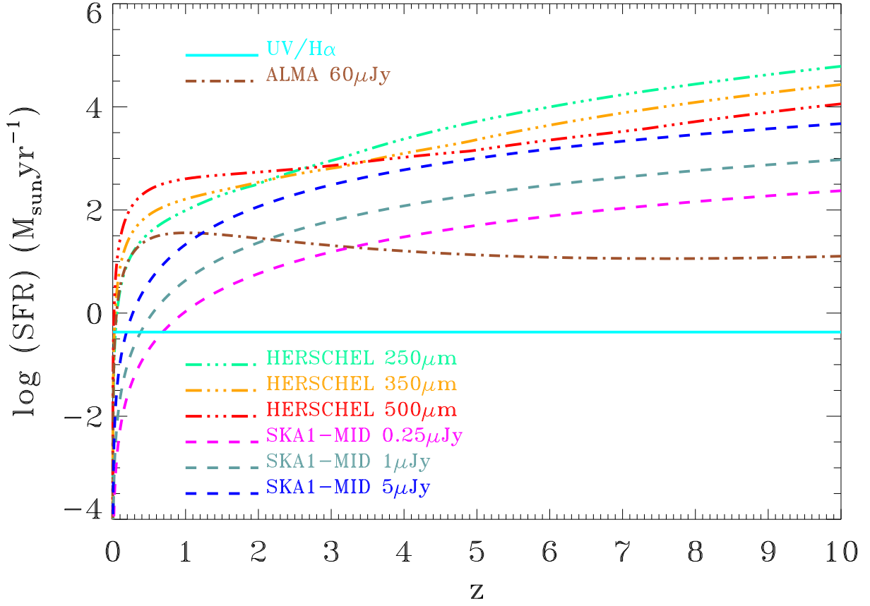
Figure 12. Minimum SFR detectable by SKA1-MID surveys 1.4 GHz down to 0.25 \mu\text{Jy} (dashed magenta line), 1 \mu\text{Jy} (dashed bottle green line) and 5 \mu\text{Jy} (dashed blue line), as a function of z , compared with the minimum SFR detected by Herschel /SPIRE surveys, basically down to the confusion limits (dashed-dot-dot-dot lines, green for 250 \mu\text{m} , orange for 350 \mu\text{m} and red for 500 \mu\text{m} ) and by UV/H \alpha surveys (horizontal cyan line). The latter line corresponds to the average minimum absolute magnitude reached by the deepest surveys, that turns out to be almost independent of redshift. Note that, while very deep in terms of SFR, the UV/H \alpha surveys miss the dust-enshrouded star formation. Also shown, for comparison, is the minimum SFR detectable in the deepest ALMA maps at 1.1 and 1.3 mm available so far (dot-dashed brown line; Carniani et al. 2015).
