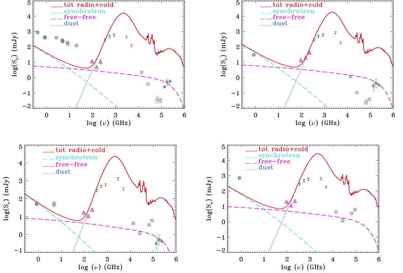
Figure 7. SPT sources selected at 95 GHz that have 1 > P(\alpha_{220}^{150} > 1.5) > 0.6 : SPT-SJ043651-5841-1 (top left), SPT-SJ203730-6513-3 (top right), SPT-SJ204101-5451-4 (bottom left), SPT-SJ213406-5334-3 (bottom right). Their SEDs are incompatible with those of star-forming galaxies, illustrated by the solid red line, and consistent with being radio sources. Data points: low frequency radio flux densities from the NED (open circles); SPT flux densities (triangles); WISE flux densities (open squares); 2MASS flux densities (spirals); in violet and dark green are IRAS and Planck upper limits, respectively. We have adopted as Planck upper limits the 90% completeness limits of the Planck Catalogue of Compact Sources (Planck Collaboration XXVIII 2014) in the “extragalactic zone”.
