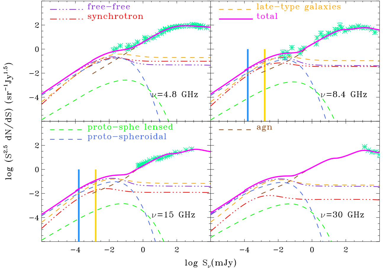
Figure 9. Predicted versus observed counts at 4.8, 8.4 and 30 GHz. Dusty galaxies come up at sub-mJy flux density levels and their counts are accounted for by the model. At higher flux densities the counts are dominated by canonical, AGN powered radio sources. The models shown are from Massardi et al. (2010) at 1.4, and 4.8 GHz and from de Zotti et al. (2005) at 8.4 and 30 GHz. The various lines correspond to the contributions from the different source populations (dashed yellow lines: late-type galaxies; dashed blue lines: unlensed proto-spheroidal galaxies; dashed green lines: strongly lensed proto-spheroidal galaxies; dashed brown lines: radio-loud AGNs; solid magenta line: total) and from the different emission processes (triple-dot dashed lines, red for synchrotron, violet for free-free). The solid vertical lines indicate the predicted flux density limits, for unresolved sources, of possible deep (yellow) and ultra-deep (blue) band 5 surveys with SKA1-MID.
