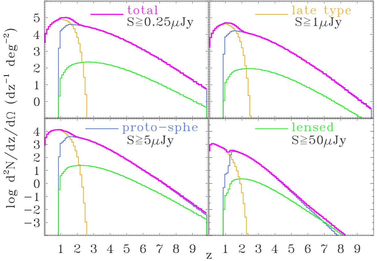
Figure 10. Predicted redshift distributions at the 5\sigma detection limits of the deepest SKA1-MID, of the MIGHTEE (MeerKAT) and of the EMU (ASKAP) 1.4 GHz surveys (see text). The lines show the contributions of the various galaxy populations: late-type galaxies (yellow); unlensed proto-spheroidal galaxies (blue); strongly lensed proto-spheroidal galaxies (green); the magenta line shows the total.
