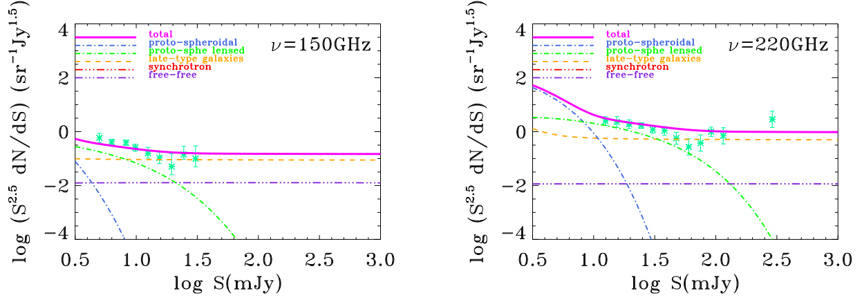
Figure 8. Euclidean normalized differential counts of dusty galaxies at 150 and at 220 GHz (left and right panel, respectively). The asterisks with error bars are the observational determinations by Mocanu et al. (2013). The various lines correspond to the contributions from the different emission processes and from the different galaxy populations, identified in the legend inside the panels. The lines corresponding to the synchrotron emission are below the lower limit of the y-axis. Note that in the considered flux density ranges the counts of star-forming galaxies seen via their radio emission are made by nearby sources and have thus an Euclidean slope. On the contrary, counts due to unlensed and lensed proto-spheroidal galaxies, seen via their dust emission, are due to strongly evolving high- z objects.
