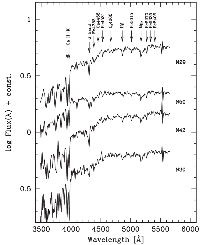
Figure 11. Spectral energy distribution for the four galaxies observed at Casleo. For easier reading, spectra have been degraded here to a resolution of 12 Å FWHM and corrected for redshift. The Ca H+K absorption lines, together with all the main spectral features included in the Lick narrow-band index system (see Table 8), are marked at the top.
