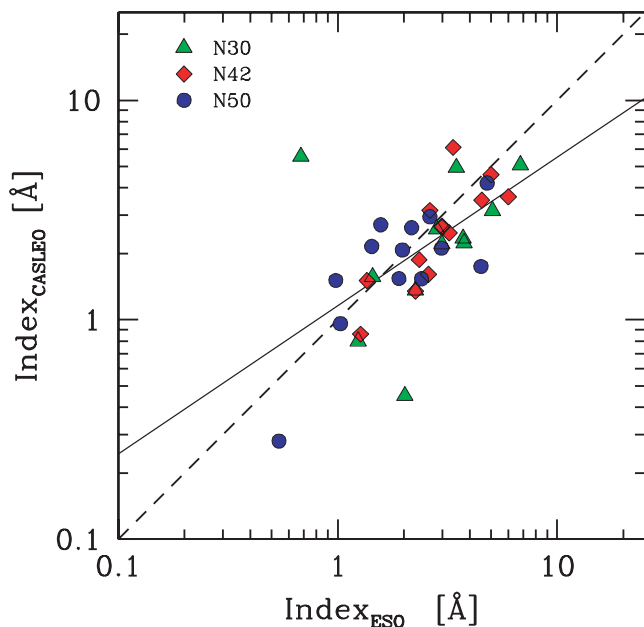
Figure 14. The set of Lick indices of Table 8 for the three galaxies in common between ESO and Casleo observations (namely, N30, N42 and N50). Due to a poorer spectral resolution ( 10 \text{ \AA} FWHM), the Casleo spectra show slightly ‘shallower’ spectral features (and correspondingly lower indices) compared with the ESO spectra, closer to the Lick standard system. The dashed line in the plot is the one-to-one relation while the solid line is the least-squares fit of the points according to equation (9). For better self-consistency, magnitude indices like Mg_1 and Mg_2 have been converted to pseudo-equivalent widths, as explained in Footnote 11.
