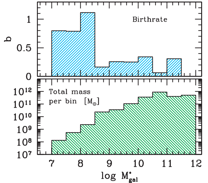
Figure 10. Upper panel: mean birth rate versus galaxy stellar mass, as inferred from the match with the Buzzoni (2005) template galaxy models (see text for the detailed procedure). The total sample of 136 likely member galaxies of Fig. 9 is considered. Note the ‘downsizing’ effect, with low-mass galaxies (of prevailing dSph/Im morphological type) supplying the fresh star formation within the NGC 5044 Group. Fresh stars are produced inside the group at a rate of roughly 23 M_{\odot} \text{ yr}^{-1} , while the bright stellar mass sampled by our observations amounts to M_{\text{gal}}^*(\text{tot}) = \sum M_{\text{gal}}^* = 2.3 \times 10^{12} M_{\odot} . This total is singled out in the lower panel in terms of the cumulative galaxy mass fraction for each mass bin.
