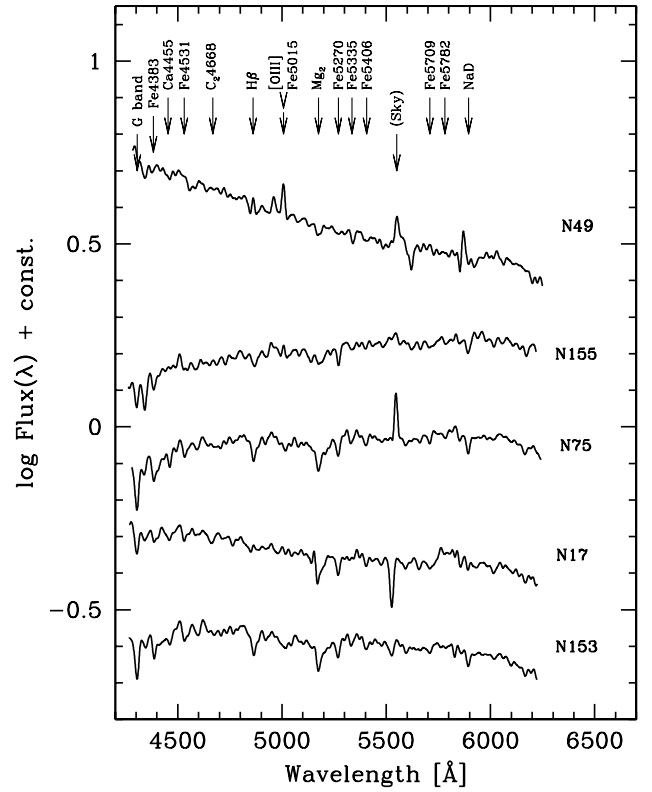
Figure 13. Same as Fig. 11, but for a second set of member galaxies observed at ESO. Note the outstanding H \beta and [O III] 5007 Å emission in Im galaxy N49. For easier reading, spectra have been degraded here to a resolution of 12 Å FWHM and corrected for redshift. Marked at the top are also all the main spectral features included in the Lick narrow-band index system (see Table 8).
