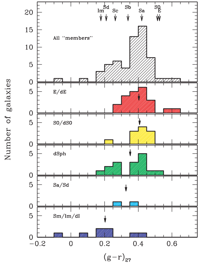
Figure 5. Apparent (g - r) colour distribution of the ESO+Casleo galaxy sample. Only likely members ( m_c codes 1 and 2 of Tables A1 and A2) are considered. These 59 galaxies (upper panel) are disaggregated into the different morphological groups along the different panels, as labelled. Mean colours from the Buzzoni (2005) template galaxy models, matched to the observations according to the Schlegel et al. (1998) reddening estimate, are marked at the top by small arrows. These are to be compared with the mean observed colours of each morphological class (from Table 3), as marked (small arrows in each panel).
