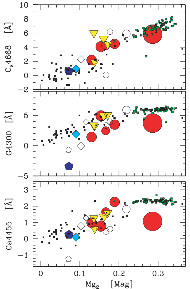
Figure 19. The Lick-gram for the two carbon molecular indices \text{C}_2 and CH (alias the G band at 4300 Å) and for the calcium index Ca 4455 versus \text{Mg}_2 for the 16 ESO galaxies plus N29 from Casleo. Symbols are as for Fig. 16. The Rampazzo et al. (2005) and Annibali et al. (2006) galaxy sample is also overplotted, together with the M31 and Galactic globular cluster data of Trager et al. (1998) (small squares). See text for a full discussion.
