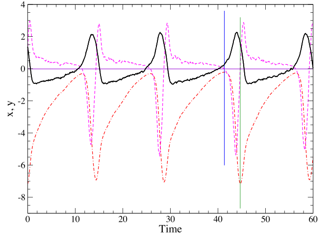
Figure 7. Numerical solutions of the variable y(t) (red dot-dashed curve) and its first derivative (magenta dashed curve) compared with the x(t) (black curve) when in the \rho spiking class. The blue and green vertical lines limit the interval between a maximum and a minimum of y(t) , where it is very quickly decreasing that corresponds to the highest emission in the x(t) peak. The violet horizontal line marks the zero level.
