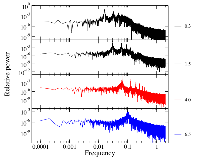
Figure 11. Power-density spectra of the light curves in Fig. 10. The two upper panels correspond to the spiking of the \rho class, while the third panel (red curve) is that of the ‘hfo’. All these spectra are dominated by the narrow lines and their harmonics of the periodic signals. The blue spectrum in the last panel has a unique broad peak typical of a QPO.
