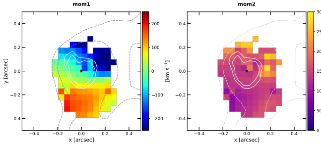
Fig. 5. Moment 1 and moment 2 maps for the component of the [OIII]λ5007 line emission tracing gas in the host galaxy (see text). The contours are the same as in Fig. 4. An S/N > 40 threshold has been used to mask lower S/N spaxels and isolate the rotation in the central spaxels. A rotational pattern is suggested by the data that is compatible with the CO(5–4) rotation detected by B18.
