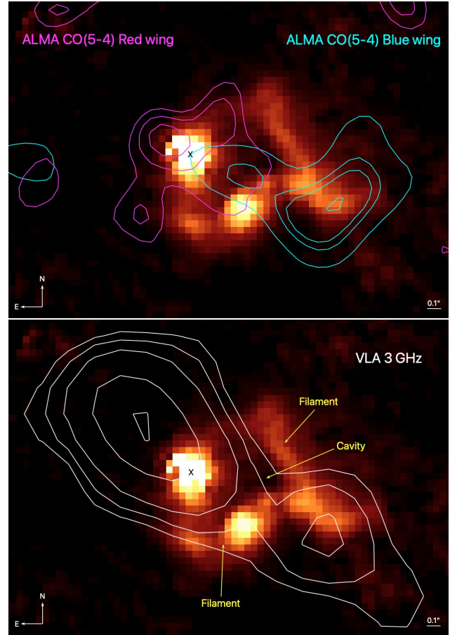
Fig. 8. Channel map of [OIII]λ5007 emission with v < -300 km s ^{-1} with contours of the CO(5-4) molecular blue- (cyan) and redshifted (magenta) outflow components (upper panel, from B18), and 3 GHz radio emission (white) from VLA observations (lower panel, from Vardoulaki et al. 2019). The location of the QSO is marked with a black cross, and the filaments and the cavity are shown with arrows. The VLA radio emission and the blueshifted ionised and molecular outflows appear to be co-spatial, as well as the possible redshifted counterparts.
