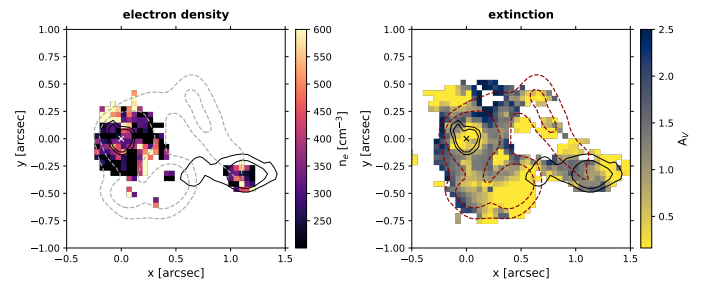
Fig. 6. Electron density map from [SII]λ6716,30 line ratio (left panel) and extinction map from the Balmer decrement H\alpha/H\beta (right panel). The contours used in Fig. 4 are overplotted. Both maps display only the spaxels with at least S/N > 3 in all the emission lines involved, and the QSO location is marked with a cross.
