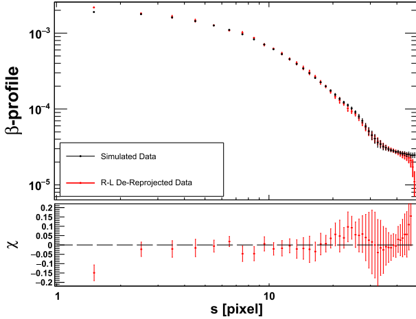
Fig. 8. Top: normalized profiles illustrating the results of the de- and reprojecting of the simulated \beta -profile map rebinned using the Voronoi tessellation with 300 counts/bin. Black: profile of the rebinned initial data maps; Red: profile obtained by de- and reprojecting the initial data maps. These profiles correspond to the azimuthal average of the maps on the left and on the right of Fig. 7, respectively. Bottom: relative residuals computed as in Fig. 3.
