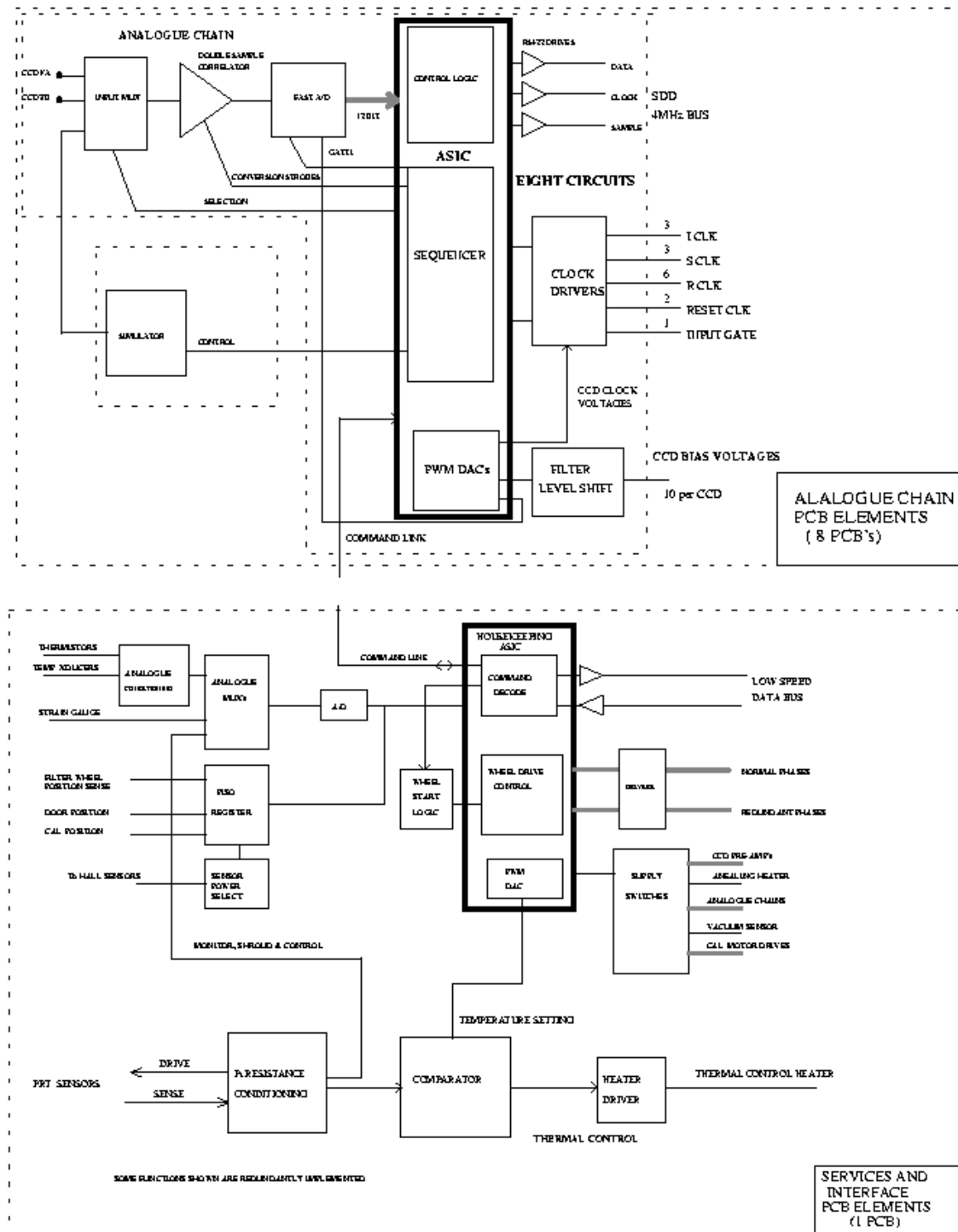
Figure 4.3-1: EMAE Block Diagram
