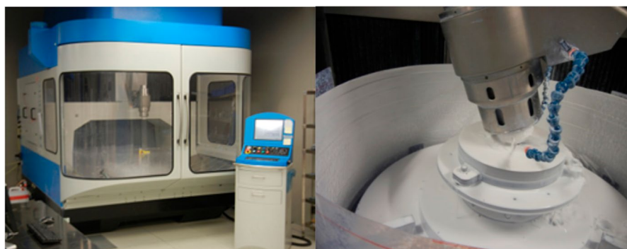
Fig. 4 Pictures of the Zeeko IRP 1200X robotic polishing machine at MediaLario: ensemble view (left) and close up of the spindle while operating (right)
