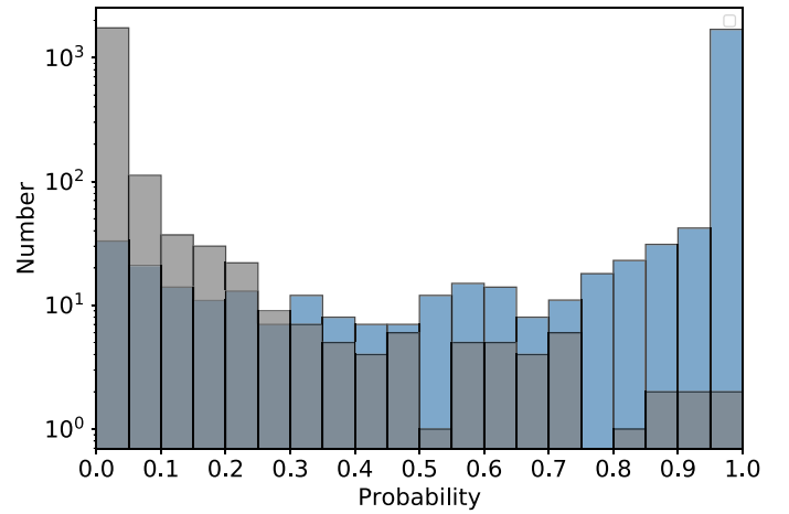
Figure 2. Left: ROC curve for the CNN classifier based on 4000 galaxies in the testing sample. We also show the locations of three different values of the threshold ( p_{\text{CNN}} = 0.25, 0.5 , and 0.75 ) used to calculate the FPR and TPR. Right: probability distribution of the testing sample. The blue histogram represents the probability distribution of the positives, while the gray histogram shows that of the negatives.
