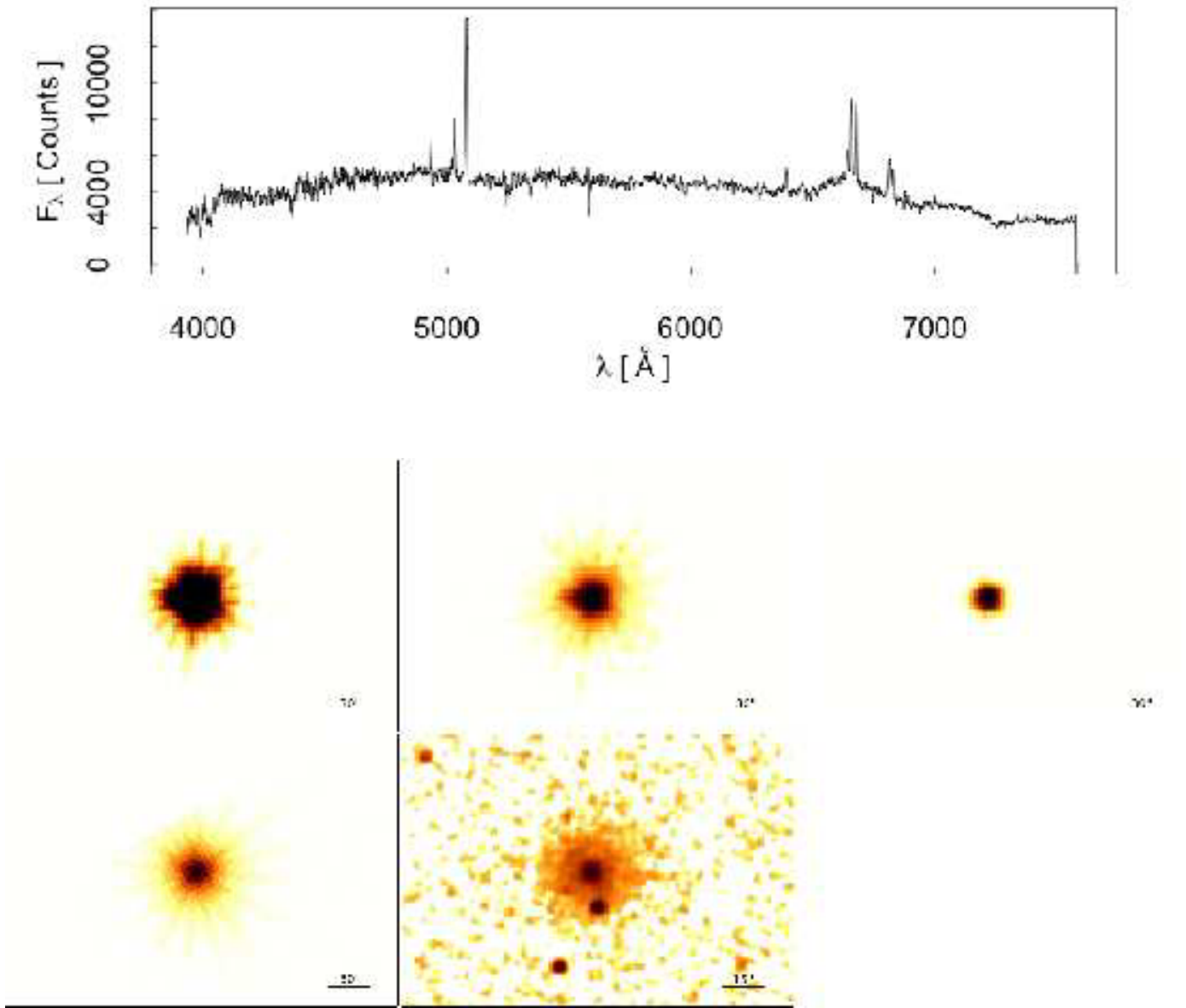
Fig. C.7: Up: Optical spectrum (from NED); bottom: images of NGC 2617. (Top left): Smoothed X-ray 0.6-0.9 keV energy band; (top center): smoothed X-ray 1.6-2.0 keV energy band; (top right): smoothed X-ray 4.5-8.0 keV energy band; (bottom left): X-ray 0.5-10.0 keV energy band without smoothing; (bottom center): 2M SS image in the K_s band.
