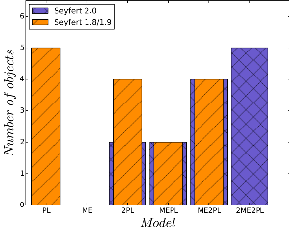
Fig. 2: Histogram of the best fit models for Seyfert 1.8/1.9 and 2.
