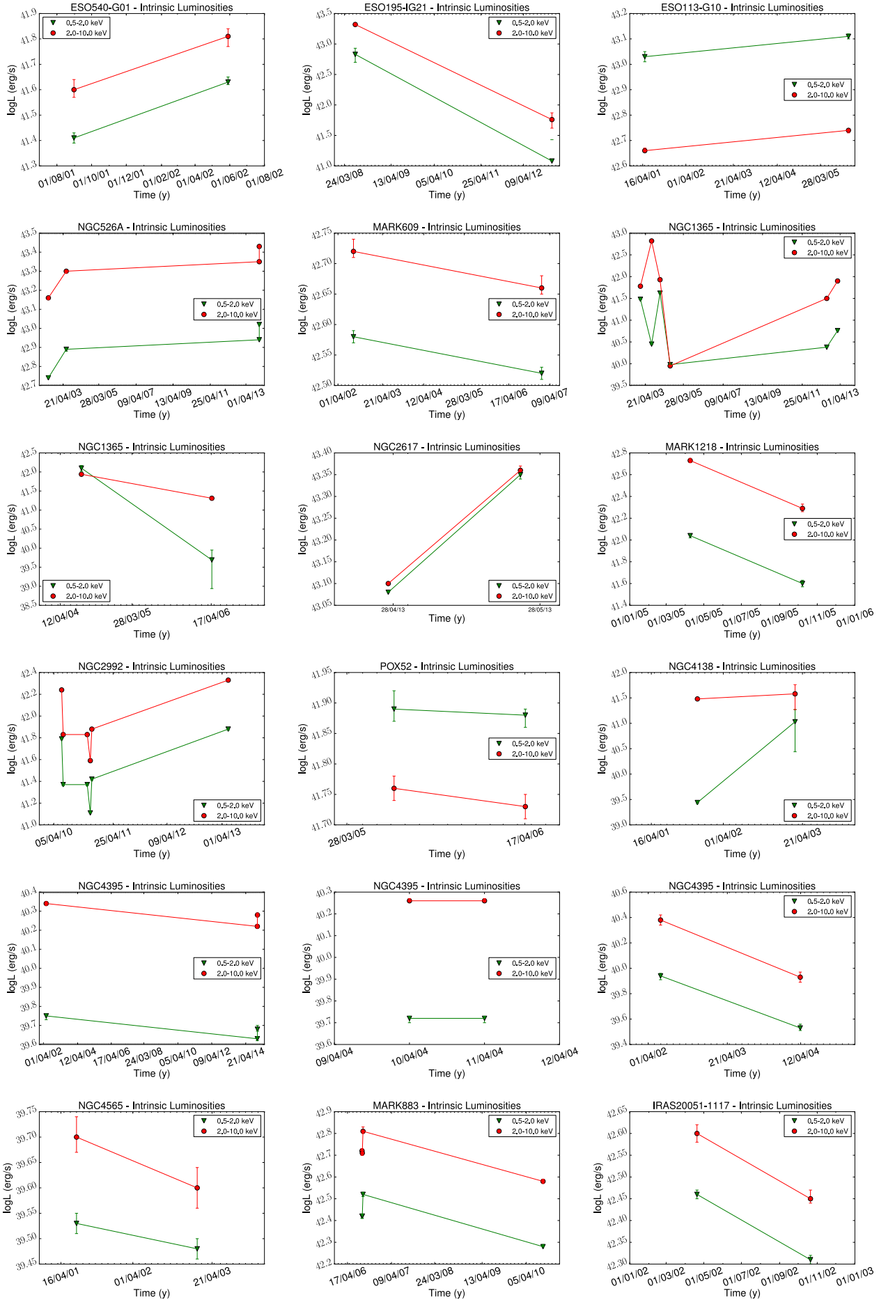
Page 24 of 55 Fig. 12: X-ray intrinsic luminosities calculated for the soft (0.5–2.0 keV, green triangles) and hard (2.0–10.0 keV, red circles) energies in the simultaneous fits, only for the variable objects
