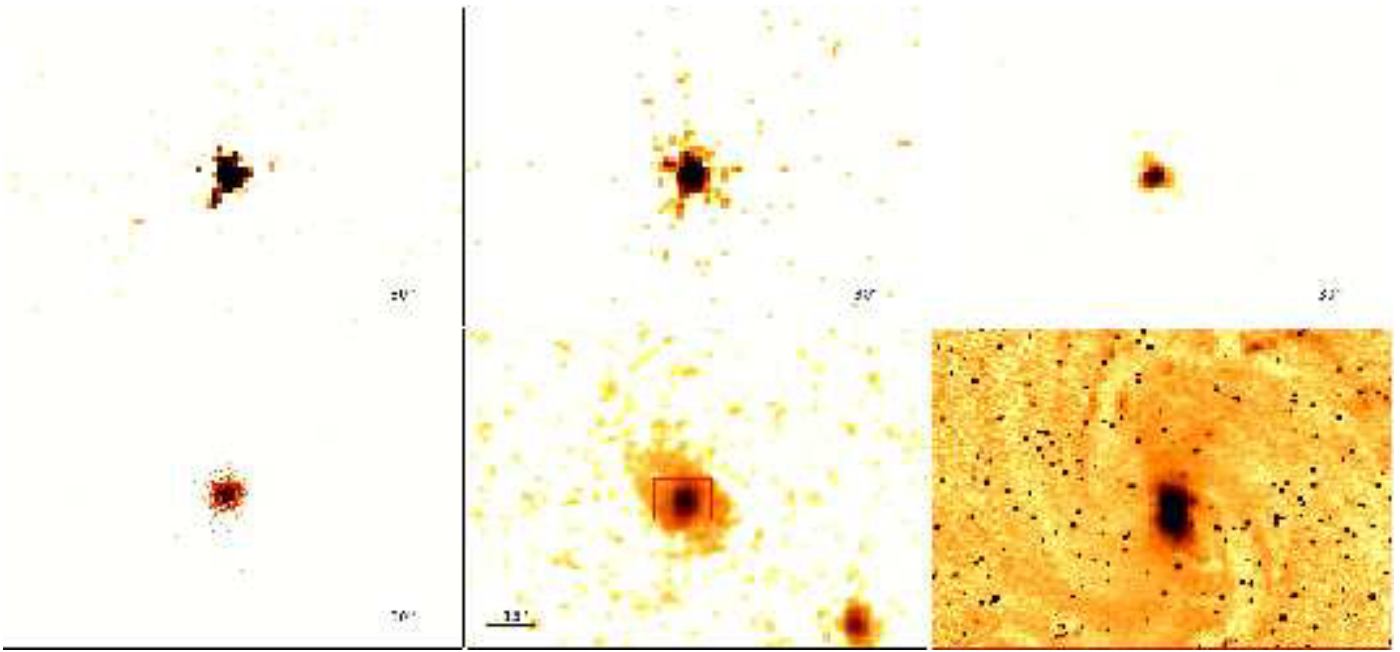
Fig. C.8: Images of M 82. (Top left): Smoothed X-ray 0.6-0.9 keV energy band; (top center): smoothed X-ray 1.6-2.0 keV energy band; (top right): smoothed X-ray 4.5-8.0 keV energy band; (bottom left): X-ray 0.5-10.0 keV energy band without smoothing; (bottom center): 2MASS image in the K_s band; (bottom right): Sharp divided Hubble image in the F606W filter.
