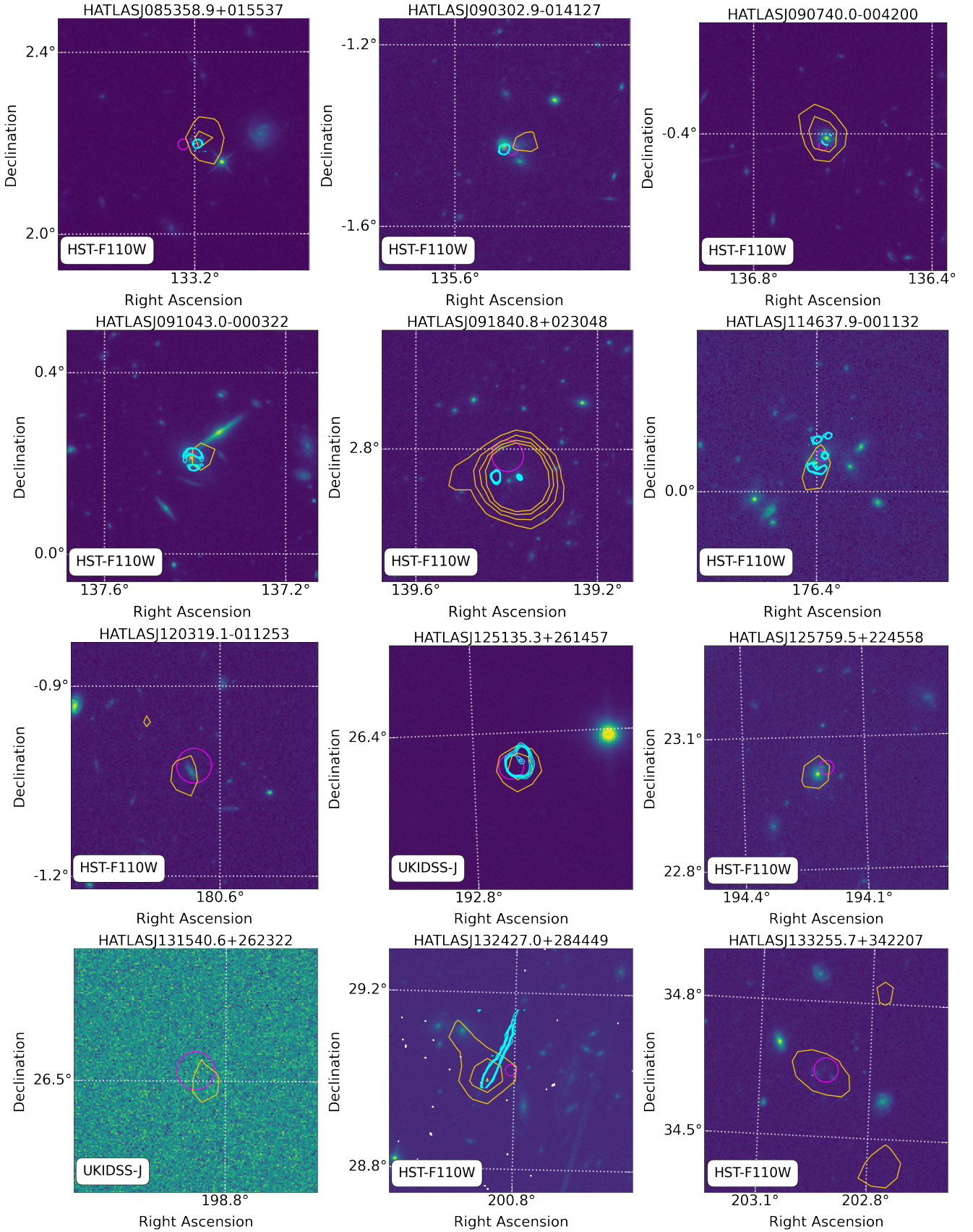
Figure 2. Cutouts of NIR images with the best available angular resolution centred on the Herschel positions for the 16 sources with a FIRST cross-match. Contours at 3,5,7,9 \sigma levels are shown in gold for FIRST and cyan for ALMA. Circles are the SPIRE position with a 3\sigma_{\text{pos}} radius. RA and Dec are reported in Deg units. The postage stamps are 30x30 arcsec.
