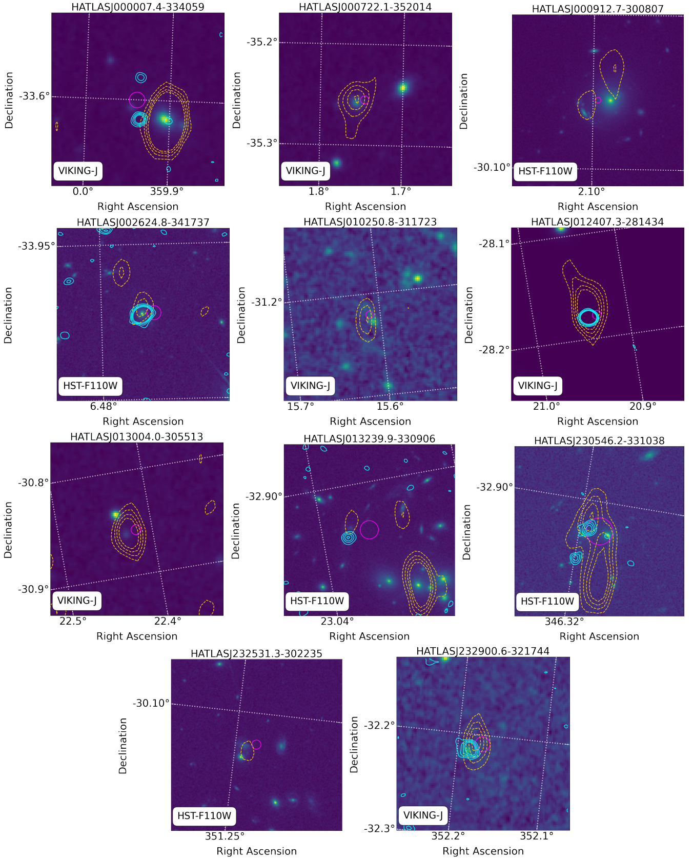
Figure 1. Cutouts of NIR images with the best available angular resolution centred on the Herschel positions for the 11 sources with an ATCA cross-match. Contours at 3, 5, 7, 9\sigma levels are shown in gold for the radio and cyan for ALMA. Circles are the SPIRE position with a 3\sigma_{\text{pos}} radius. RA and Dec are reported in Deg units. The postage stamps are 30x30 arcsec
