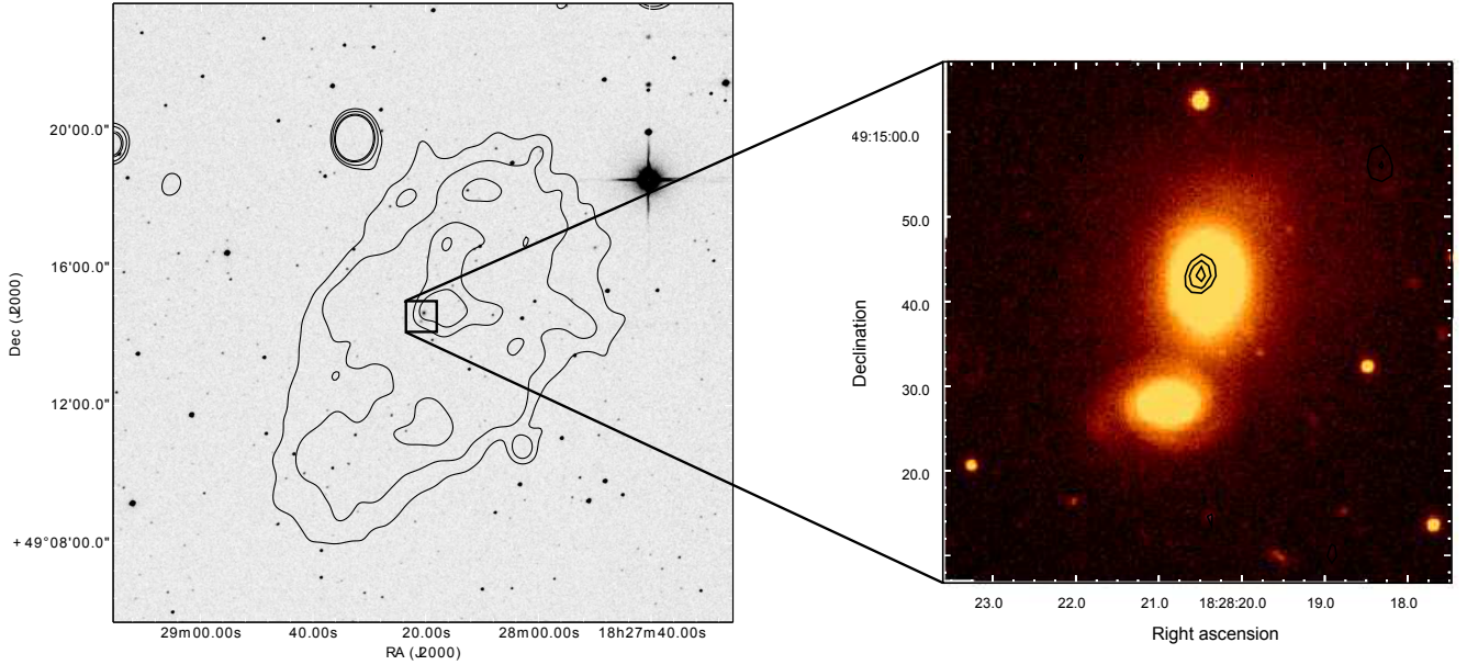
Fig. 2. Left – blob1 contours from the 1.4 GHz WSRT map (levels 3, 6, 12, and 15 \sigma ) overlaid on the 2MASS K_s -band image of the field; right – Zoom-in on the host galaxy and on the companion galaxy from the r -band image contours from the 5 GHz WSRT map in black (levels 3, 5, and 7 \times \sigma (0.085 mJy beam -1 )).
